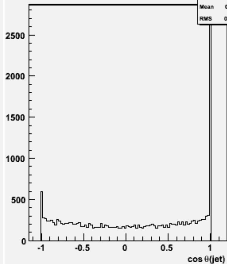
cos \theta for 2-jets :w104526 e2e2h_o
