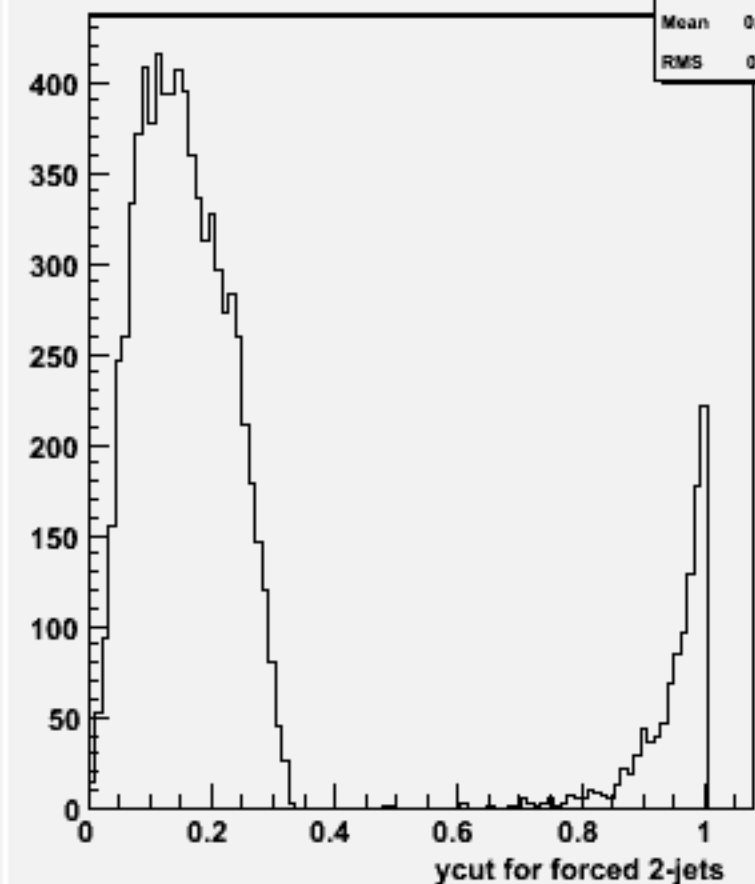
Ycut for 2-jets :w104526 e2e2h_o
