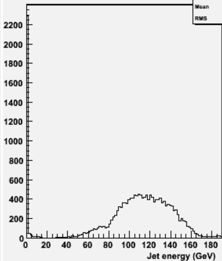
energy for 2-jets :w104526 e2e2h_o
