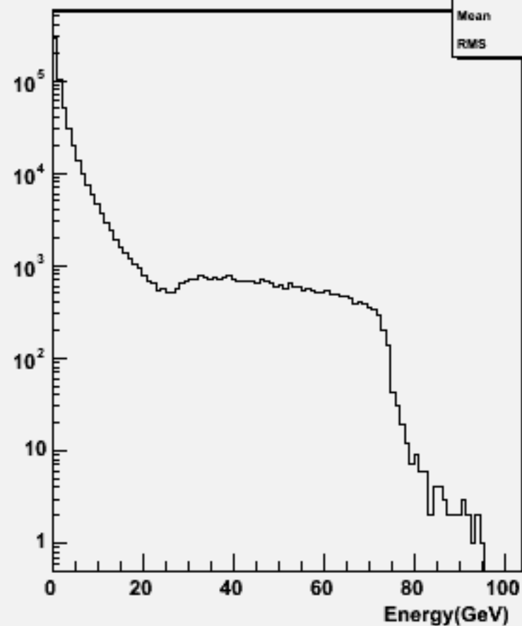
Particle Energy : w104526 e2e2h_o
