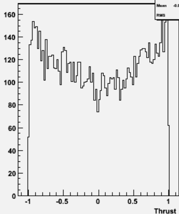
cos \Theta (thrust) w104526 e2e2h_o
