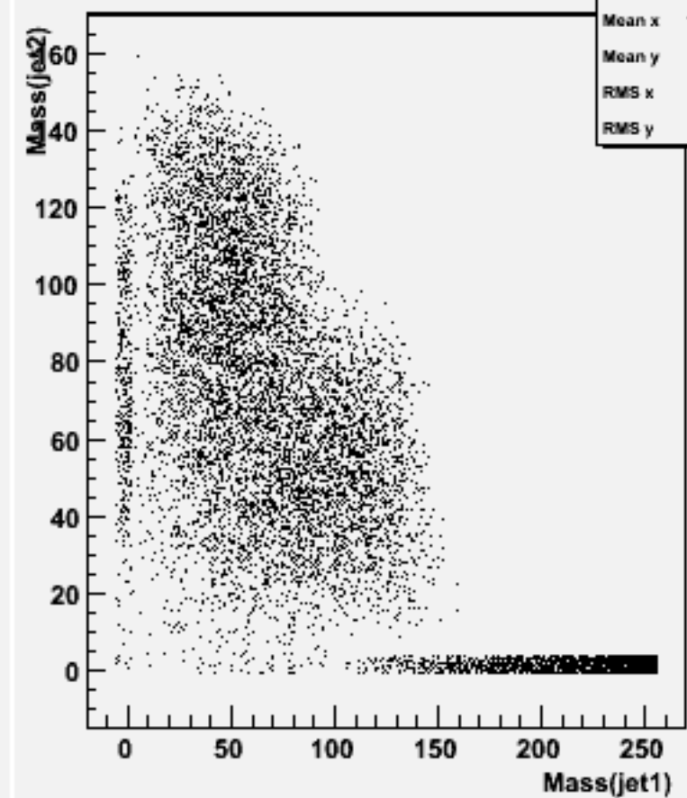
Jet mass for forced 2-jets : w104526 e2e2h_o
