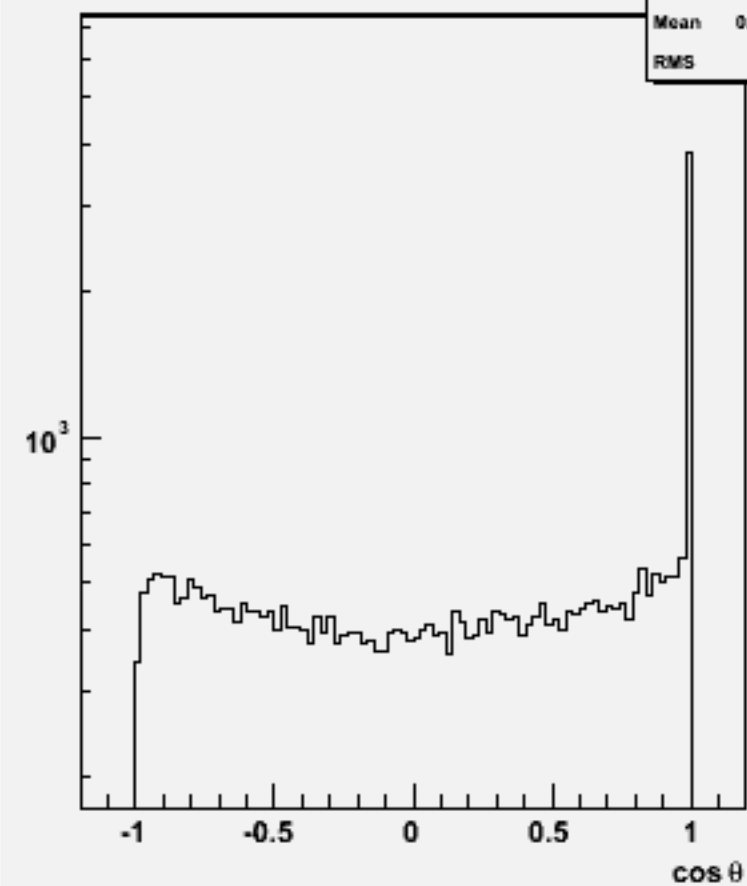
Jet cos \theta (All jets)w104526 e2e2h_o
