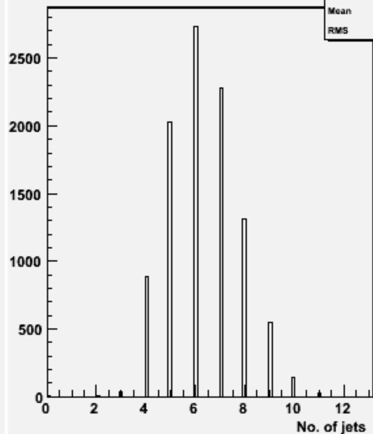
No. jets (ycut=0.001) : w104526 e2e2h_o
