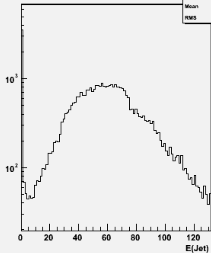
Jet energies(All jets)w104526 e2e2h_o
