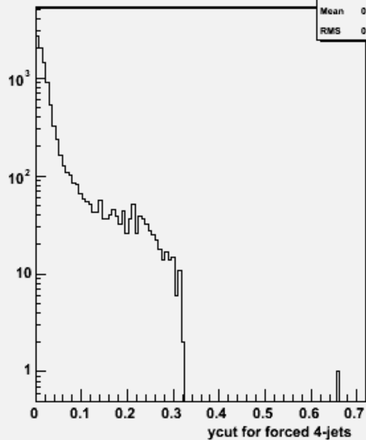
Ycut for 4-jets :w104526 e2e2h_o
