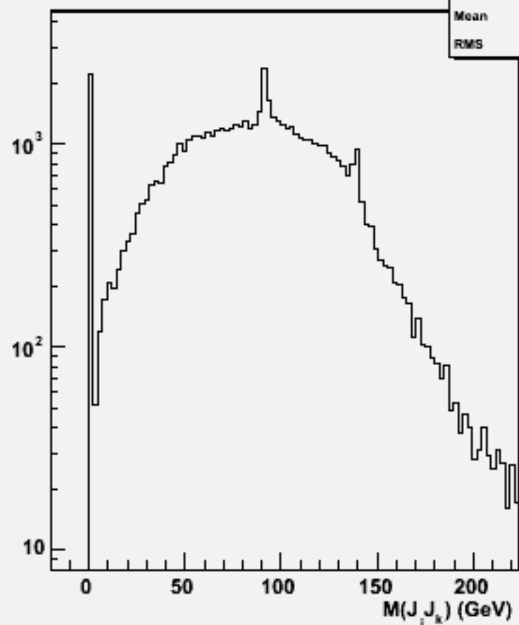
2jets mass(All comb)w104526 e2e2h_o
