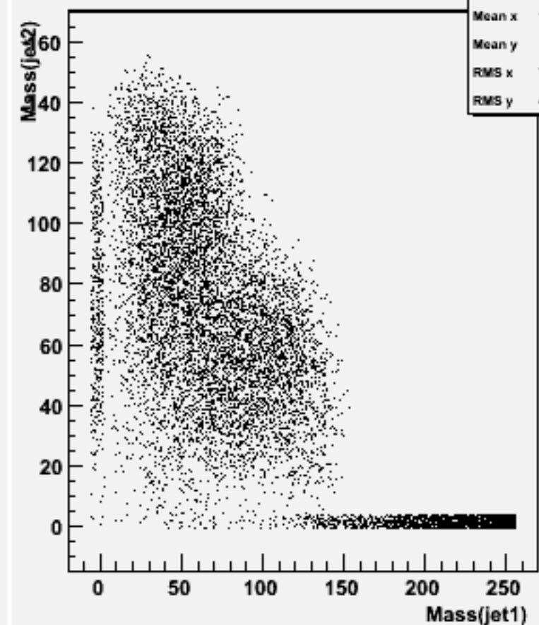
Jet mass for forced 2-jets : w104525 e2e2h_o
