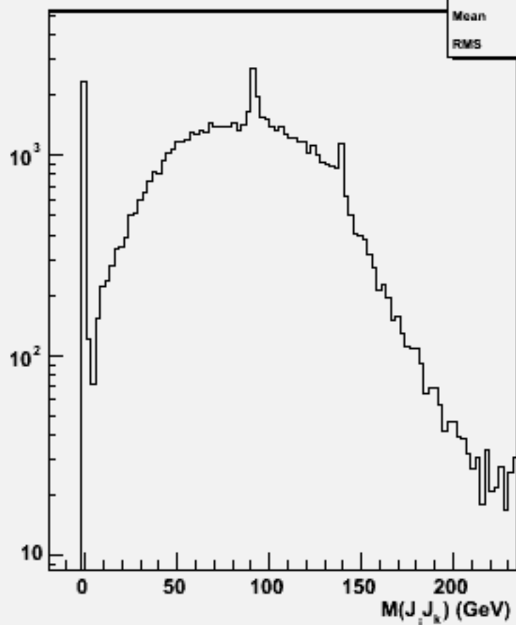
2jets mass(All comb)w104525 e2e2h_o
