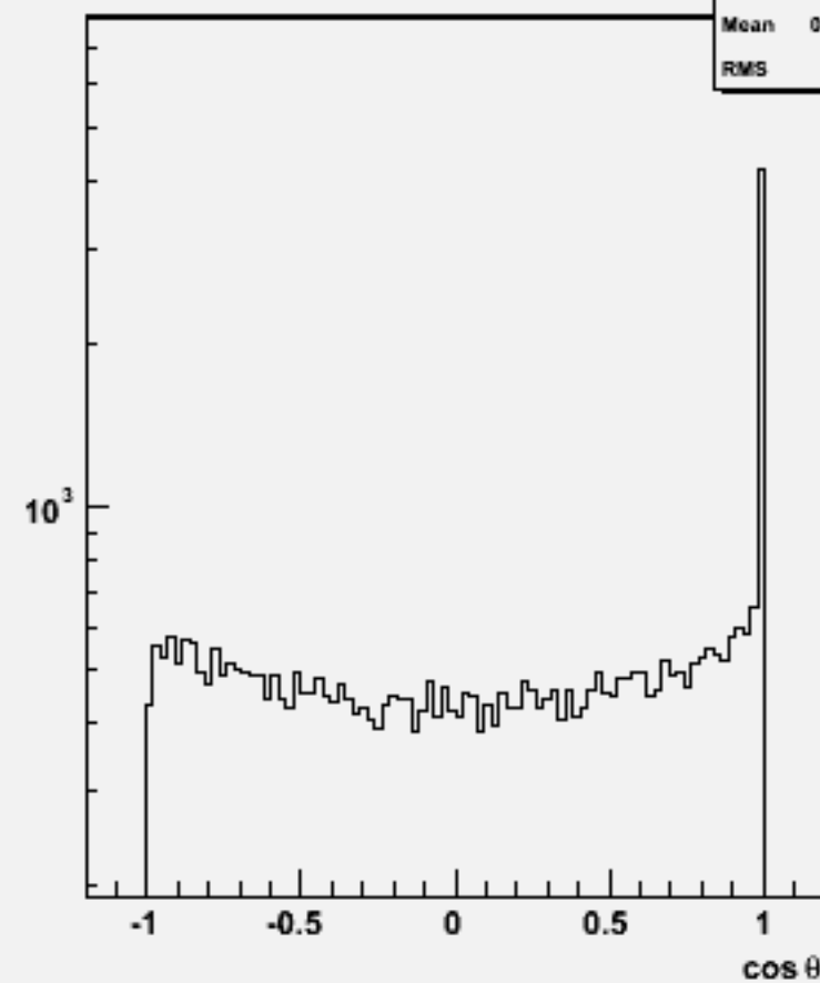
Jet cos \theta (All jets)w104525 e2e2h_o
