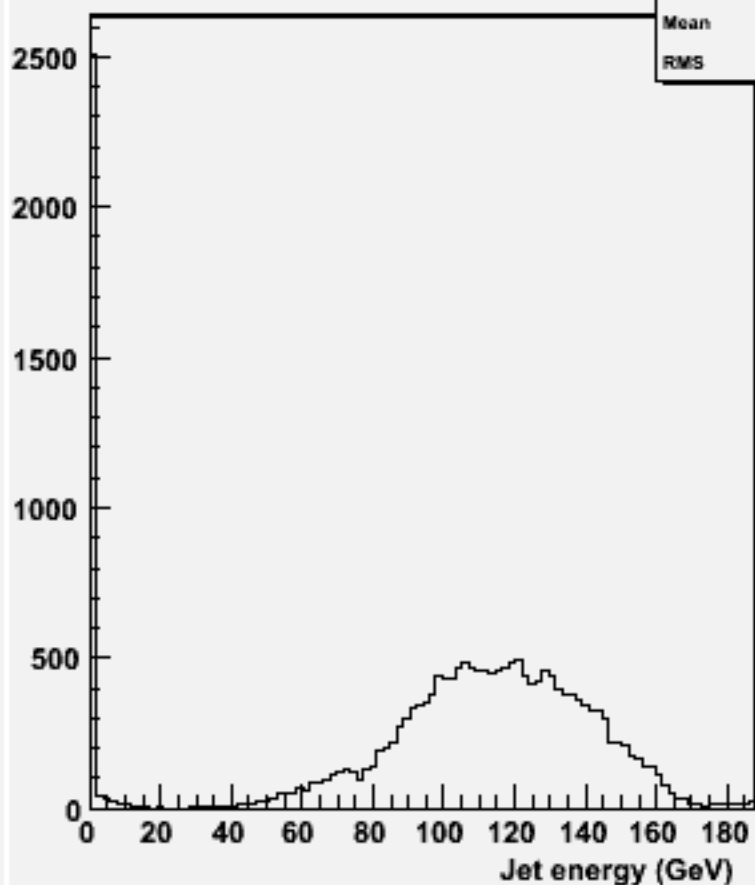
energy for 2-jets :w104525 e2e2h_o
