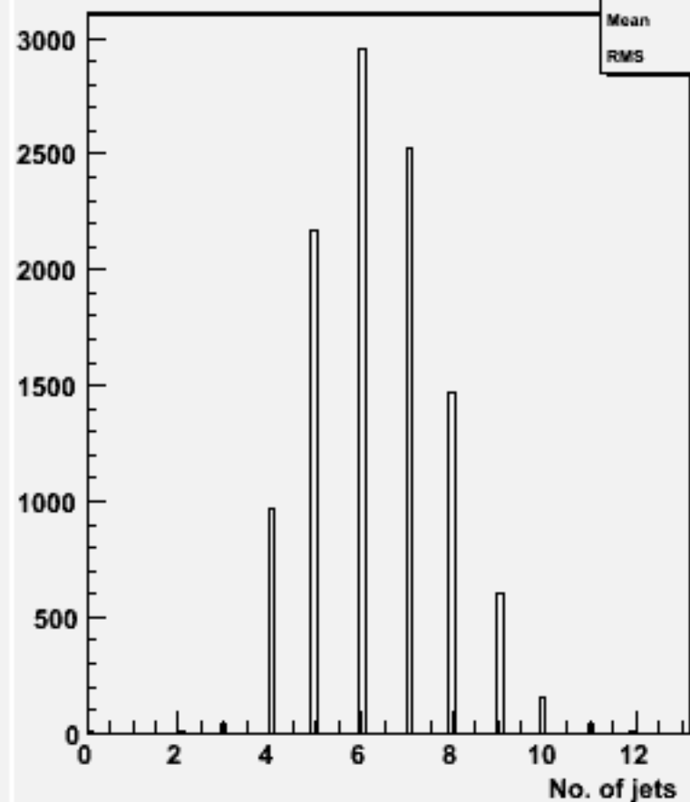
No. jets (ycut=0.001) : w104525 e2e2h_o
