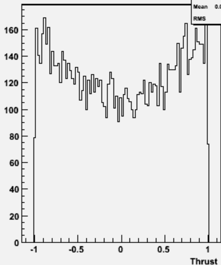
cos \Theta (thrust) w104525 e2e2h_o
