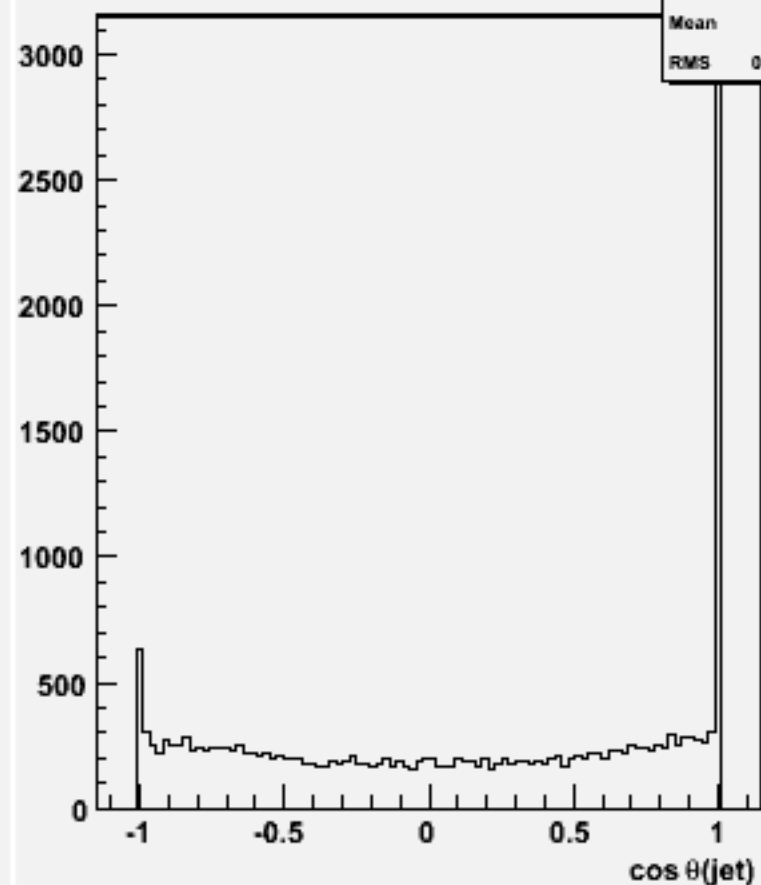
cos \theta for 2-jets :w104525 e2e2h_o
