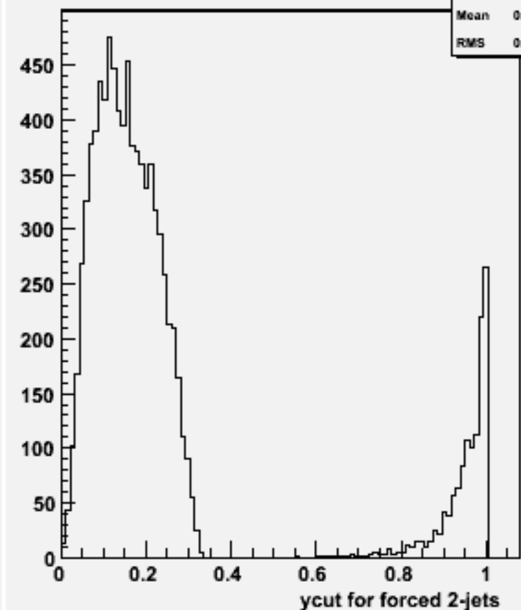
Ycut for 2-jets :w104525 e2e2h_o
