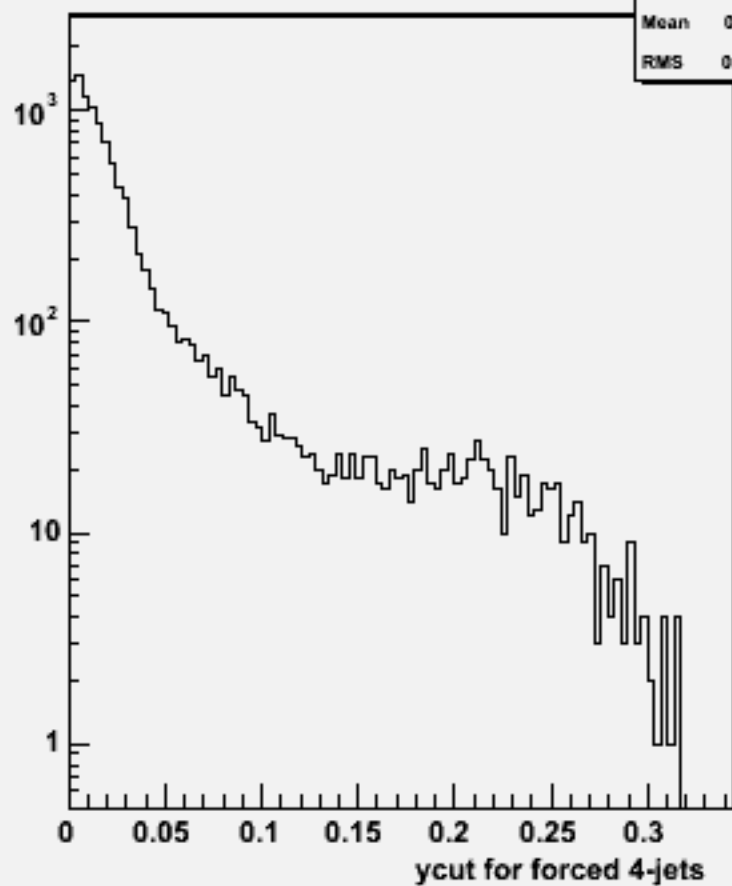
Ycut for 4-jets :w104525 e2e2h_o
