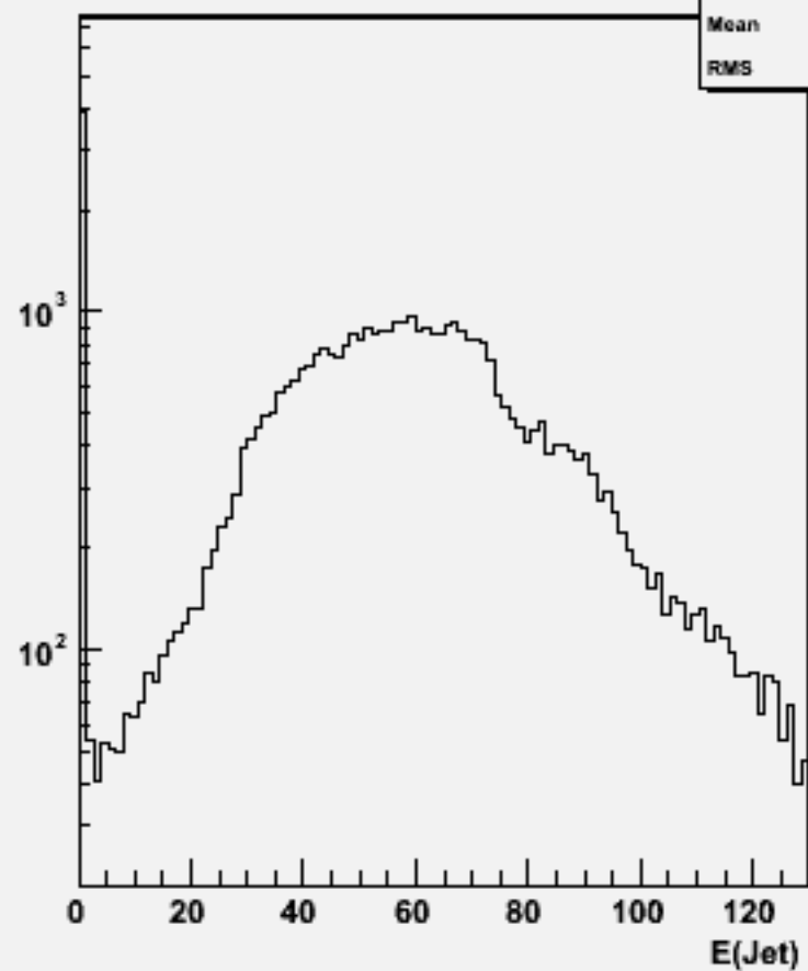
Jet energies(All jets)w104525 e2e2h_o
