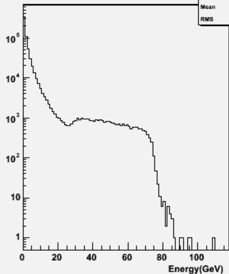
Particle Energy : w104525 e2e2h_o
