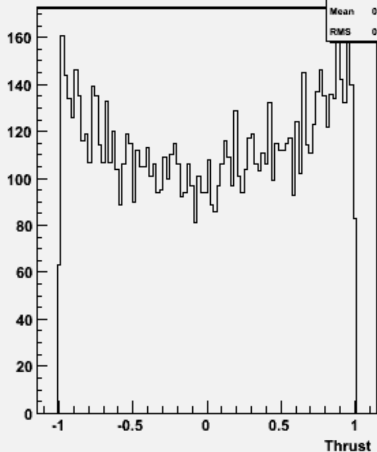
cos \theta (thrust) w104522 e1e1h_o
