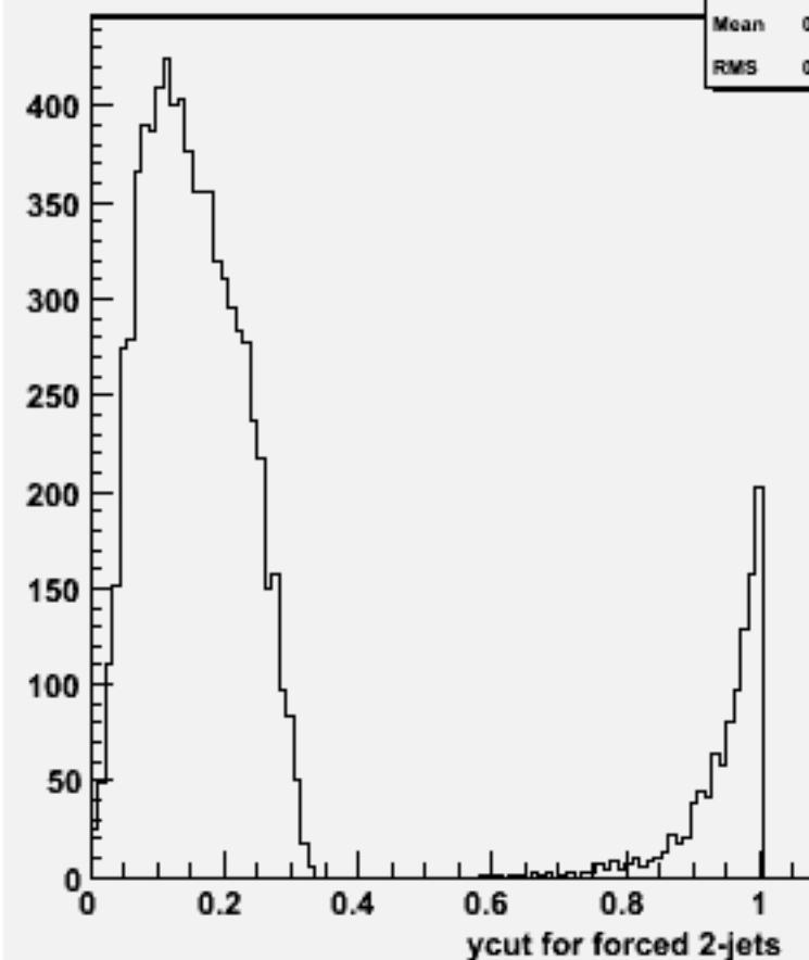
Ycut for 2-jets :w104522 e1e1h_o
