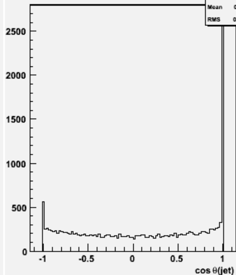
cos \theta for 2-jets :w104522 e1e1h_o
