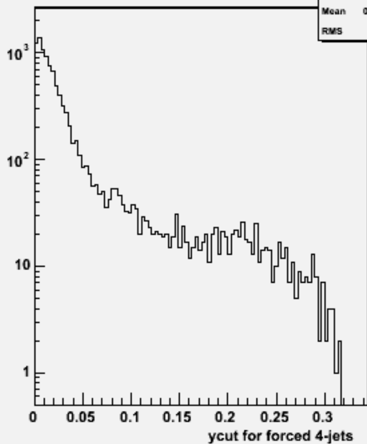
Ycut for 4-jets :w104522 e1e1h_o
