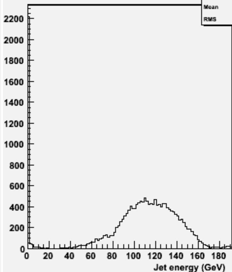
energy for 2-jets :w104522 e1e1h_o
