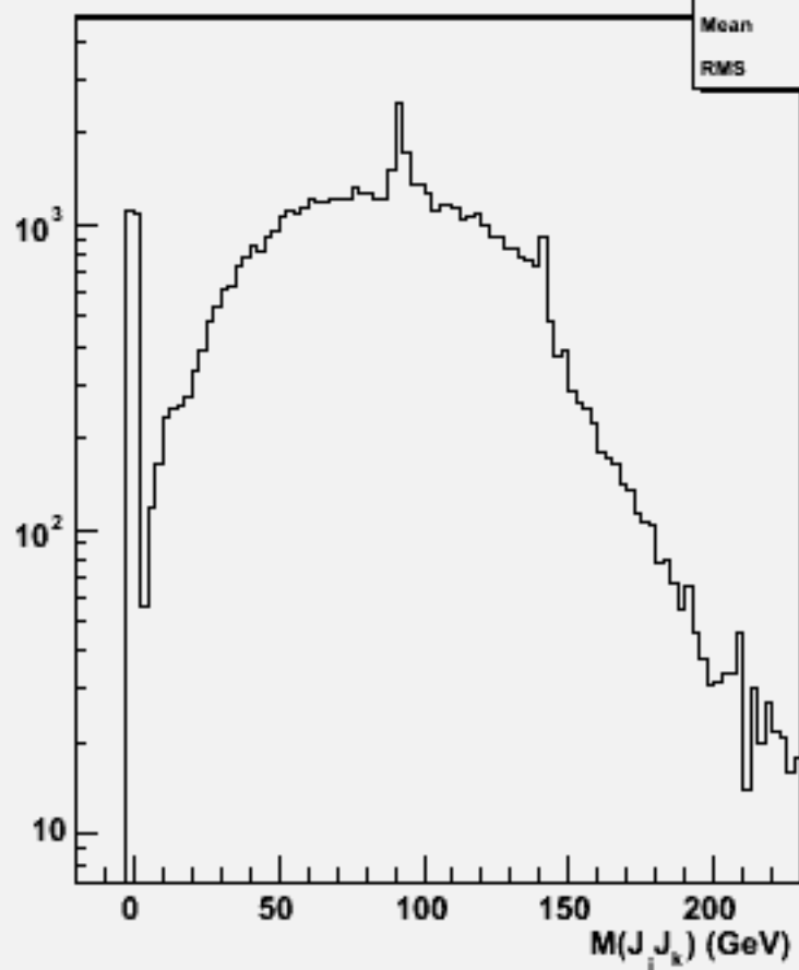
2jets mass(All comb)w104522 e1e1h_o
