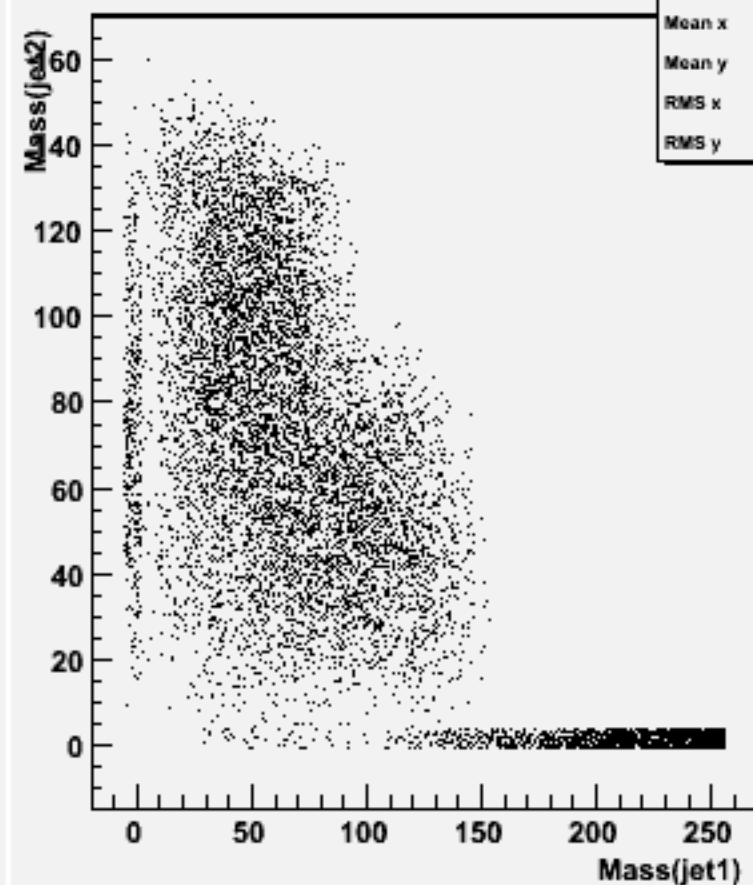
Jet mass for forced 2-jets : w104522 e1e1h_o
