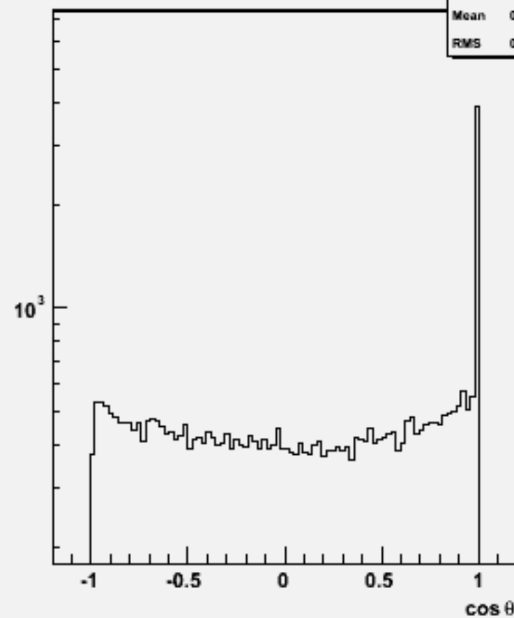
Jet cos \theta (All jets)w104522 e1e1h_o
