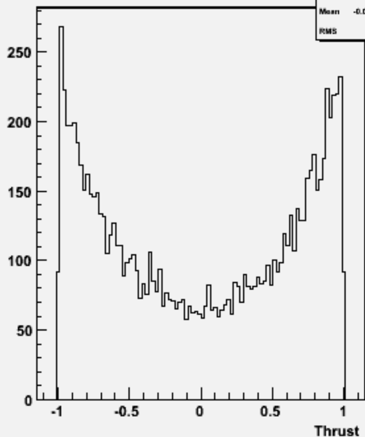
cos \Theta (thrust) w104520 e1e1h_o
