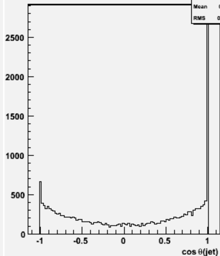
cos \theta for 2-jets :w104520 e1e1h_o
