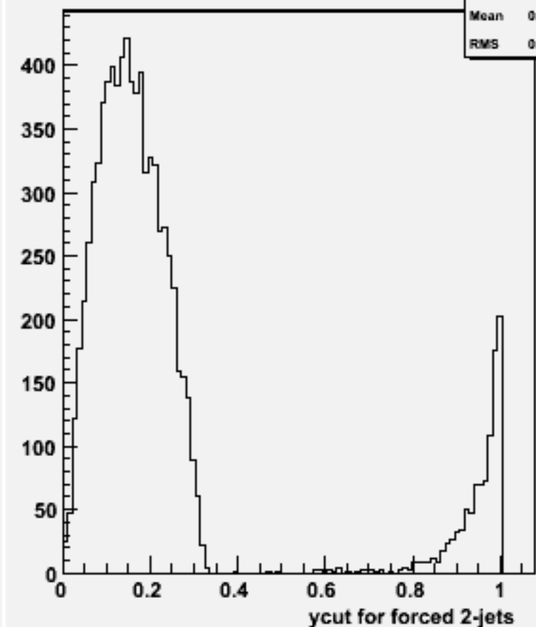
Ycut for 2-jets :w104520 e1e1h_o
