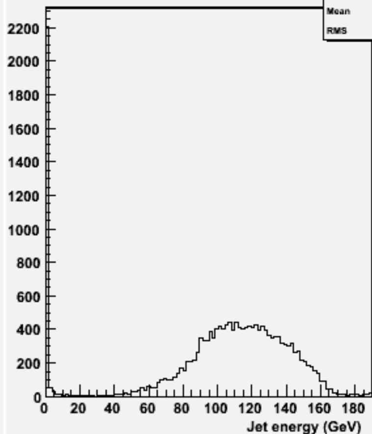
energy for 2-jets :w104520 e1e1h_o
