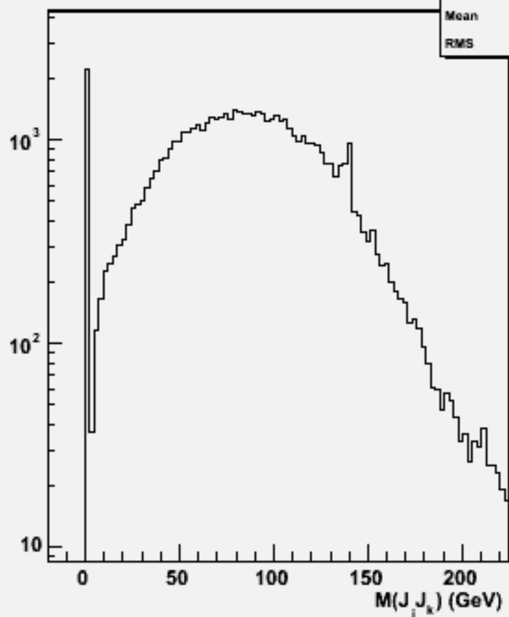
2jets mass(All comb)w104520 e1e1h_o
