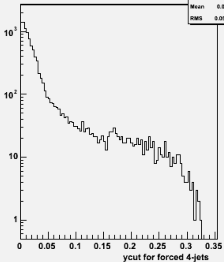
Ycut for 4-jets :w104520 e1e1h_o
