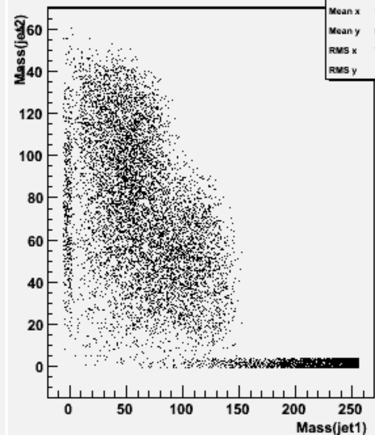
Jet mass for forced 2-jets : w104520 e1e1h_o
