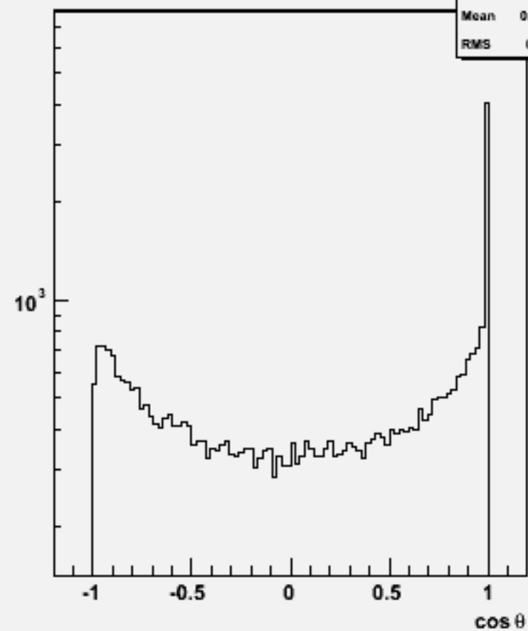
Jet cos \theta (All jets)w104520 e1e1h_o
