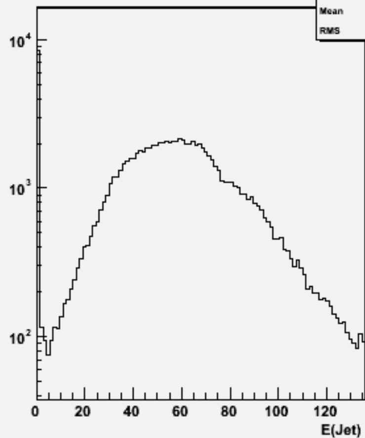
Jet energies(All jets)w104518 cch_o
