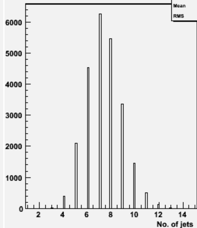
No. jets (ycut=0.001) : w104518 cch_o
