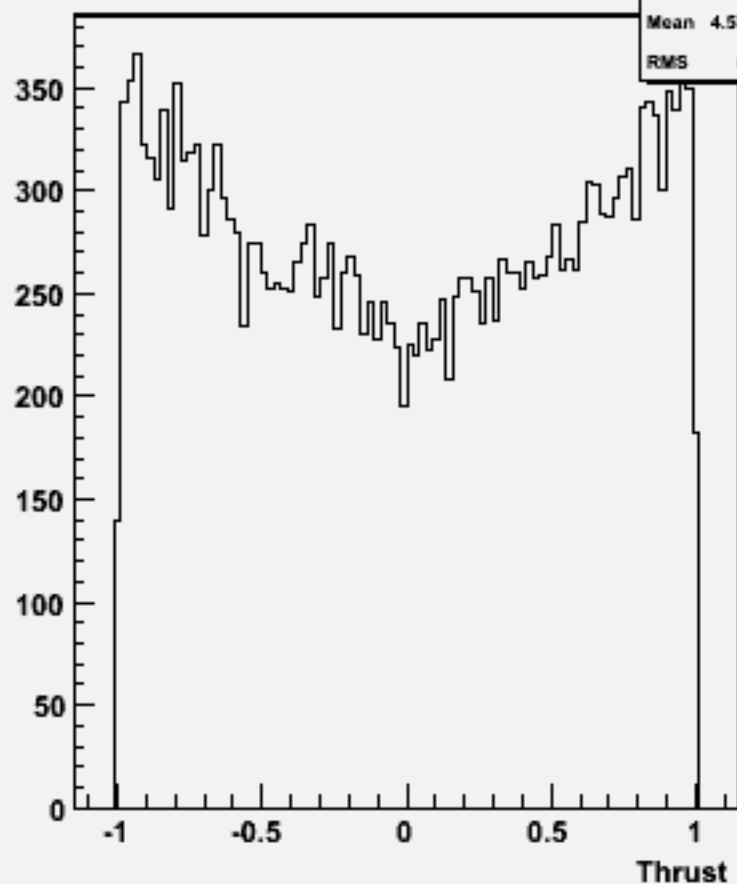
cos \Theta (thrust) w104518 cch_o
