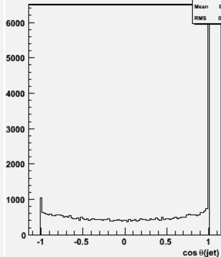
cos \Theta for 2-jets :w104518 cch_o
