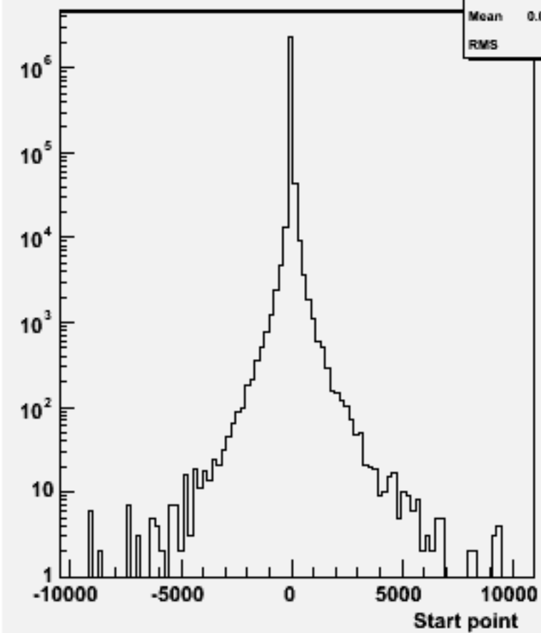
Start point Z : w104518 cch_o
