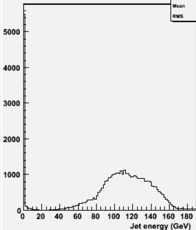
energy for 2-jets :w104518 cch_o
