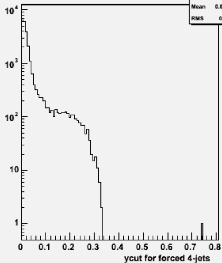
Ycut for 4-jets :w104518 cch_o
