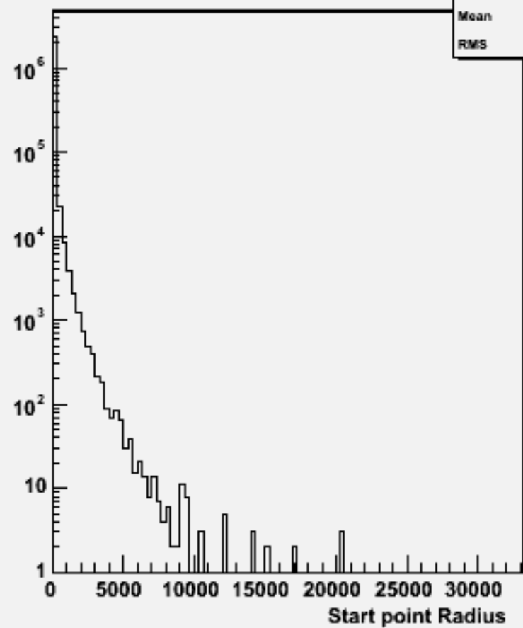
Start point R : w104518 cch_o
