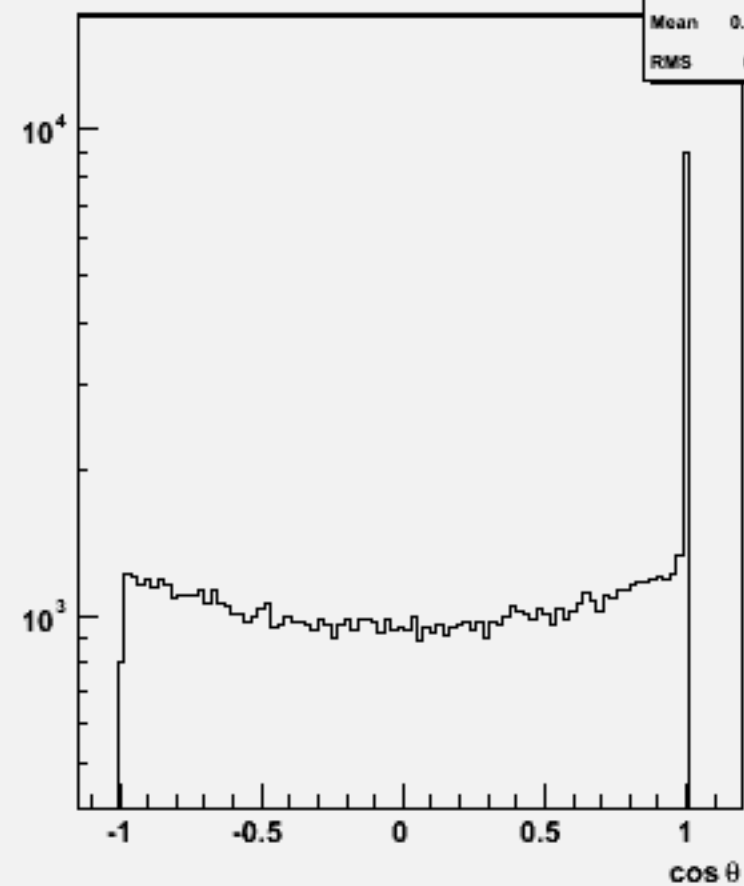
Jet cosθ (All jets)w104518 cch_o
