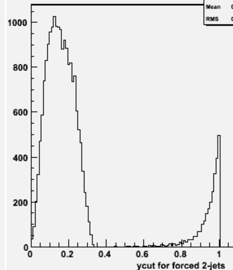
Ycut for 2-jets :w104518 cch_o
