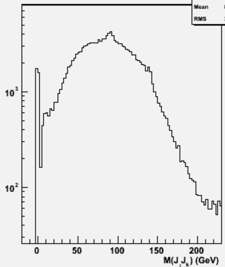
2jets mass(All comb)w104518 cch_o
