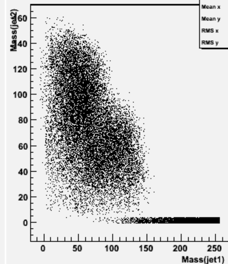
Jet mass for forced 2-jets : w104518 cch_o
