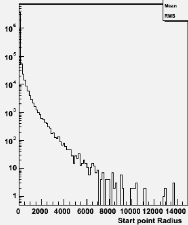
Start point R : w104517 cch_o
