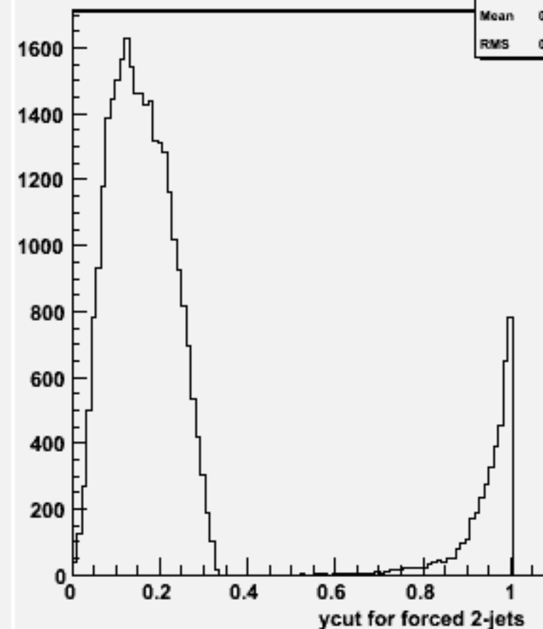
Ycut for 2-jets :w104517 cch_o
