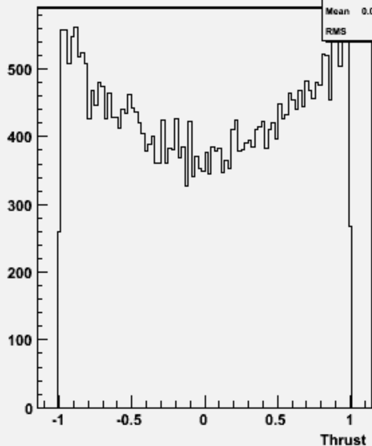
cos \Theta (thrust) w104517 cch_o
