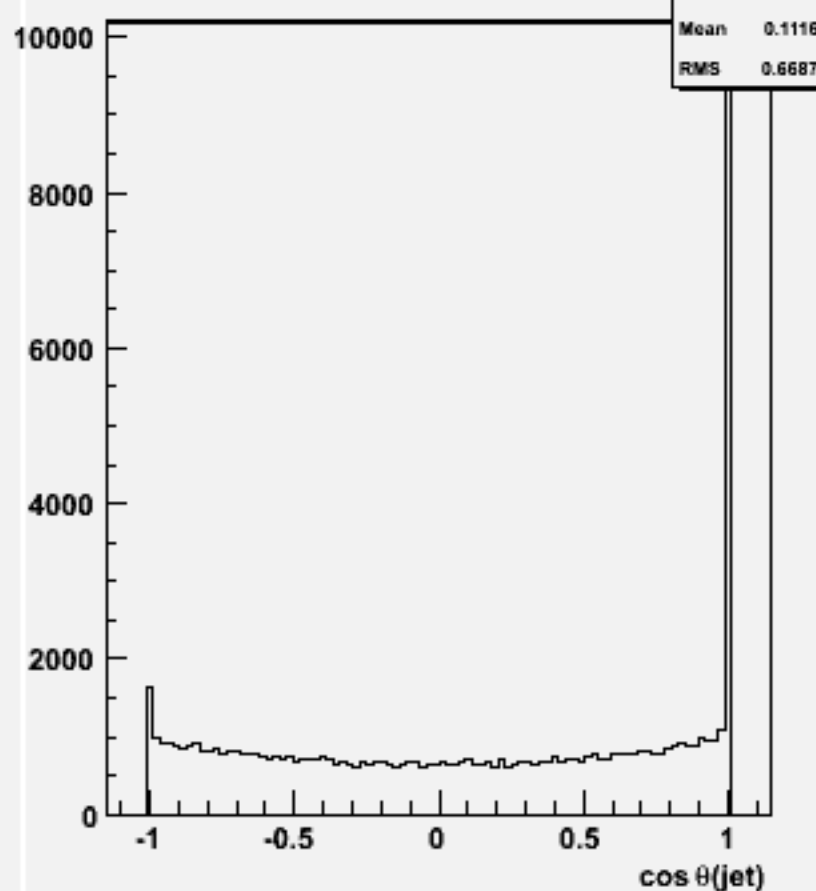
cos \theta for 2-jets :w104517 cch_o
