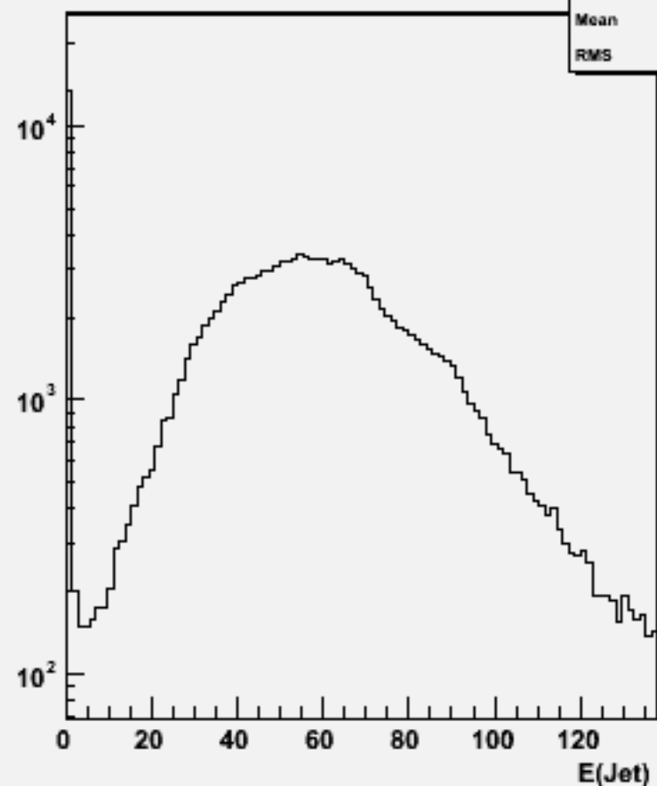
Jet energies(All jets)w104517 cch_o
