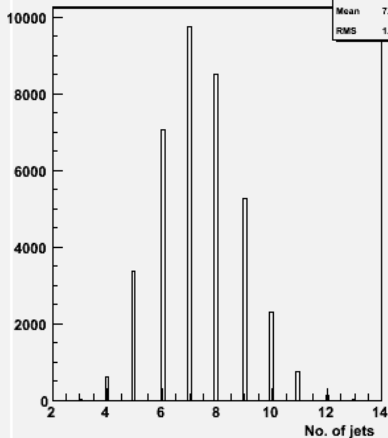
No. jets (ycut=0.001) : w104517 cch_o
