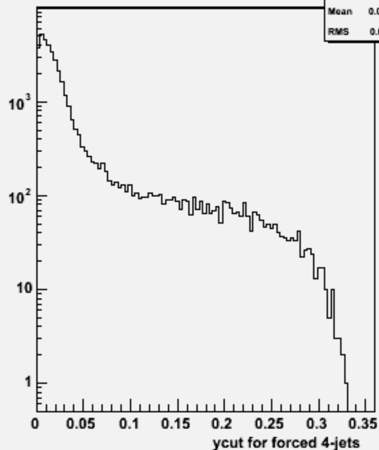
Ycut for 4-jets :w104517 cch_o
