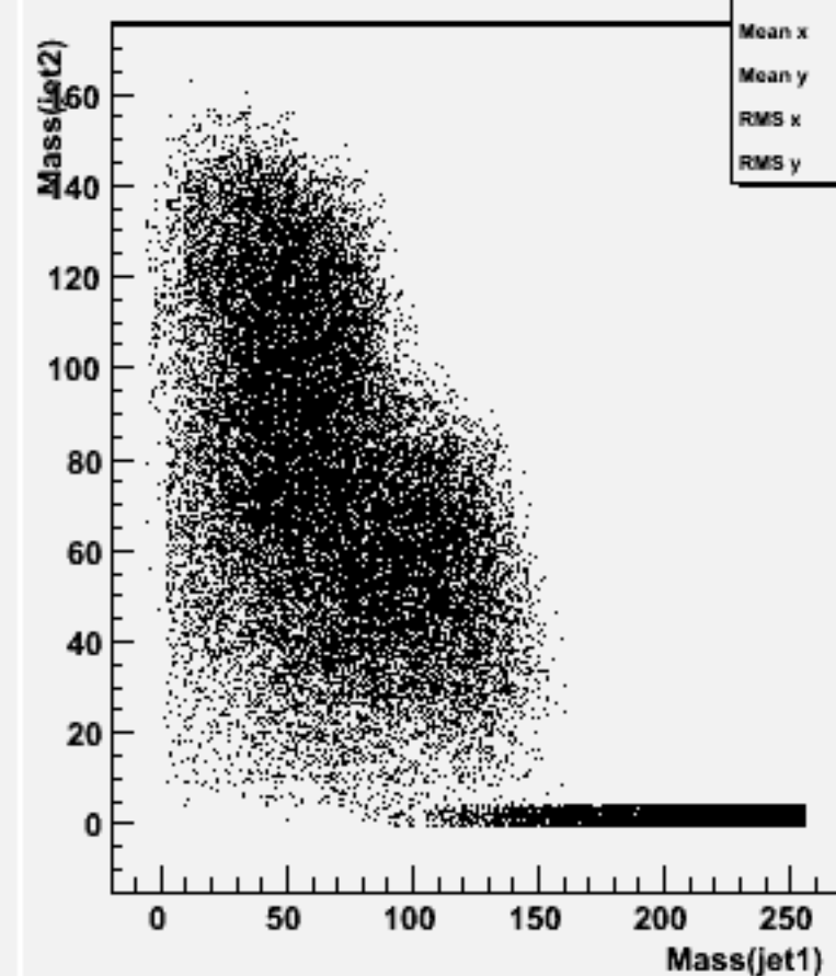
Jet mass for forced 2-jets : w104517 cch_o
