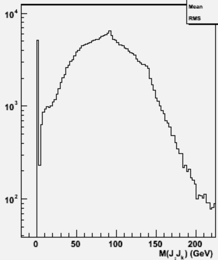
2jets mass(All comb)w104517 cch_o
