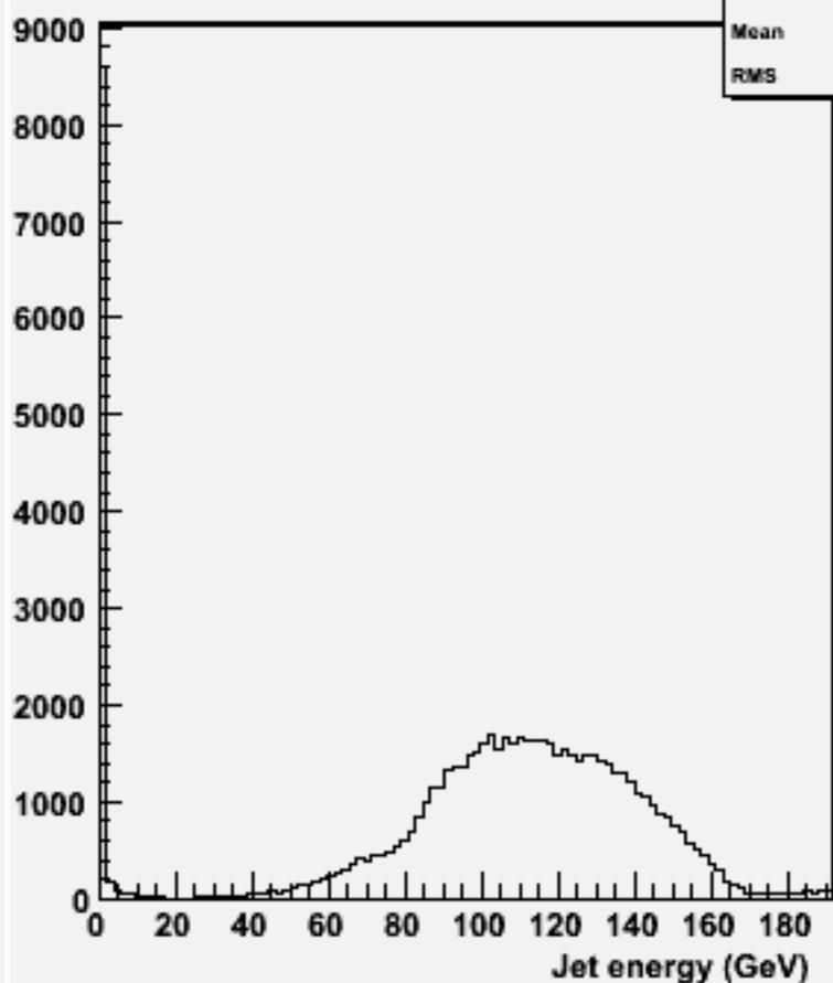
energy for 2-jets :w104517 cch_o
