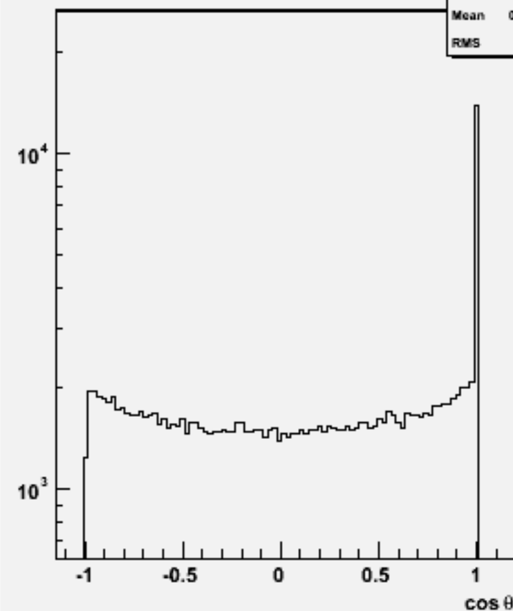
Jet cos \theta (All jets)w104517 cch_o
