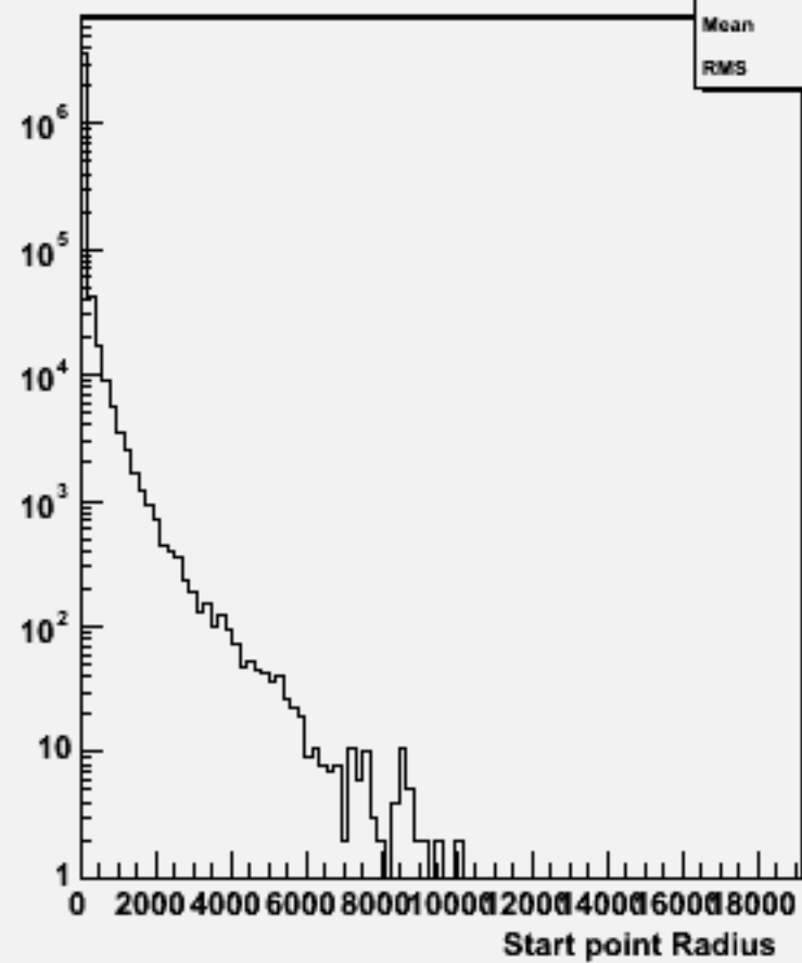
Start point R : w104513 uuh_o
