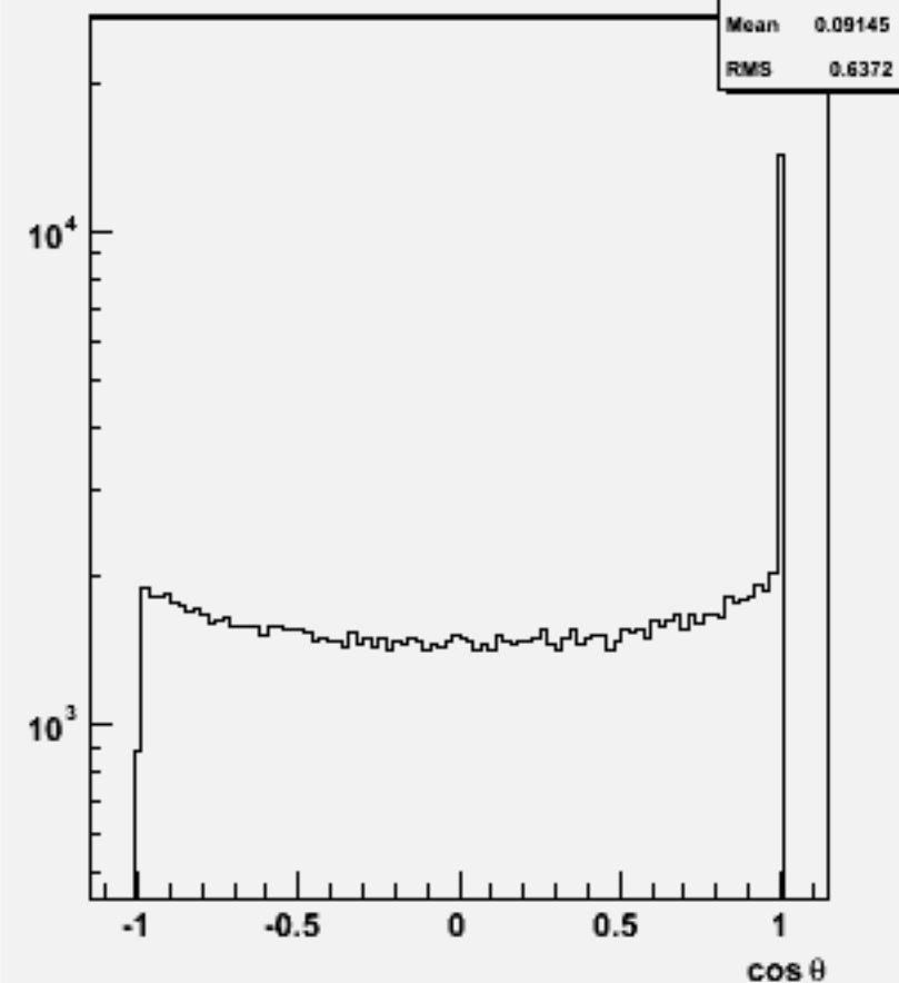
Jet cos \theta (All jets)w104513 uuh_o
