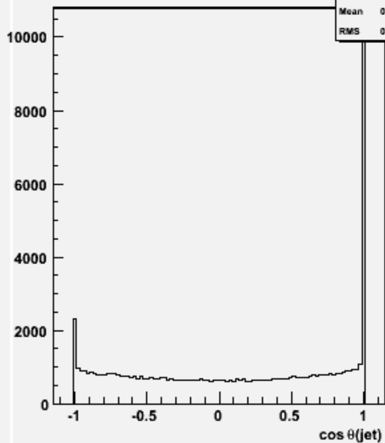
cos \theta for 2-jets :w104513 uuh_o
