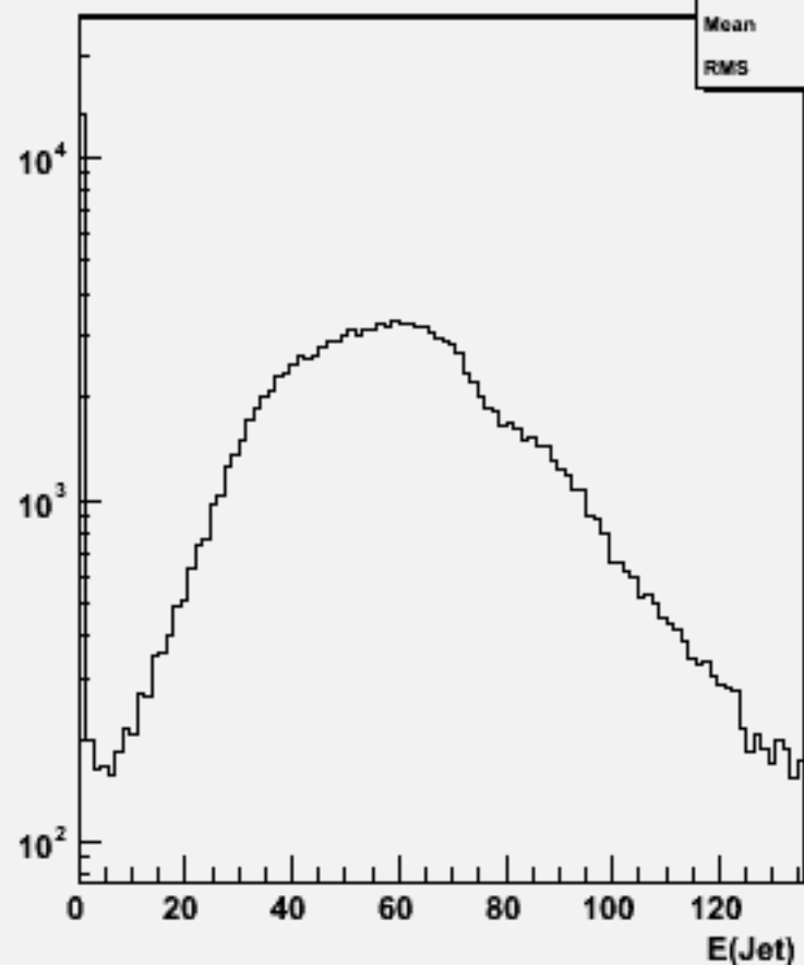
Jet energies(All jets)w104513 uuh_o
