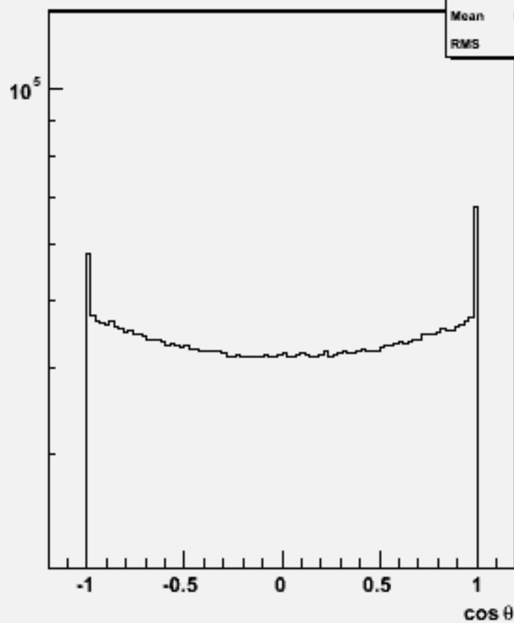
Particle \cos\theta : w104513 uuh_o
