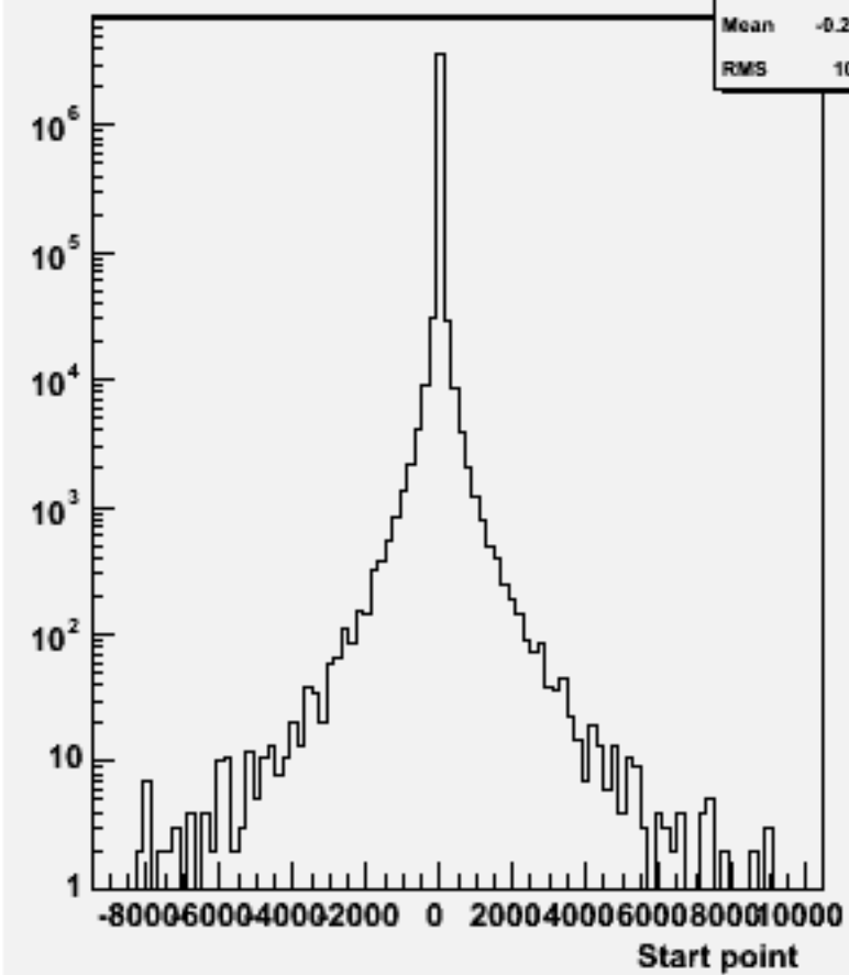
Start point Z : w104513 uuh_o
