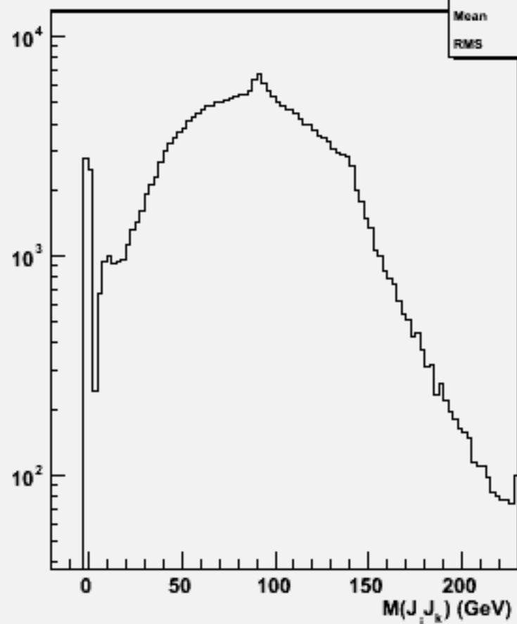
2jets mass(All comb)w104513 uuh_o
