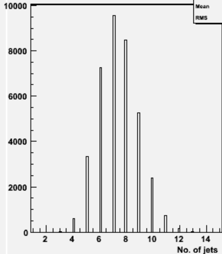
No. jets (ycut=0.001) : w104513 uuh_o
