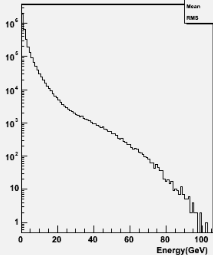
Particle Energy : w104513 uuh_o
