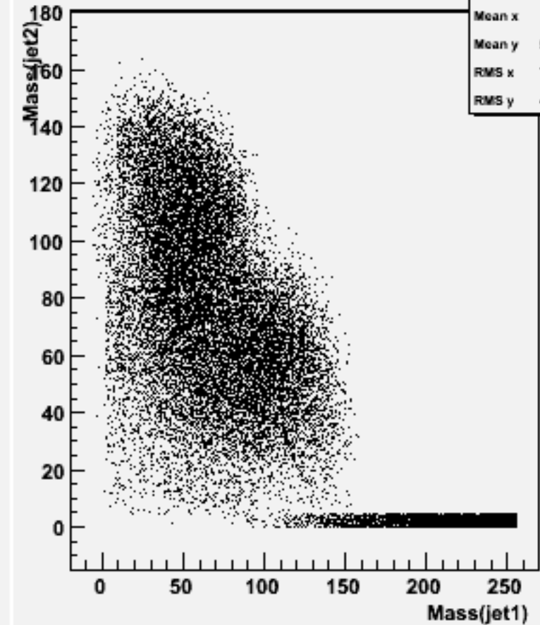
Jet mass for forced 2-jets : w104513 uuh_o
