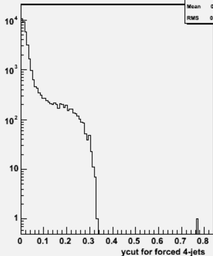
Ycut for 4-jets :w104513 uuh_o
