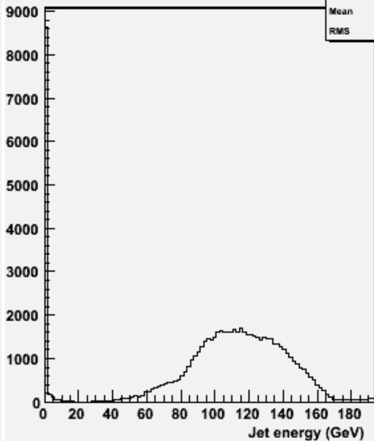
energy for 2-jets :w104513 uuh_o
