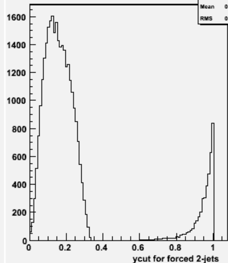
Ycut for 2-jets :w104513 uuh_o
