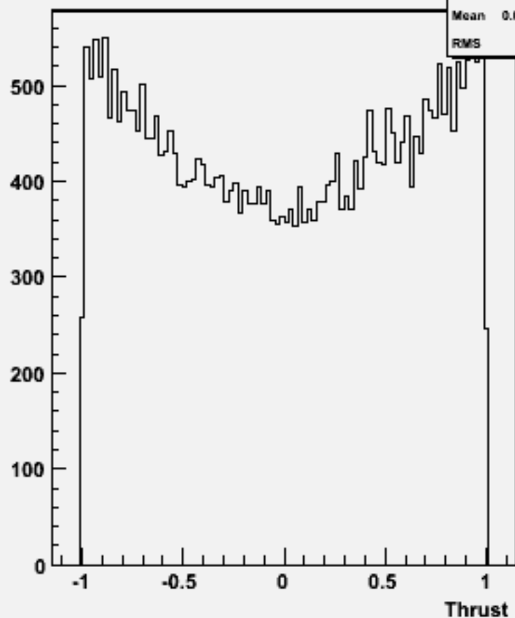
cos \Theta (thrust) w104513 uuh_o
