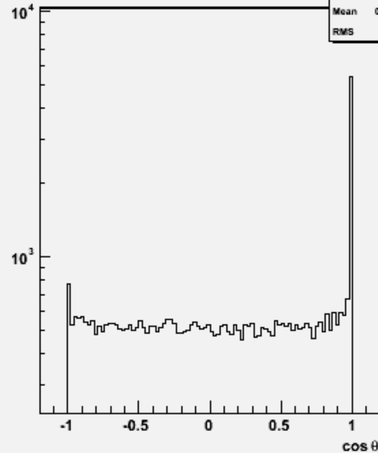
Jet cosθ (All jets)w104510 n3n3h_o
