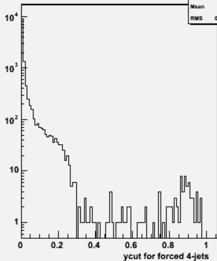
Ycut for 4-jets :w104510 n3n3h_o
