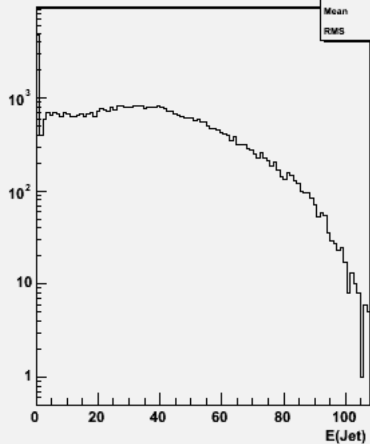
Jet energies(All jets)w104510 n3n3h_o
