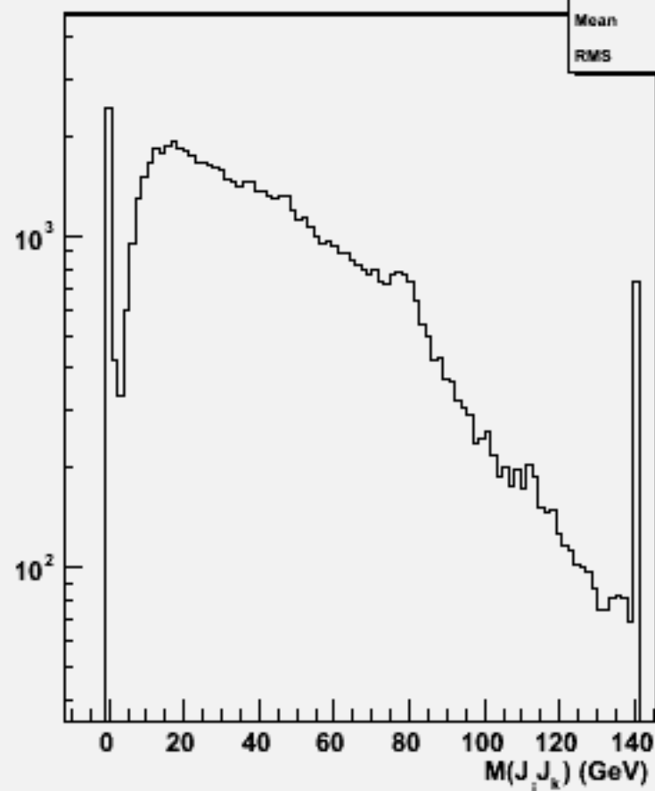
2jets mass(All comb)w104510 n3n3h_o
