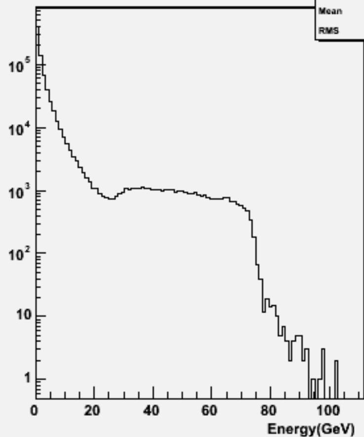
Particle Energy : w104510 n3n3h_o
