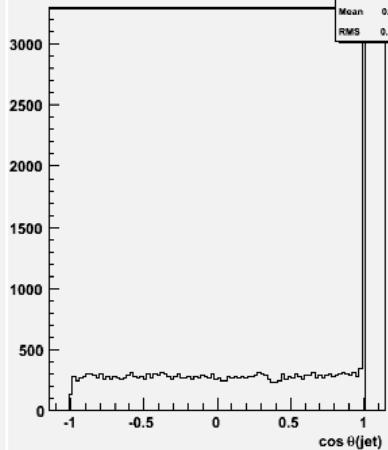
cos \theta for 2-jets :w104510 n3n3h_o
