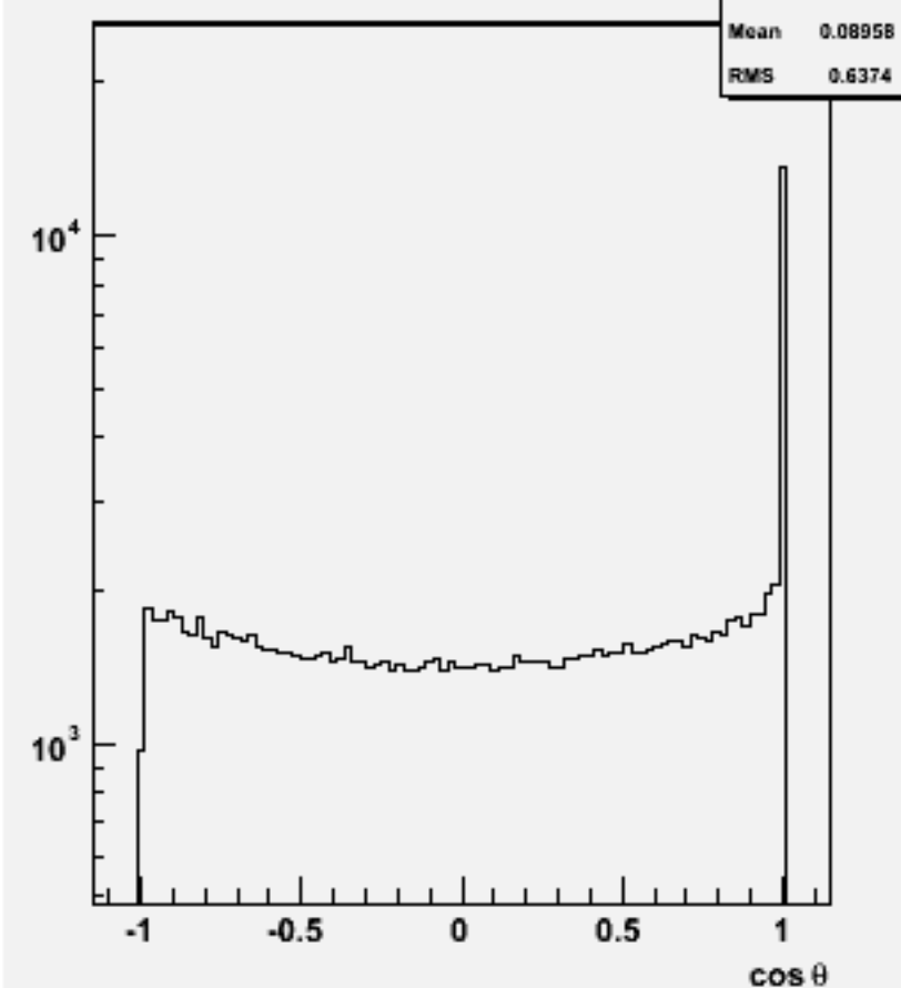
Jet cos \theta (All jets)w104492 bbh_o
