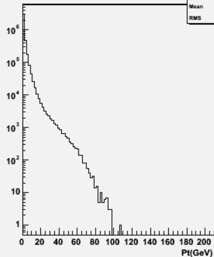
Particle Pt : w104492 bbh_o
