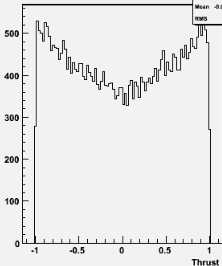
cos \Theta (thrust) w104492 bbh_o
