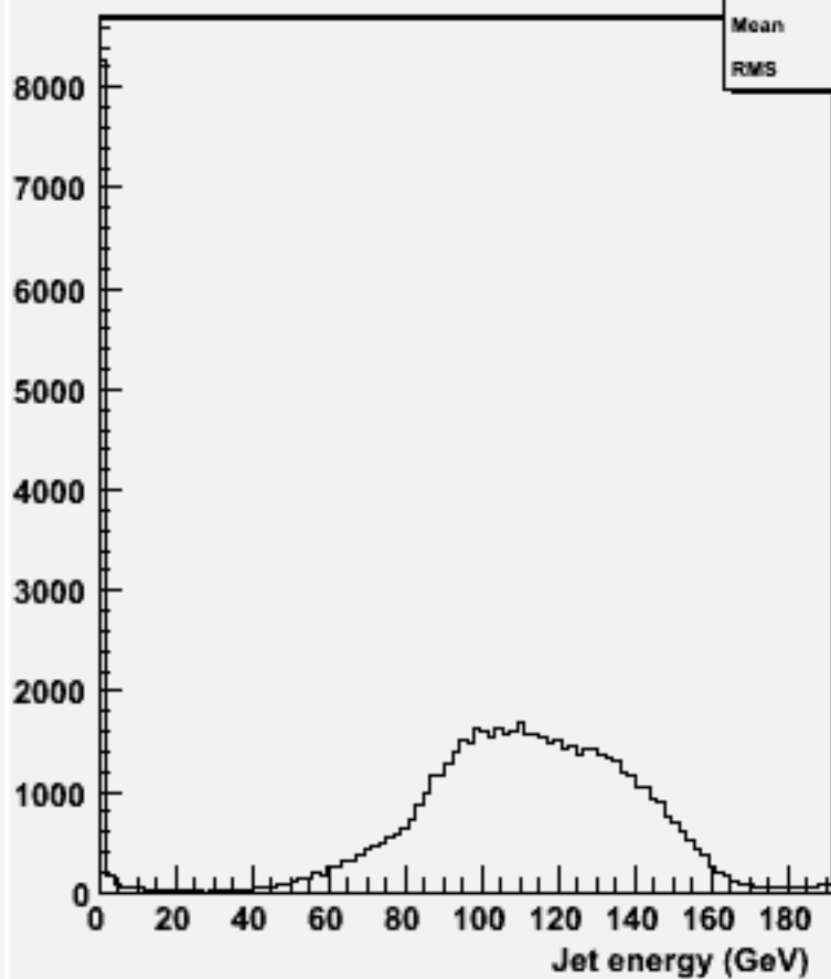
energy for 2-jets :w104492 bbh_o
