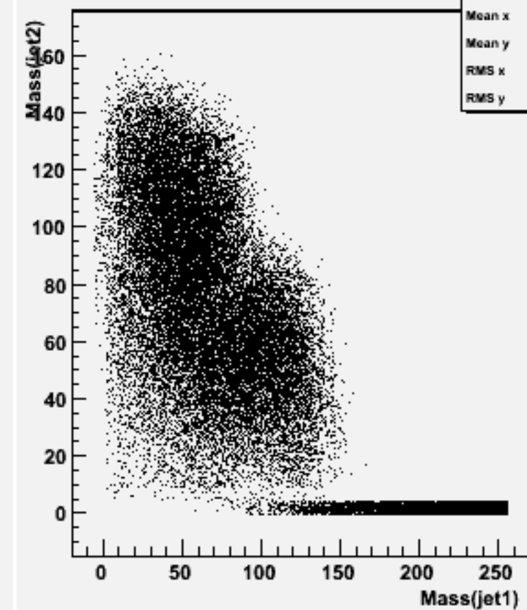
Jet mass for forced 2-jets : w104492 bbh_o
