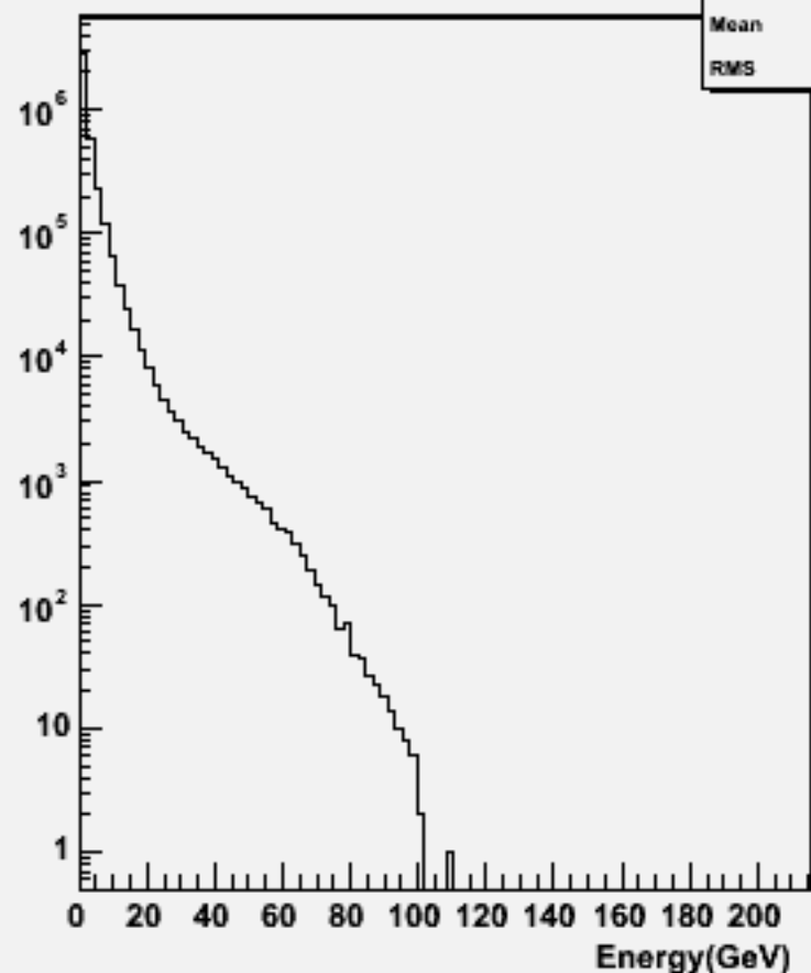
Particle Energy : w104492 bbh_o
