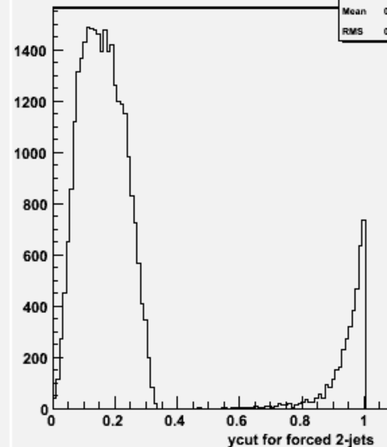
Ycut for 2-jets :w104492 bbh_o
