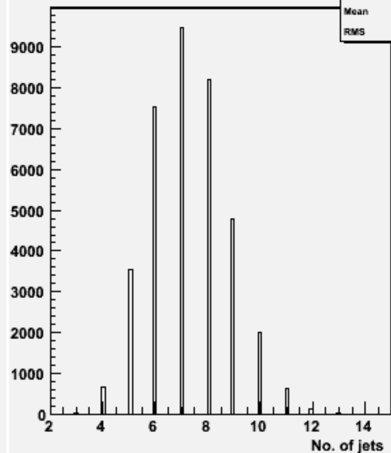
No. jets (ycut=0.001) : w104492 bbh_o
