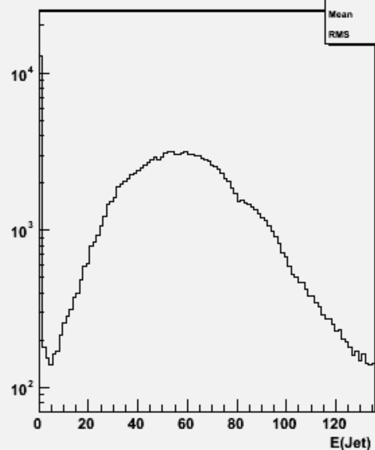
Jet energies(All jets)w104492 bbh_o
