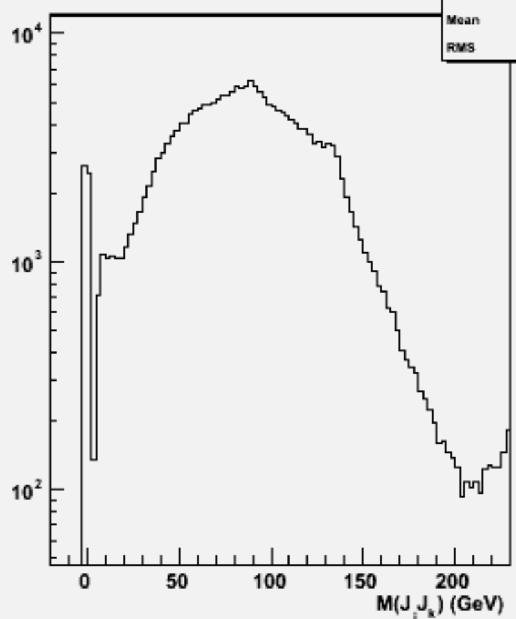
2jets mass(All comb)w104492 bbh_o
