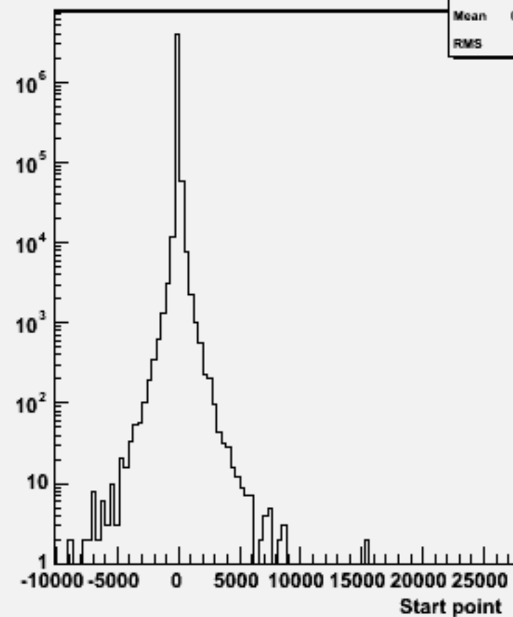
Start point Z : w104492 bbh_o
