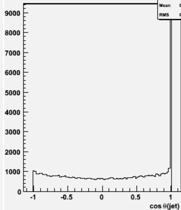
cos \theta for 2-jets :w104492 bbh_o
