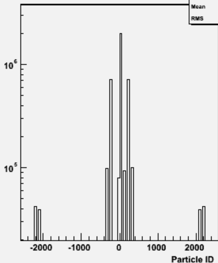
Particle ID : w104492 bbh_o
