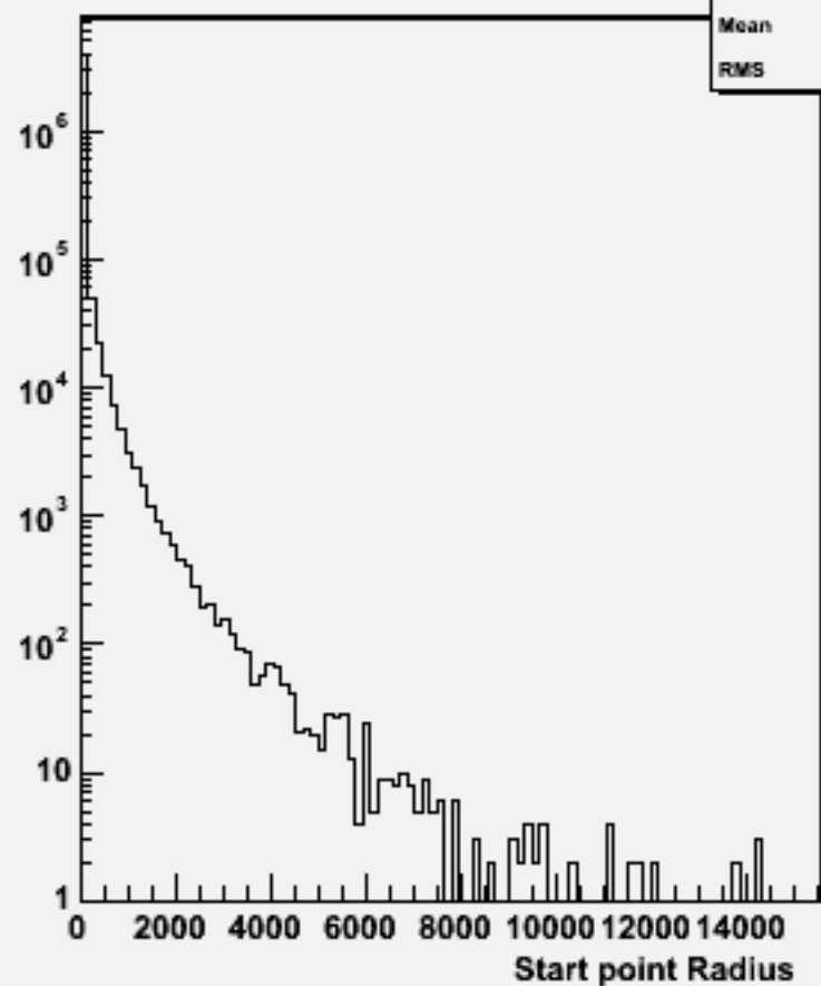
Start point R : w104492 bbh_o
