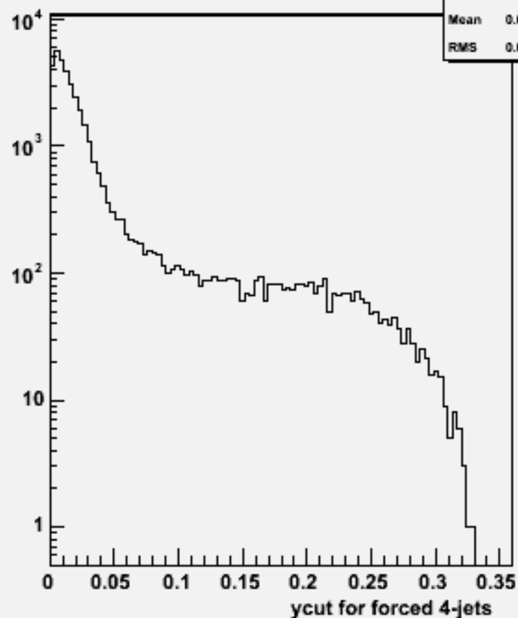
Ycut for 4-jets :w104492 bbh_o
