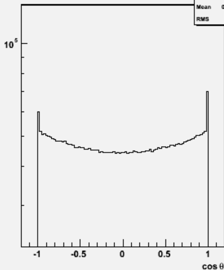
Particle cosθ : w104492 bbh_o
