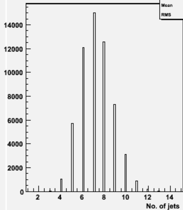
No. jets (ycut=0.001) : w104487 ssh_o
