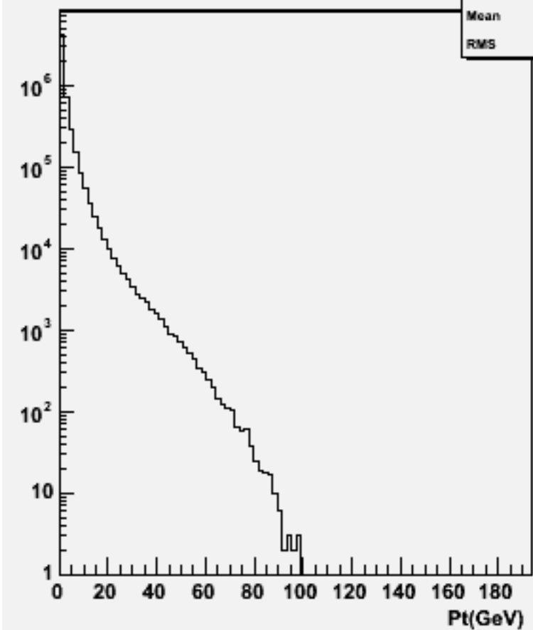
Start point Z : w104487 ssh_o
