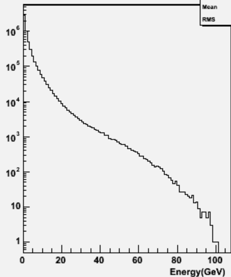
Start point R : w104487 ssh_o
