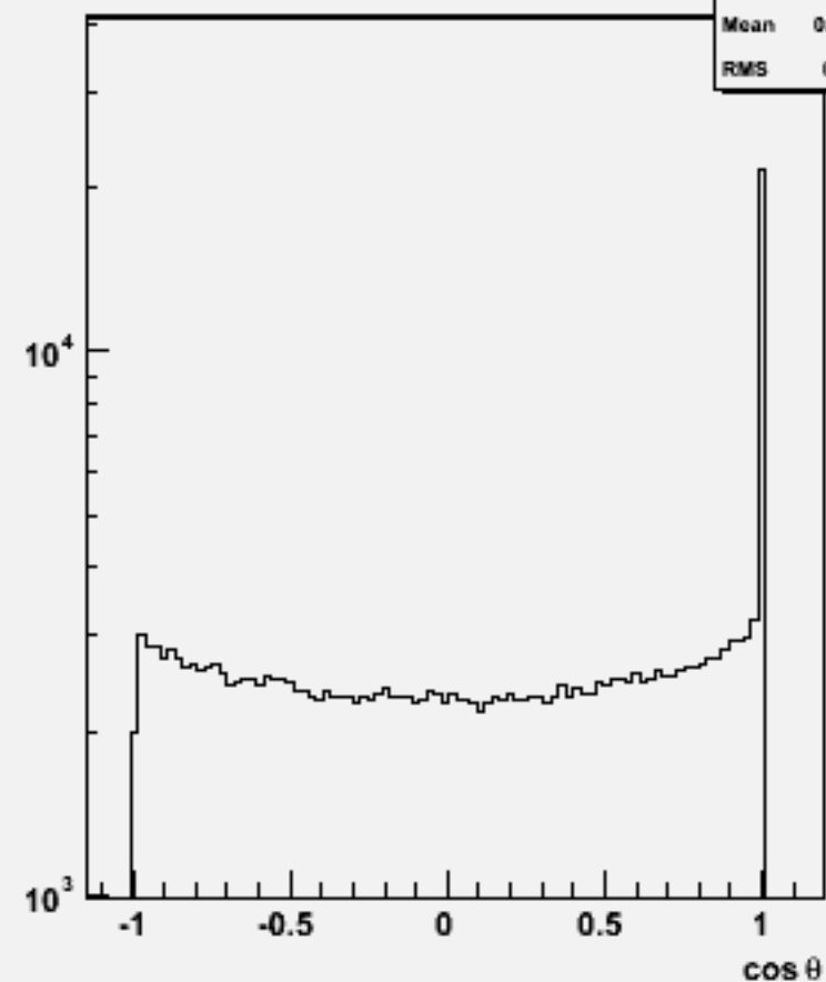
Jet cos \theta (All jets)w104487 ssh_o
