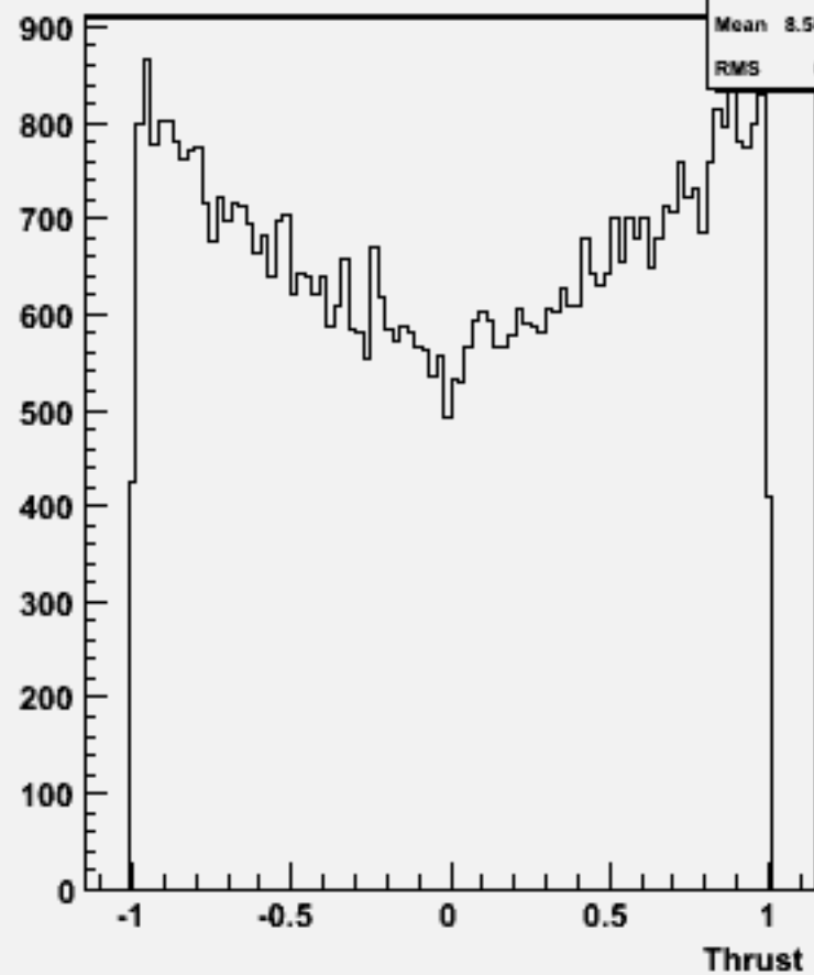
cos \theta (thrust) w104487 ssh_o
