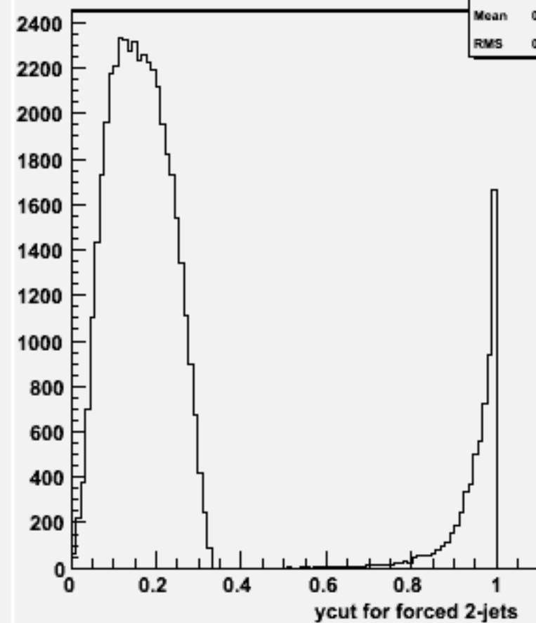
Ycut for 2-jets :w104487 ssh_o
