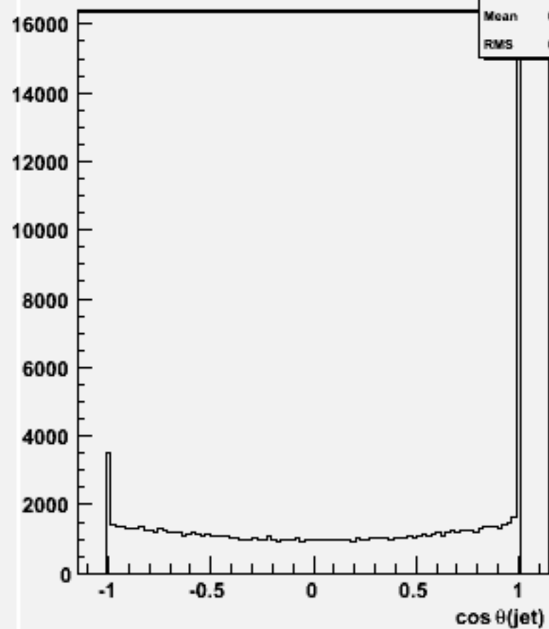
cos \theta for 2-jets :w104487 ssh_o
