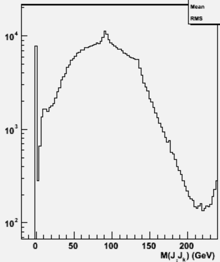
2jets mass(All comb)w104487 ssh_o
