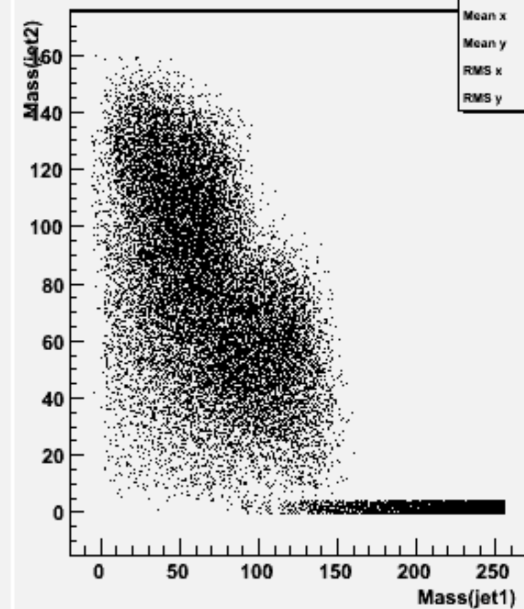
Jet mass for forced 2-jets : w104487 ssh_o
