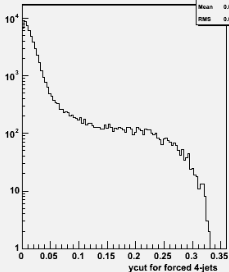
Ycut for 4-jets :w104487 ssh_o
