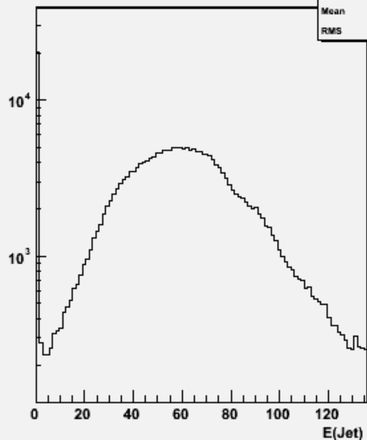
Jet energies(All jets)w104487 ssh_o
