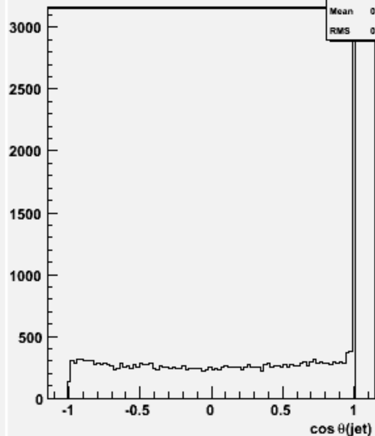
cos \theta for 2-jets :w104479 e3e3h_o
