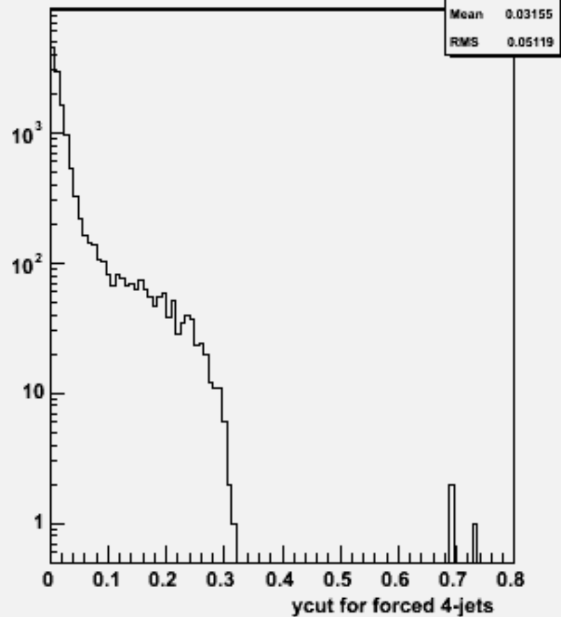
Ycut for 4-jets :w104479 e3e3h_o
