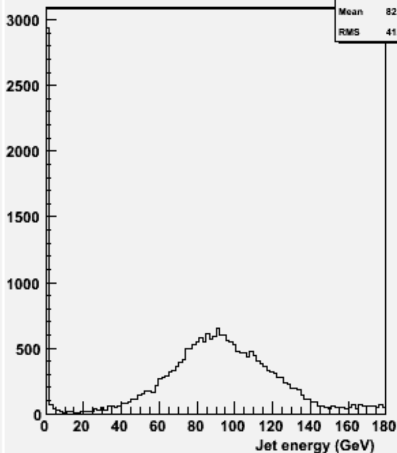
energy for 2-jets :w104479 e3e3h_o
