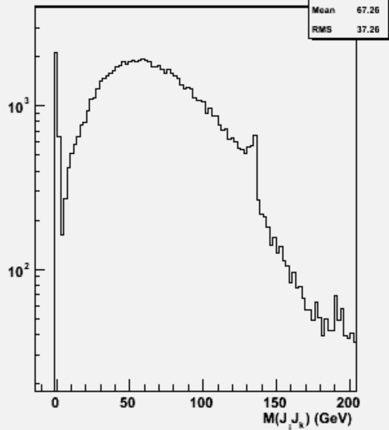
2jets mass(All comb)w104479 e3e3h_o
