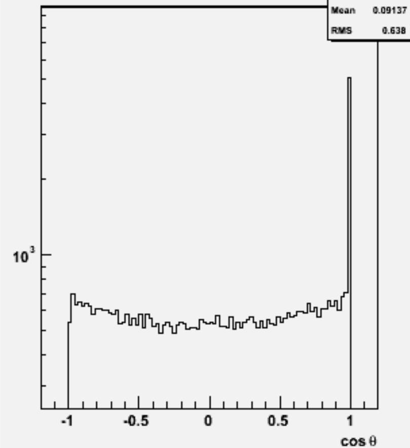
Jet cos \theta (All jets)w104479 e3e3h_o
