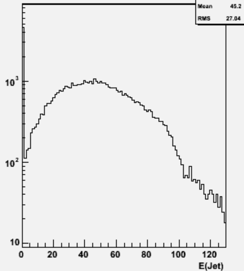
Jet energies(All jets)w104479 e3e3h_o
