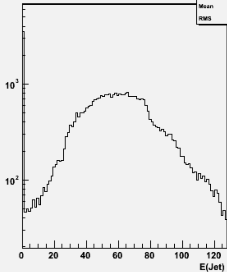
Jet energies(All jets)w104476 e2e2h_o
