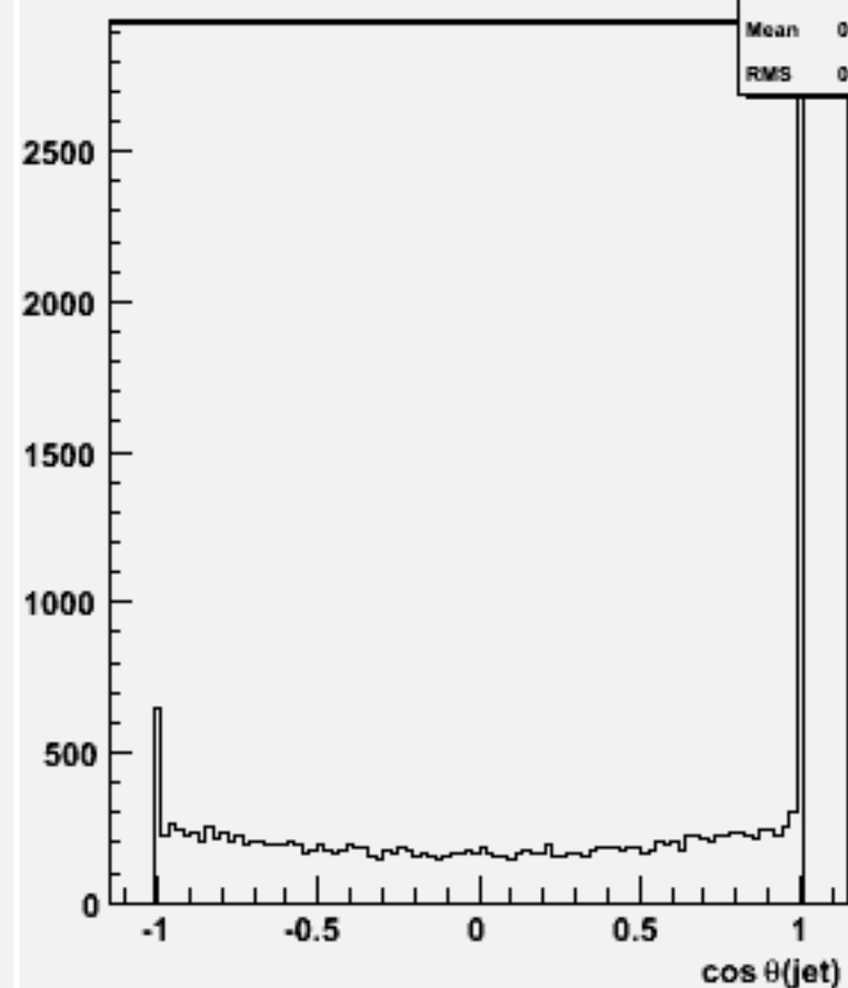
cos \theta for 2-jets :w104476 e2e2h_o
