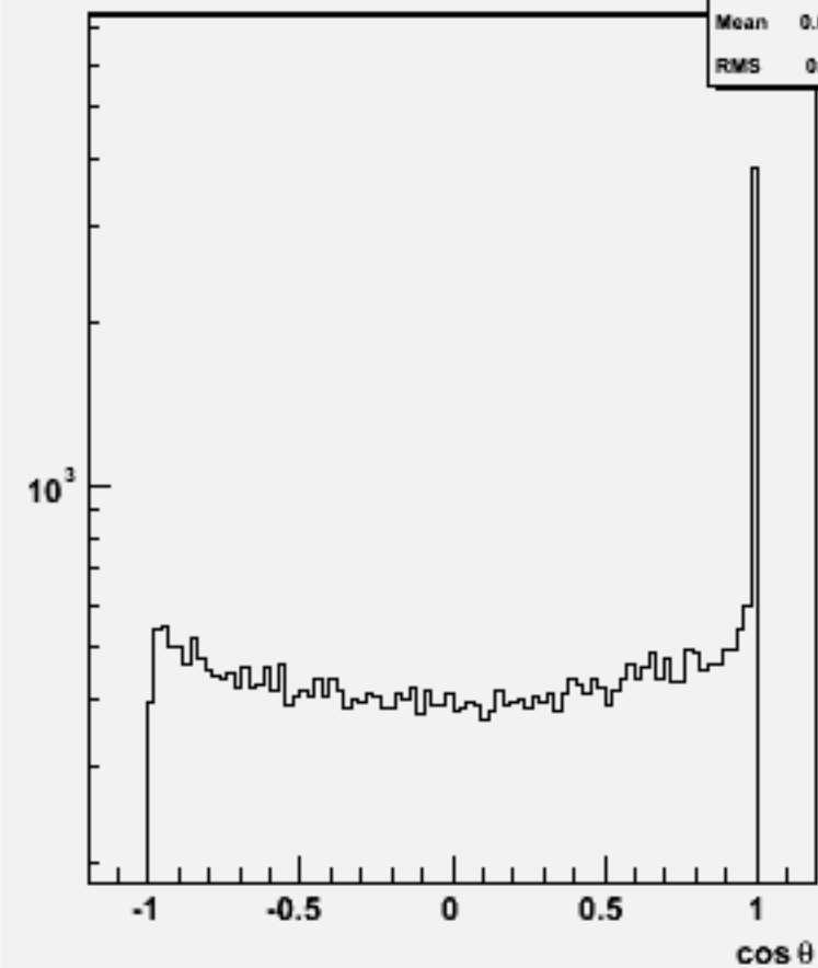
Jet cos \theta (All jets)w104476 e2e2h_o
