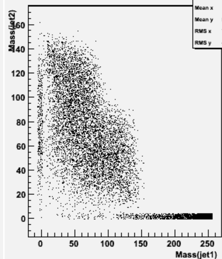
Jet mass for forced 2-jets : w104476 e2e2h_o
