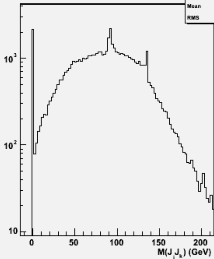
2jets mass(All comb)w104476 e2e2h_o
