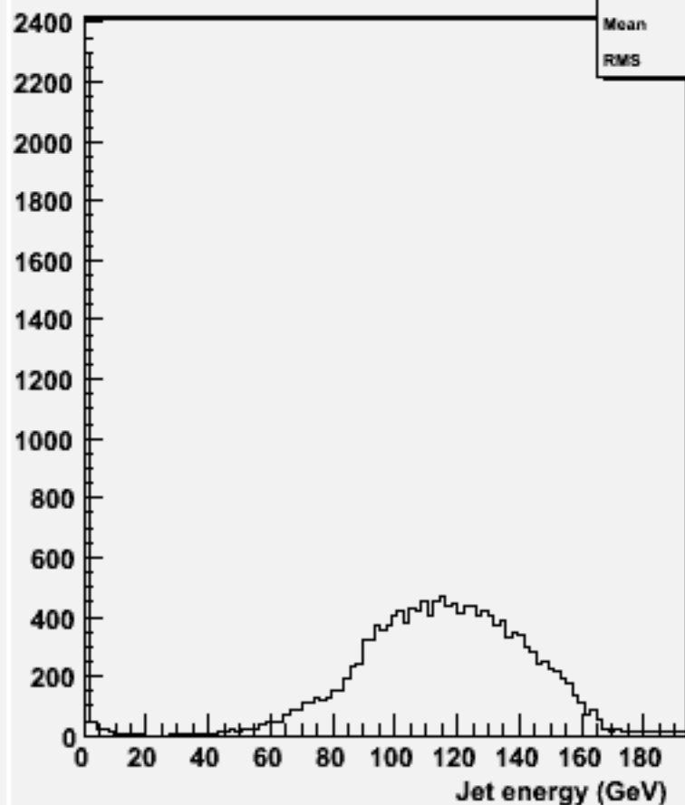
energy for 2-jets :w104476 e2e2h_o
