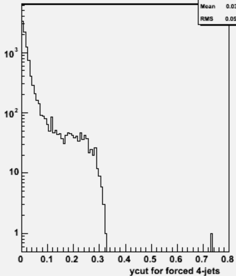
Ycut for 4-jets :w104476 e2e2h_o
