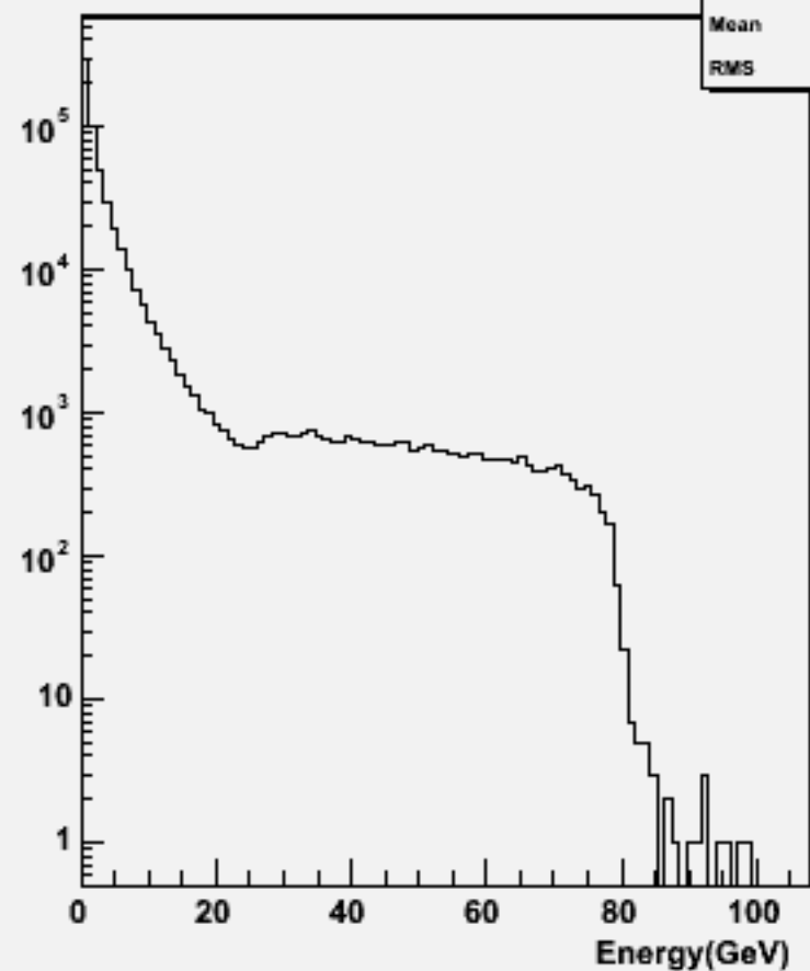
Particle Energy : w104476 e2e2h_o
