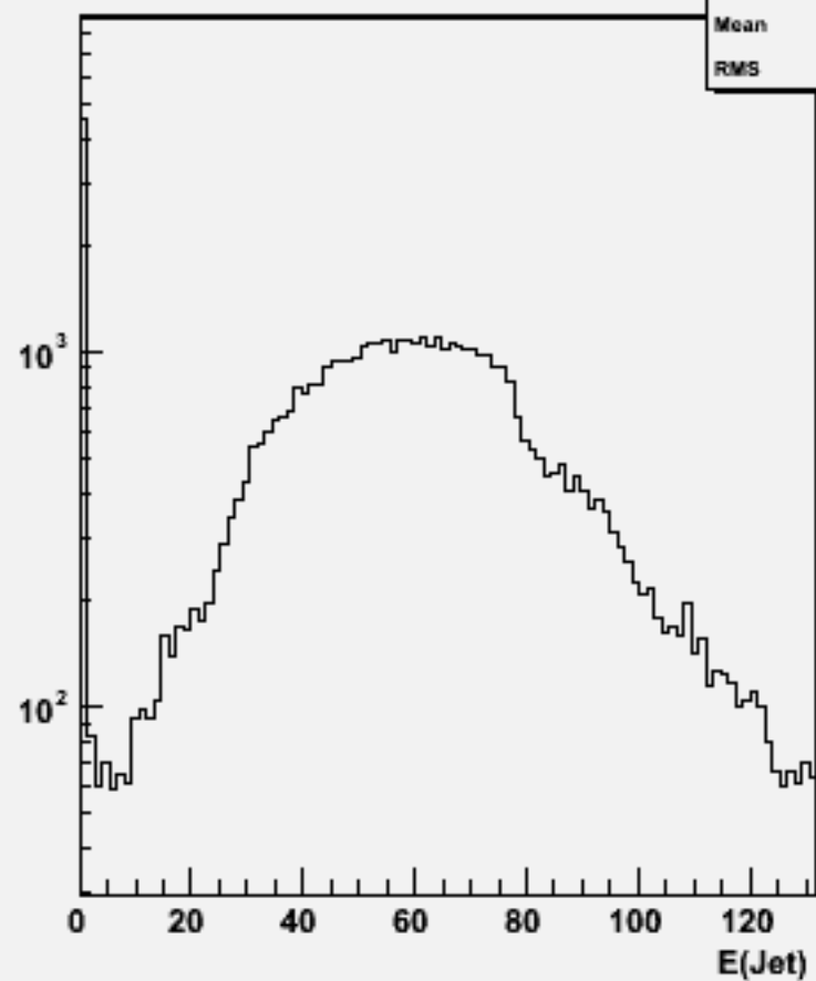
Jet energies(All jets)w104475 e2e2h_o
