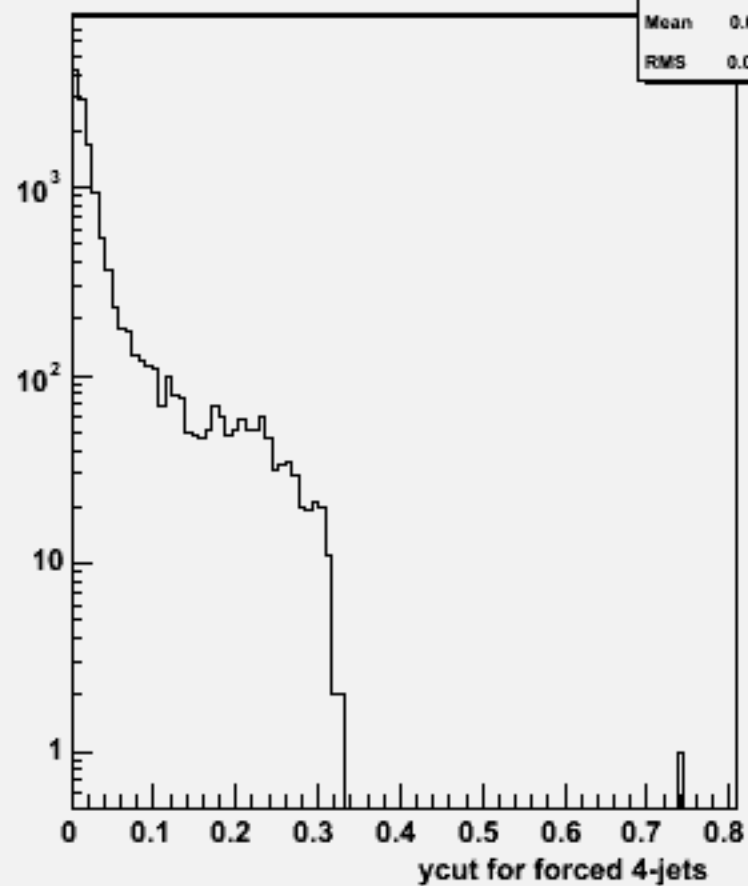
Ycut for 4-jets :w104475 e2e2h_o
