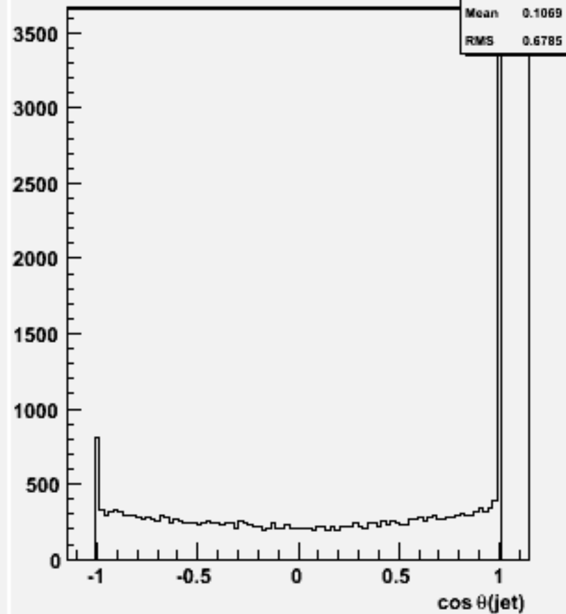
cos \theta for 2-jets :w104475 e2e2h_o
