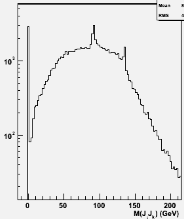
2jets mass(All comb)w104475 e2e2h_o
