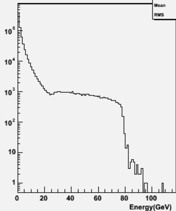
Particle Energy : w104475 e2e2h_o
