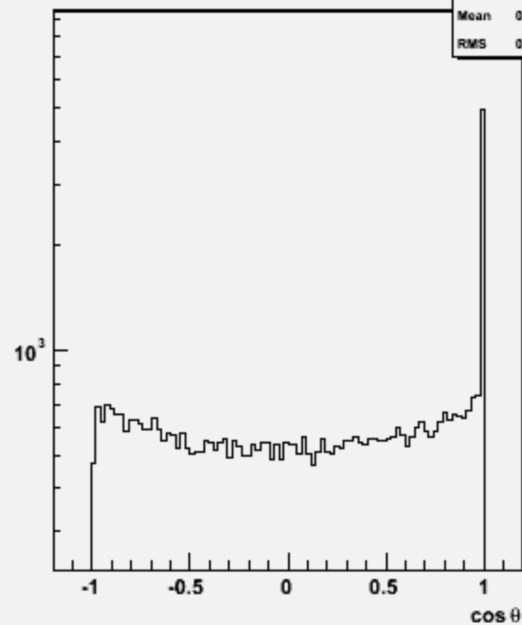
Jet cos \theta (All jets)w104475 e2e2h_o
