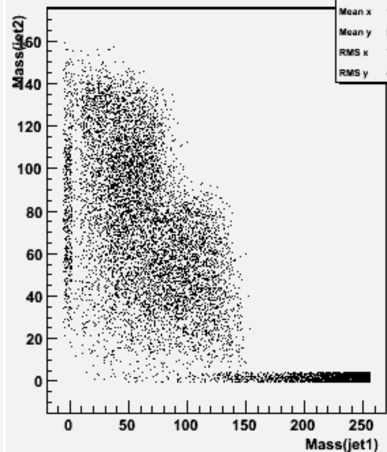
Jet mass for forced 2-jets : w104473 e1e1h_o
