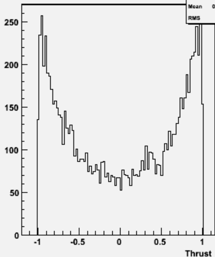
cos \Theta (thrust) w104473 e1e1h_o
