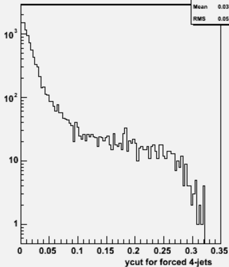
Ycut for 4-jets :w104473 e1e1h_o
