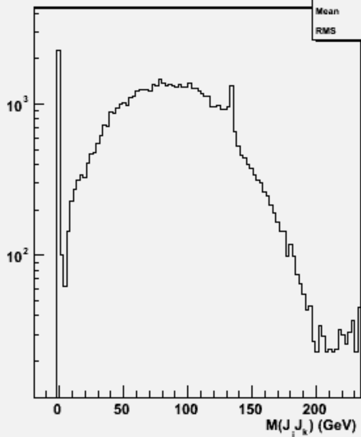
2jets mass(All comb)w104473 e1e1h_o
