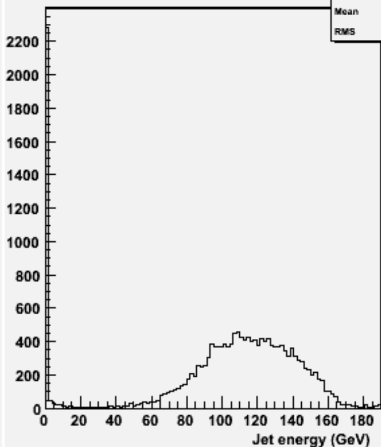
energy for 2-jets :w104473 e1e1h_o
