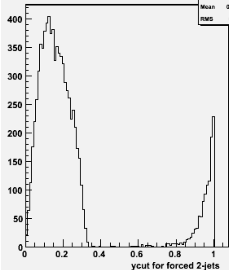
Ycut for 2-jets :w104473 e1e1h_o
