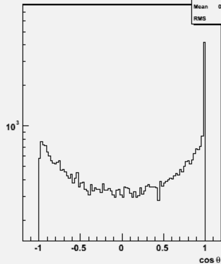
Jet cos \theta (All jets)w104473 e1e1h_o
