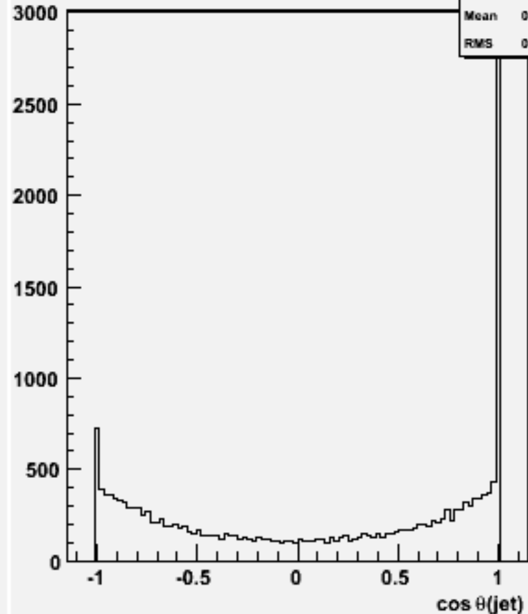
cos \theta for 2-jets :w104473 e1e1h_o
