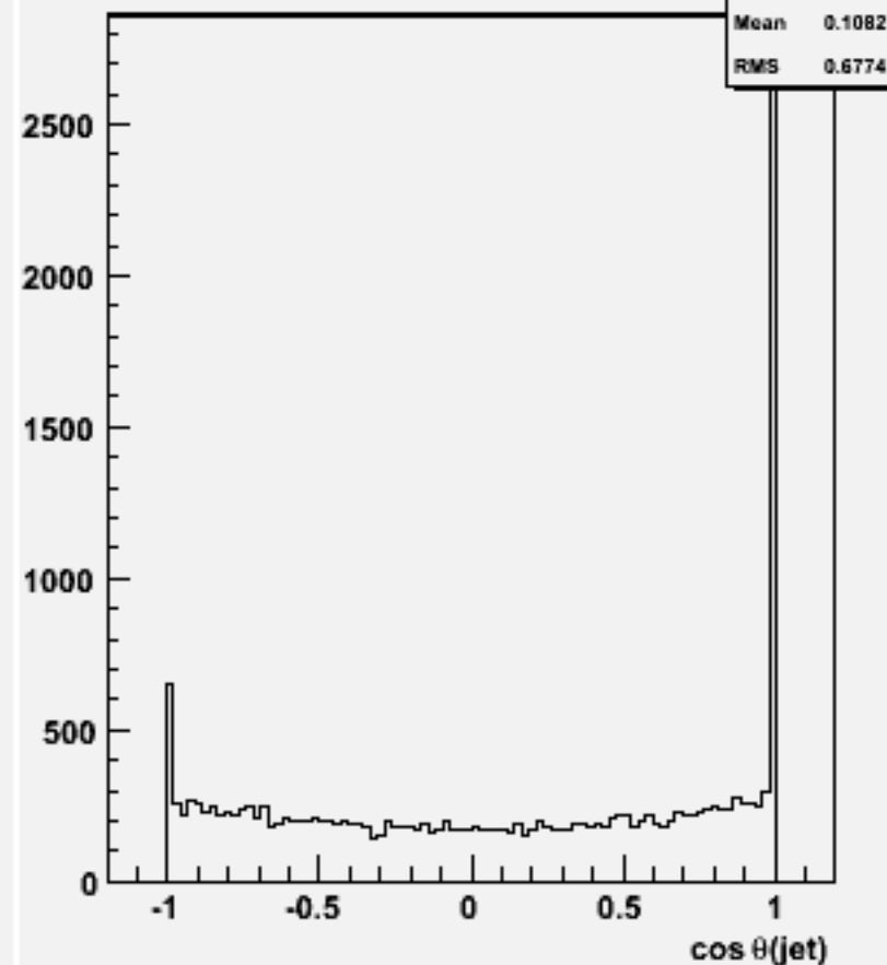
cos \theta for 2-jets :w104472 e1e1h_o
