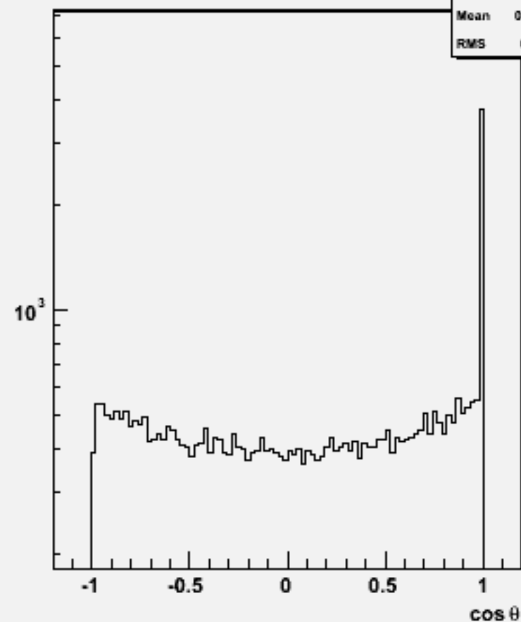
Jet cos \theta (All jets)w104472 e1e1h_o
