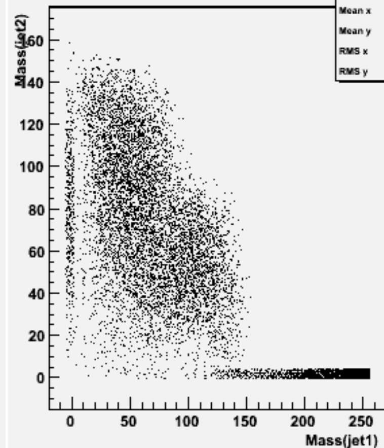
Jet mass for forced 2-jets : w104472 e1e1h_o
