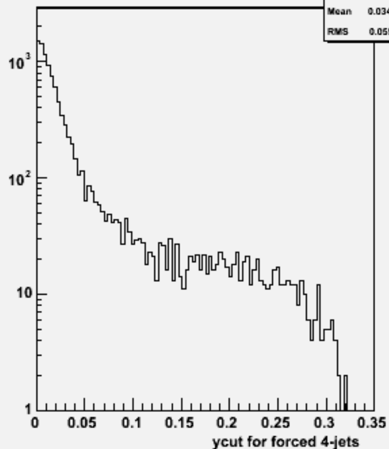
Ycut for 4-jets :w104472 e1e1h_o
