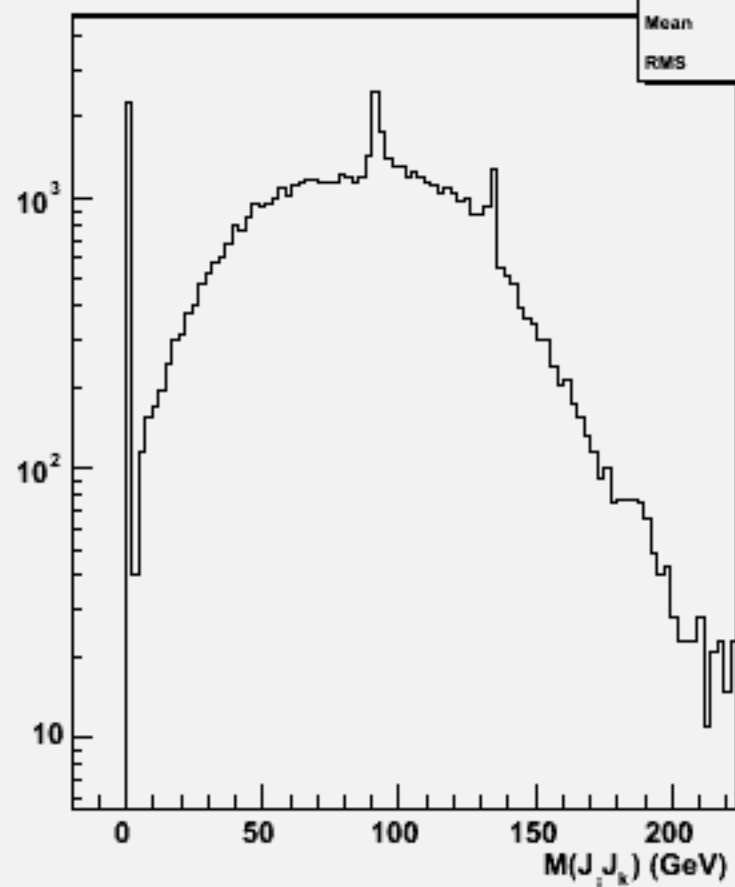
2jets mass(All comb)w104472 e1e1h_o
