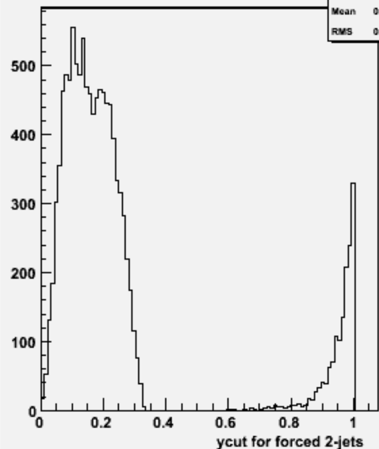
Ycut for 2-jets :w104471 e1e1h_o
