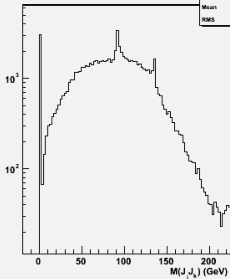
2jets mass(All comb)w104471 e1e1h_o
