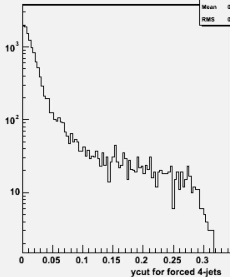
Ycut for 4-jets :w104471 e1e1h_o
