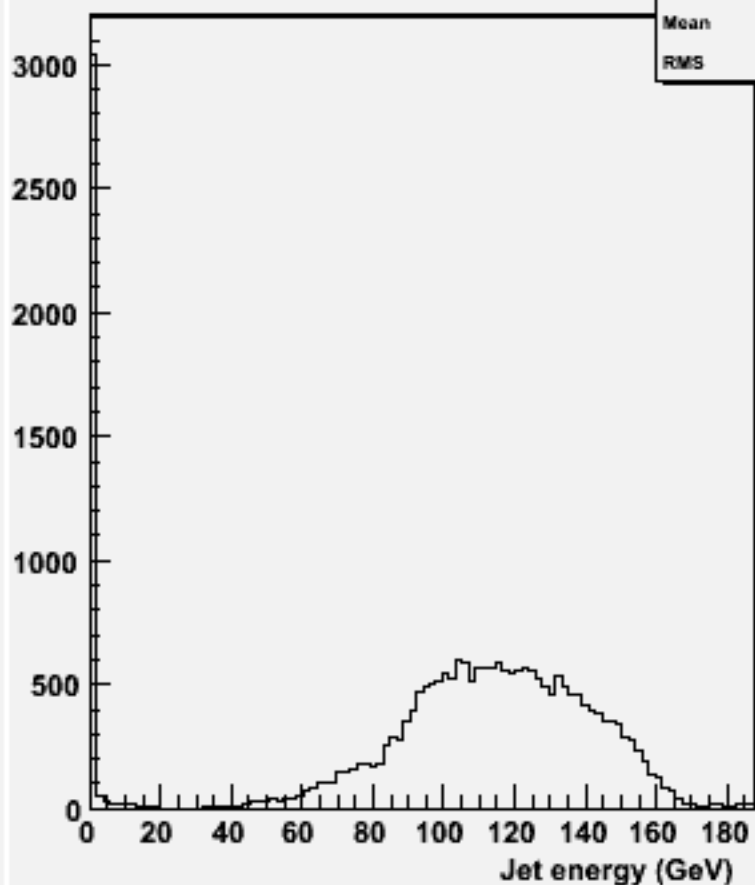
energy for 2-jets :w104471 e1e1h_o
