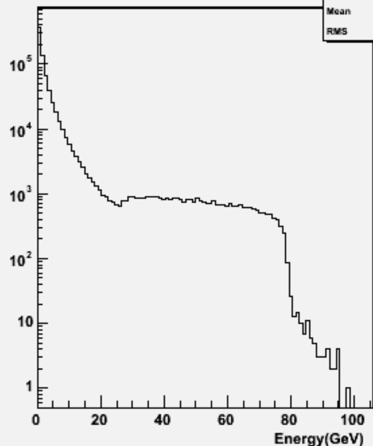
Particle Energy : w104471 e1e1h_o
