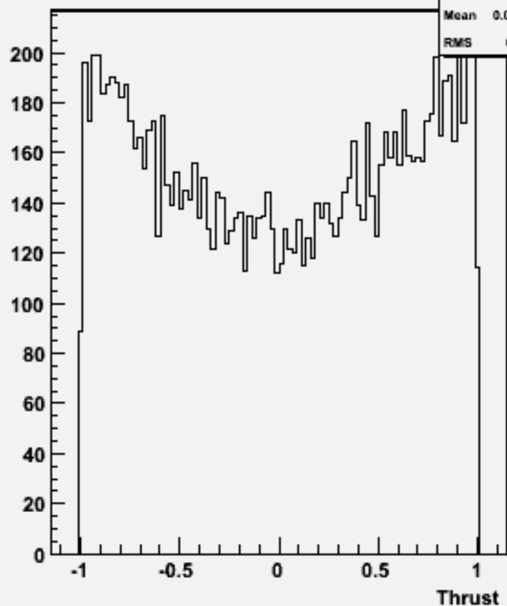
cos \Theta (thrust) w104471 e1e1h_o
