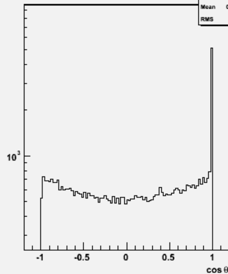
Jet cos \theta (All jets)w104471 e1e1h_o
