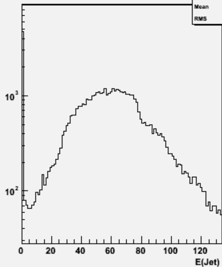
Jet energies(All jets)w104471 e1e1h_o
