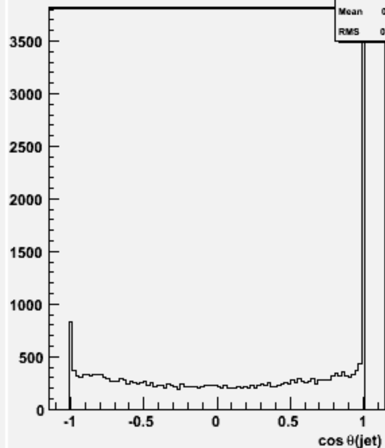
cos \theta for 2-jets :w104471 e1e1h_o
