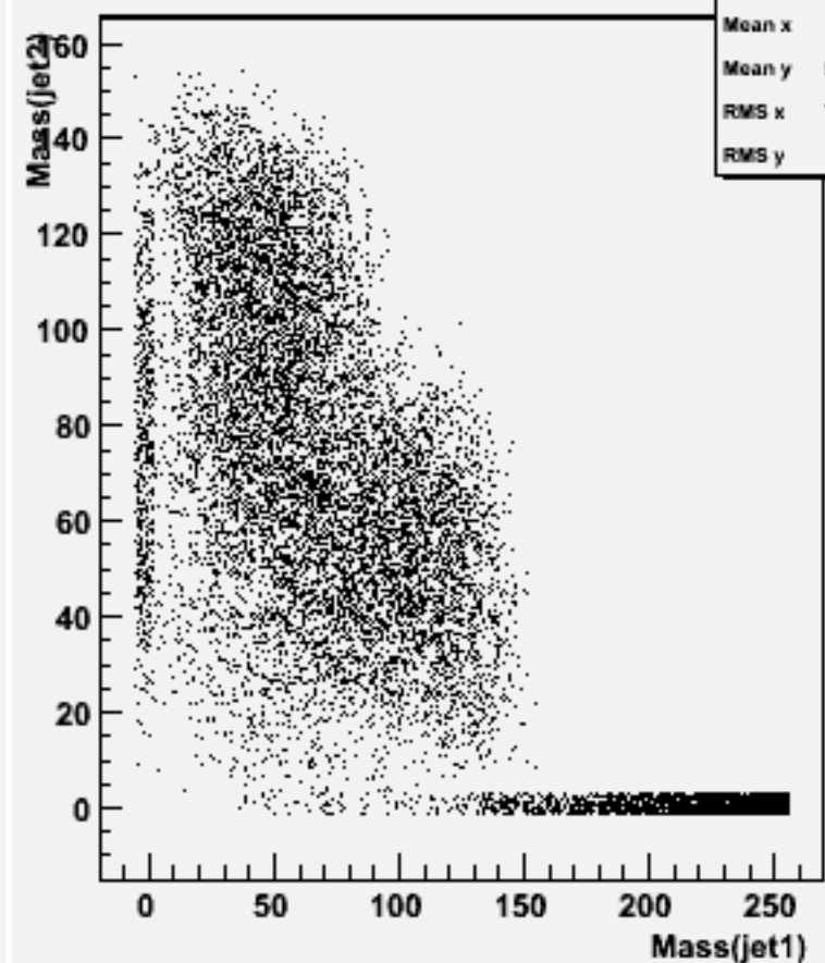
Jet mass for forced 2-jets : w104471 e1e1h_o
