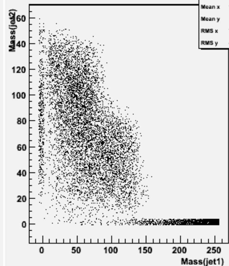
Jet mass for forced 2-jets : w104470 e1e1h_o
