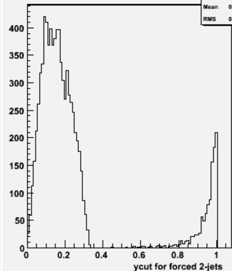
Ycut for 2-jets :w104470 e1e1h_o
