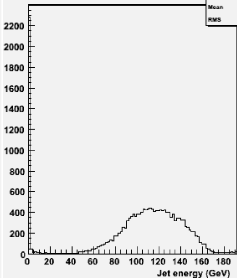
energy for 2-jets :w104470 e1e1h_o
