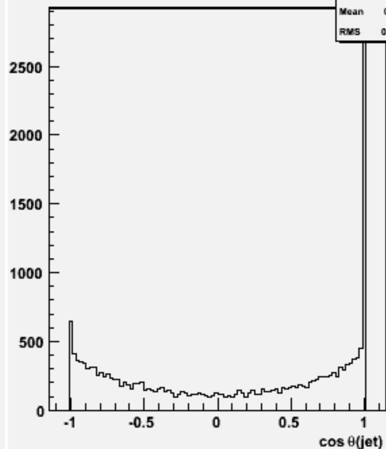
cos \theta for 2-jets :w104470 e1e1h_o
