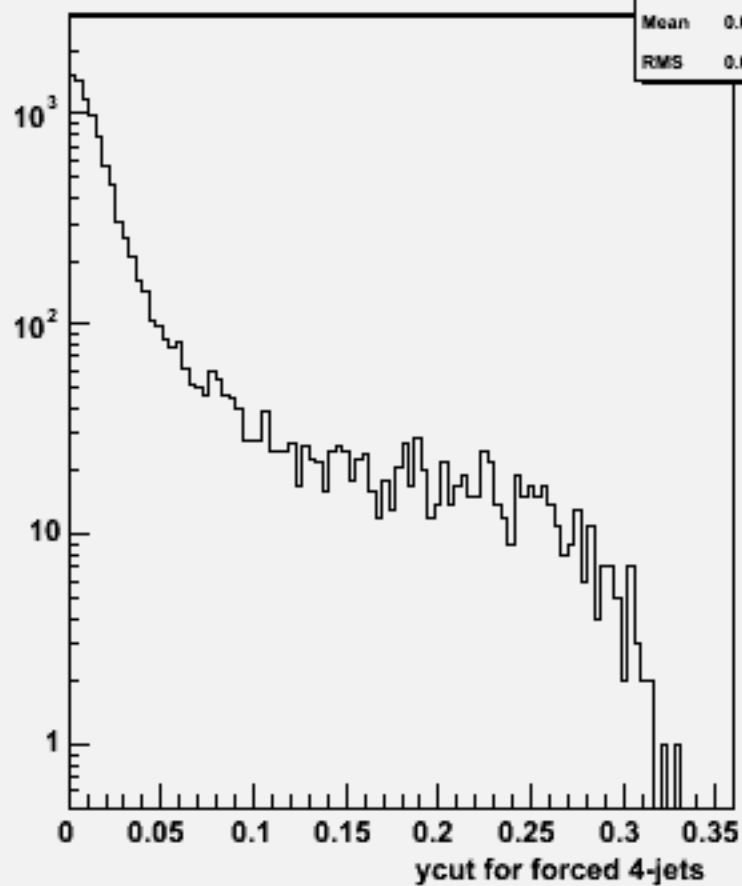
Ycut for 4-jets :w104470 e1e1h_o
