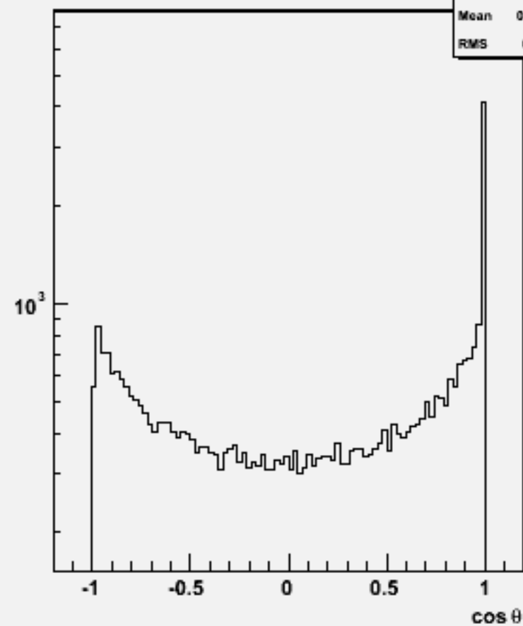
Jet cos \theta (All jets)w104470 e1e1h_o
