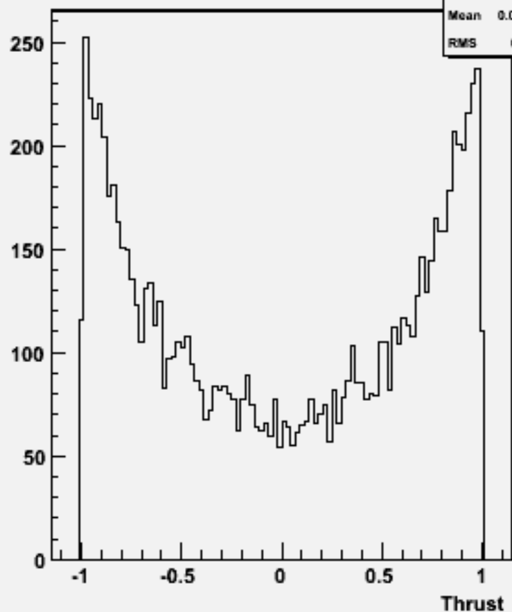
cos \theta (thrust) w104470 e1e1h_o
