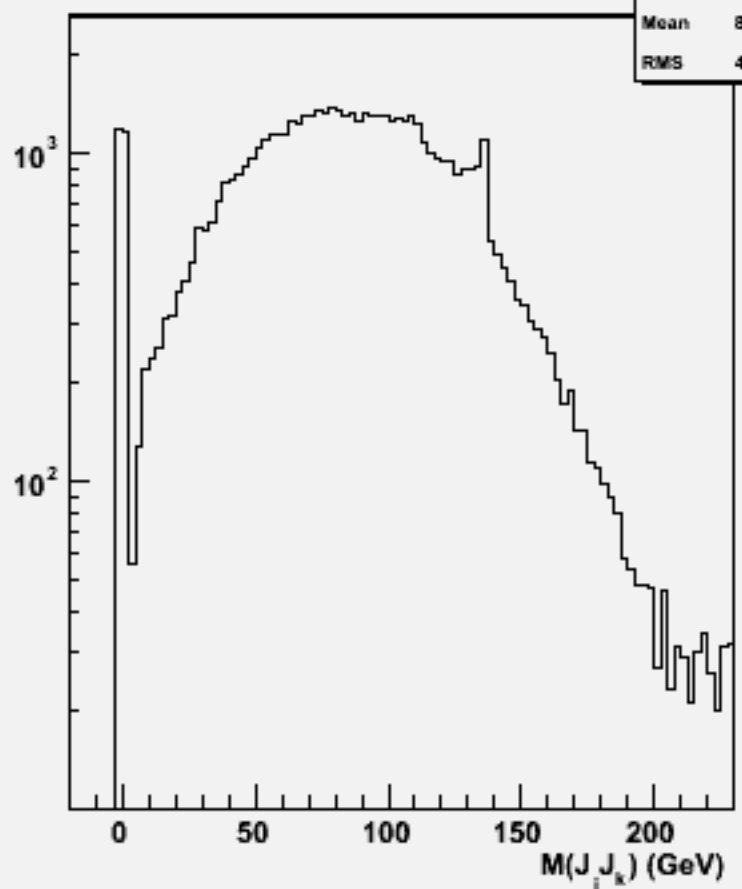
2jets mass(All comb)w104470 e1e1h_o
