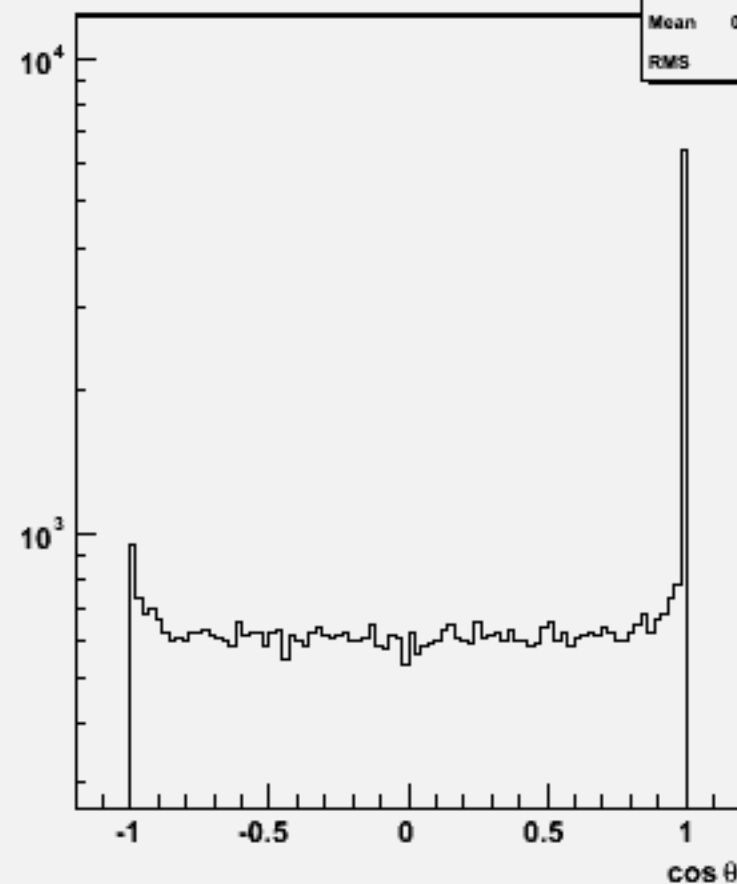
Jet cos \theta (All jets)w104460 n3n3h_o
