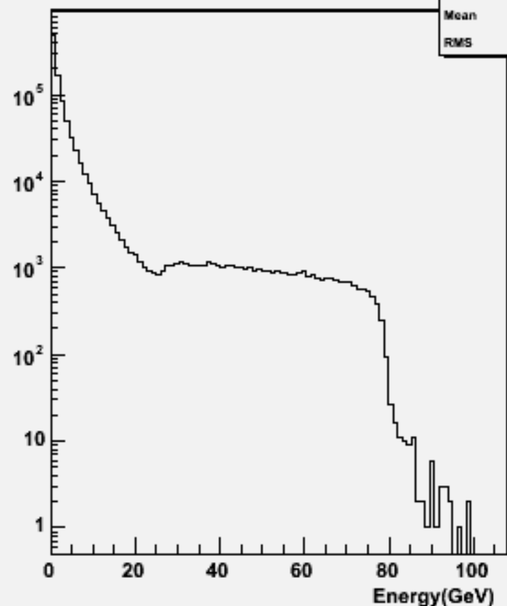
Particle Energy : w104460 n3n3h_o
