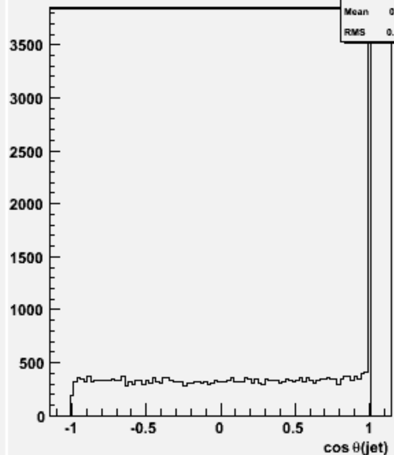
cos \theta for 2-jets :w104460 n3n3h_o
