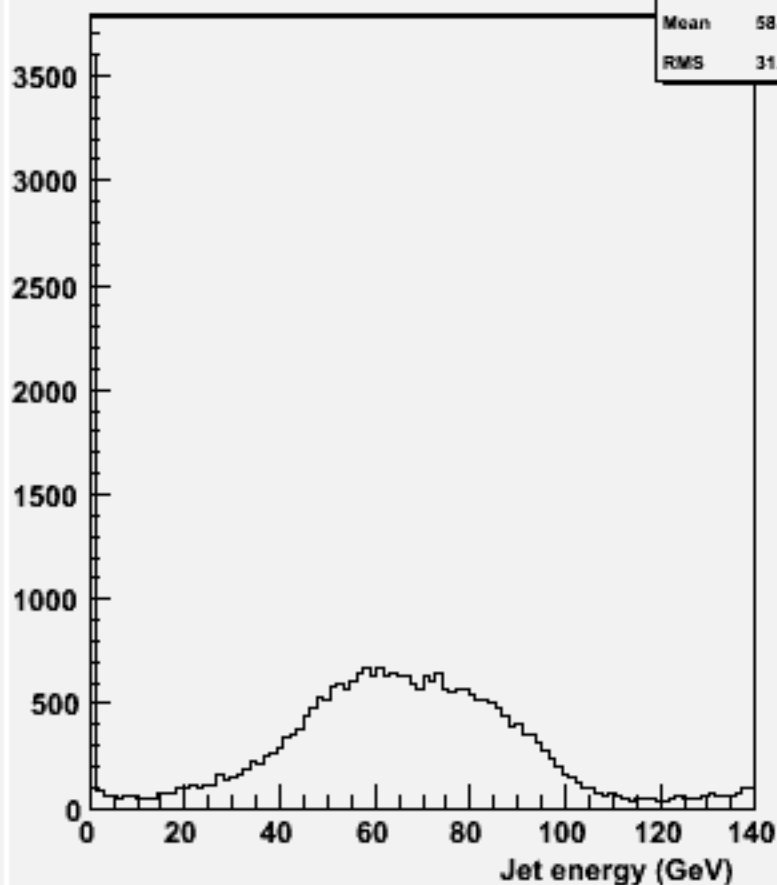
energy for 2-jets :w104460 n3n3h_o
