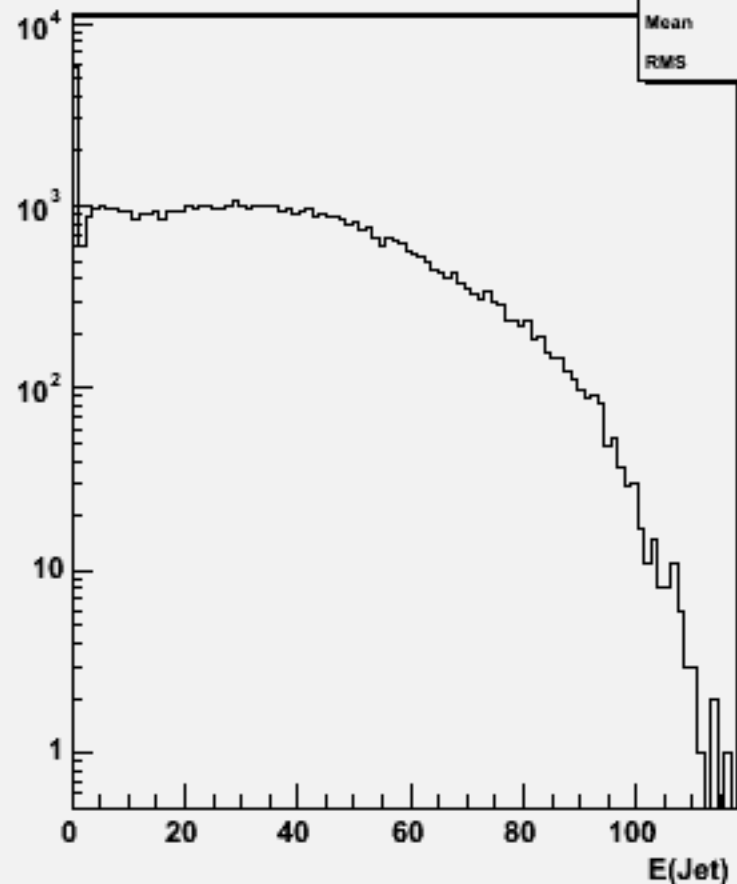
Jet energies(All jets)w104460 n3n3h_o
