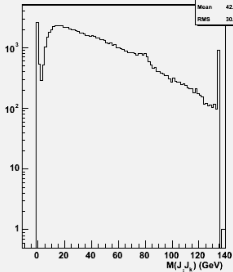
2jets mass(All comb)w104460 n3n3h_o
