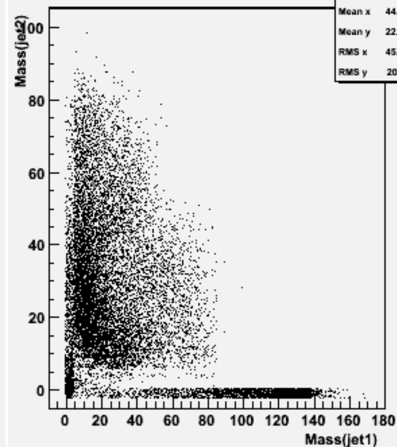
Jet mass for forced 2-jets : w104460 n3n3h_o
