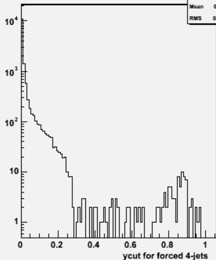
Ycut for 4-jets :w104460 n3n3h_o
