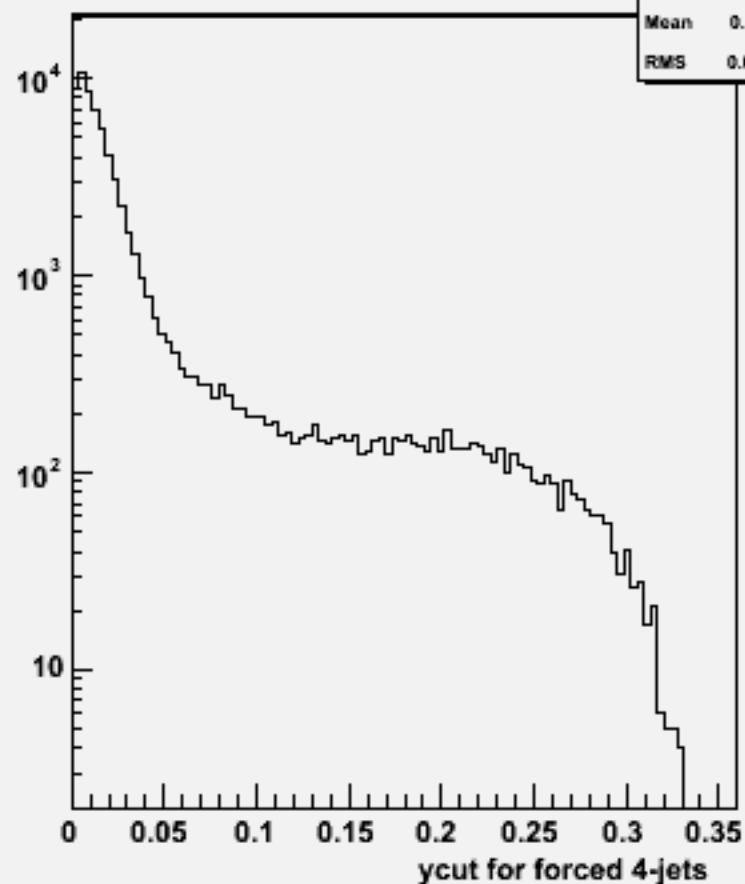
Ycut for 4-jets :w104441 bbh_o
