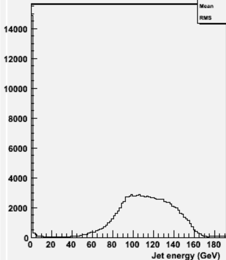
energy for 2-jets :w104441 bbh_o
