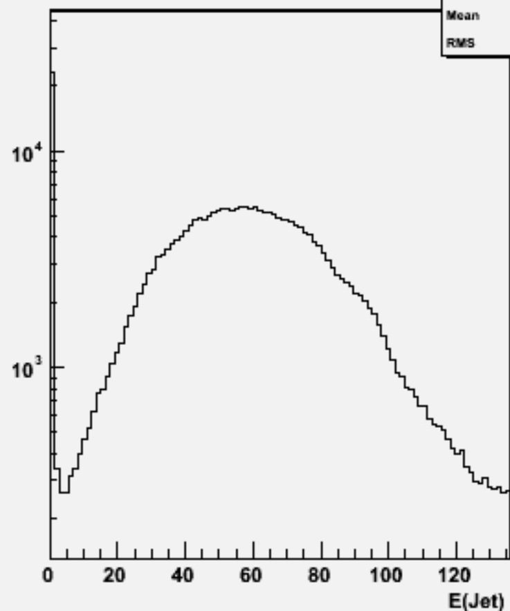
Jet energies(All jets)w104441 bbh_o
