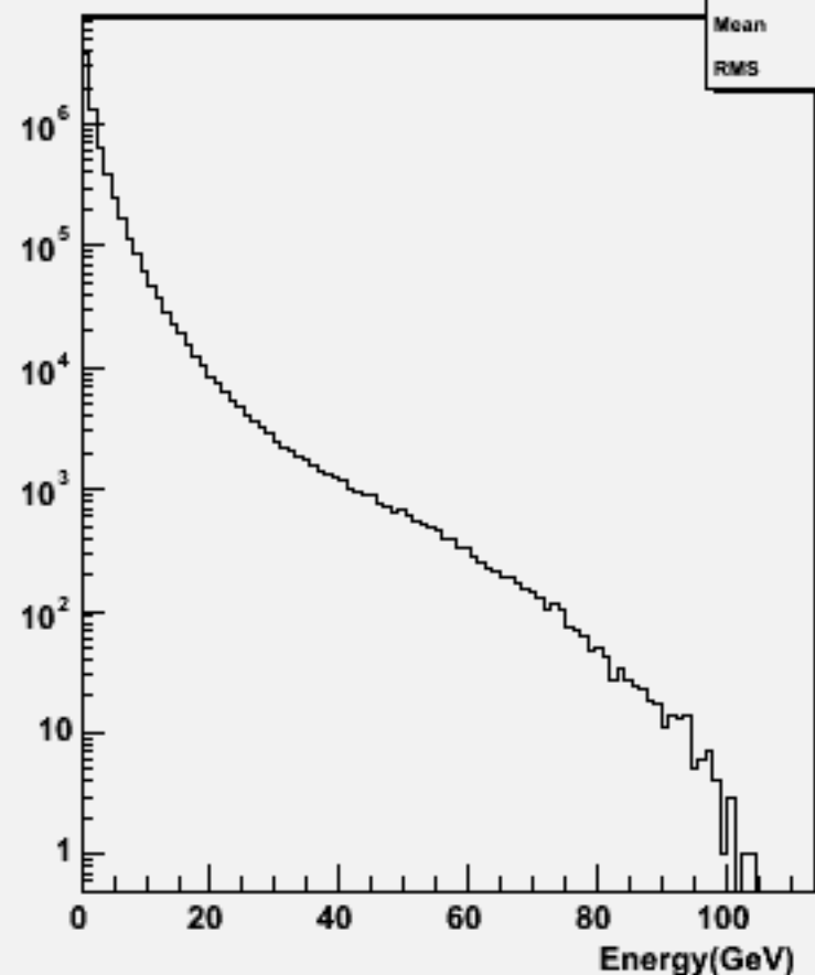
Start point R : w104441 bbh_o
