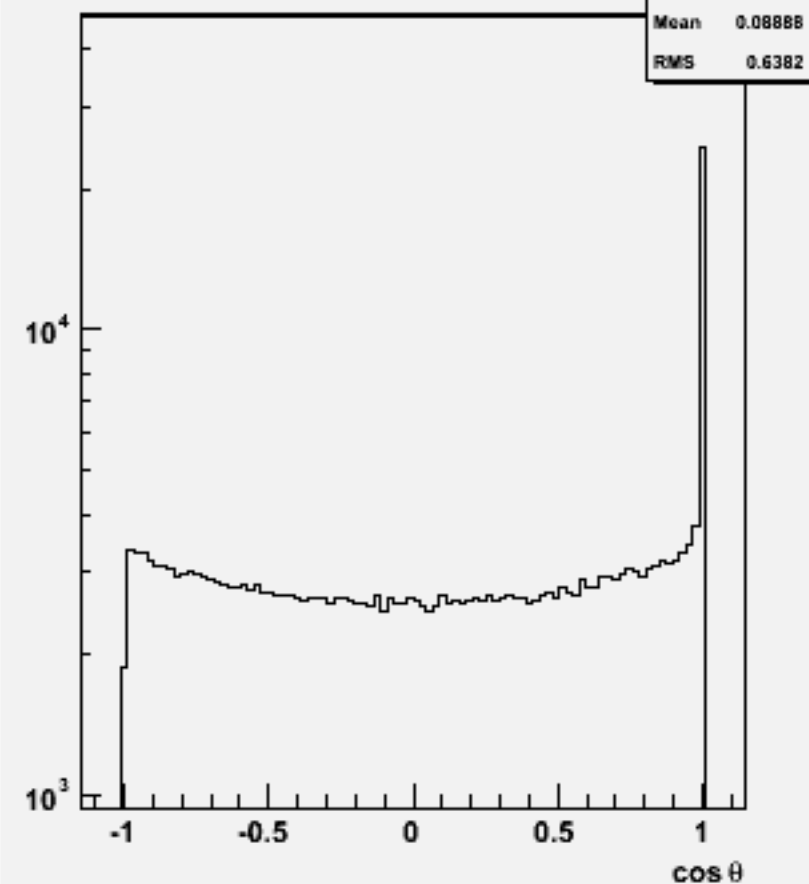
Jet cos \theta (All jets)w104441 bbh_o
