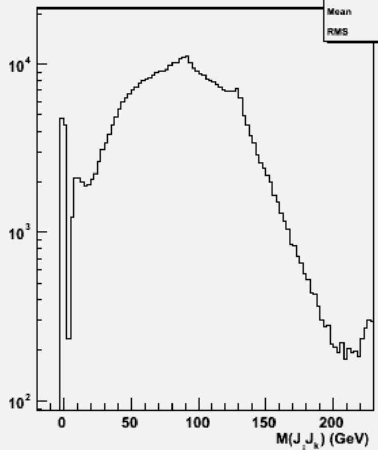
2jets mass(All comb)w104441 bbh_o
