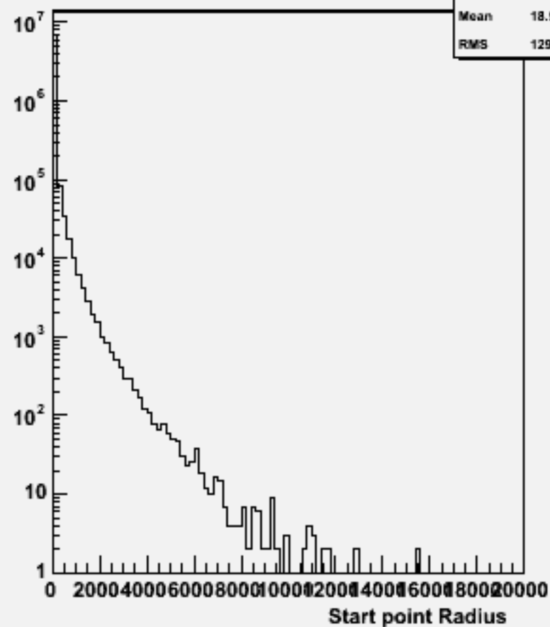
Start point R : w104441 bbh_o
