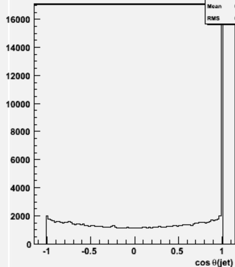
cos \theta for 2-jets :w104441 bbh_o
