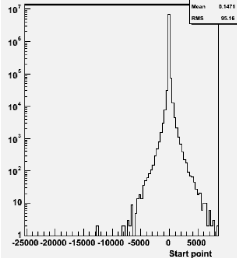
Start point Z : w104441 bbh_o
