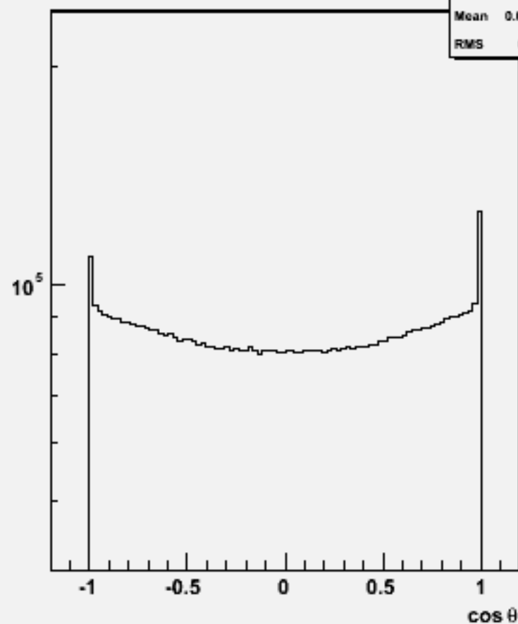
Particle cosθ : w104441 bbh_o
