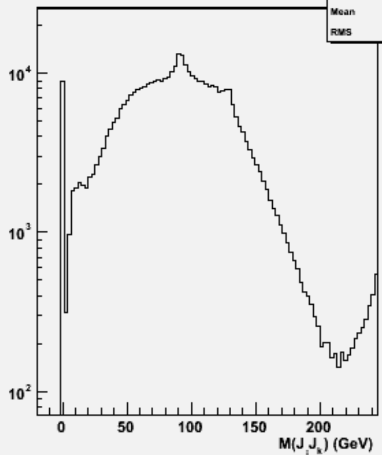
2jets mass(All comb)w104437 ssh_o
