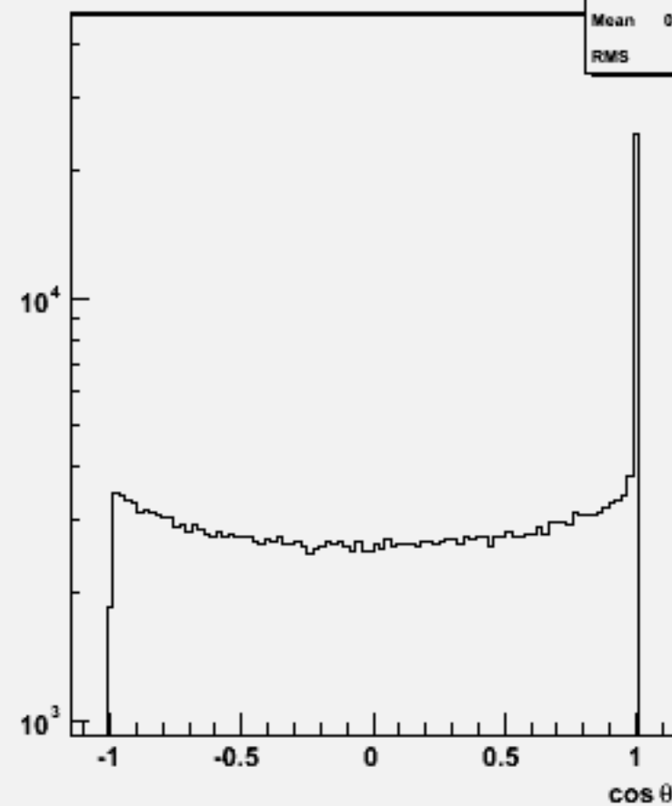
Jet cosθ (All jets)w104437 ssh_o
