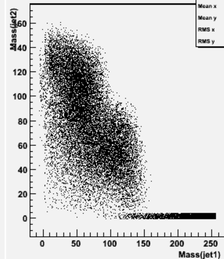
Jet mass for forced 2-jets : w104437 ssh_o
