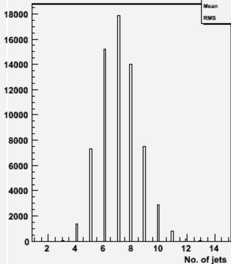
No. jets (ycut=0.001) : w104437 ssh_o
