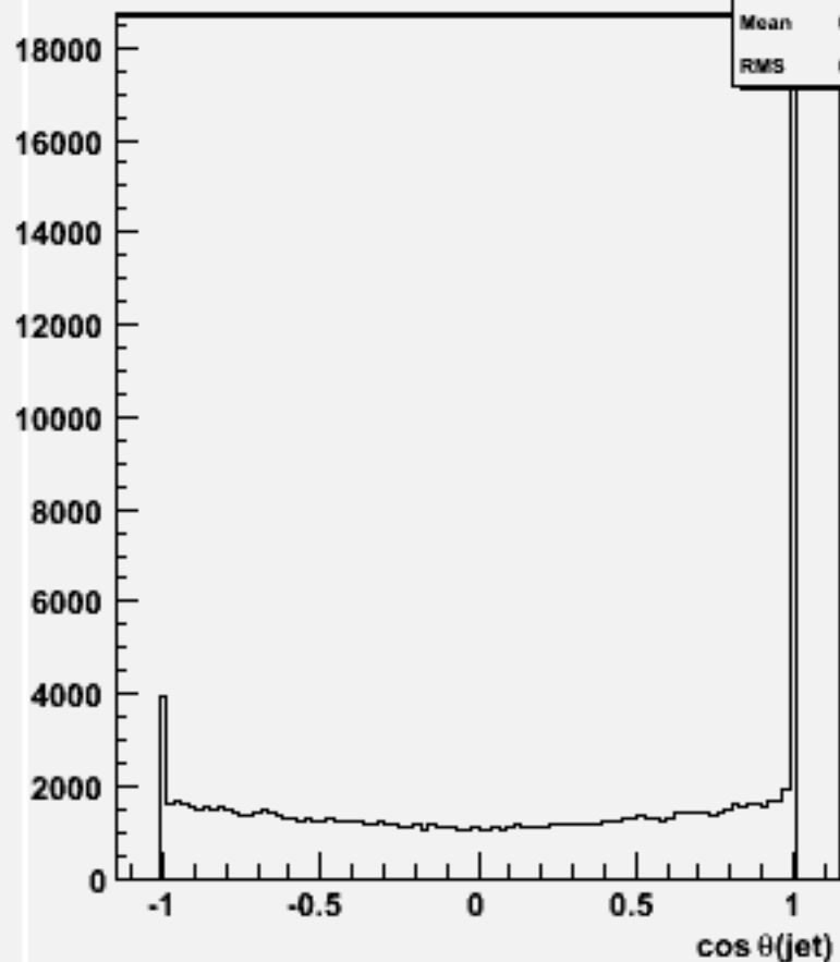
cos \theta for 2-jets :w104437 ssh_o
