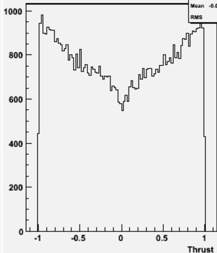
cos \Theta (thrust) w104437 ssh_o
