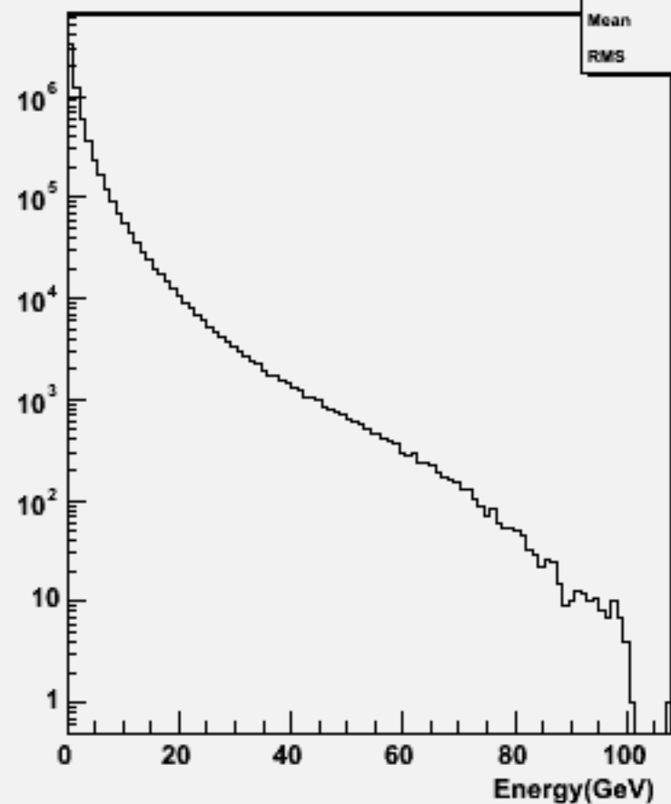
Start point R : w104437 ssh_o
