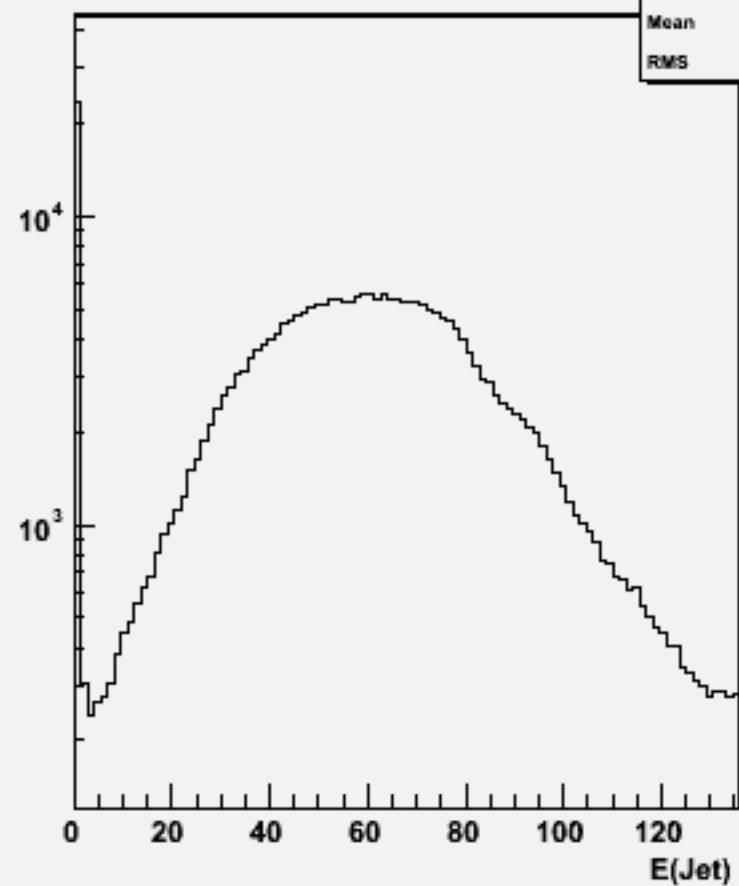
Jet energies(All jets)w104437 ssh_o
