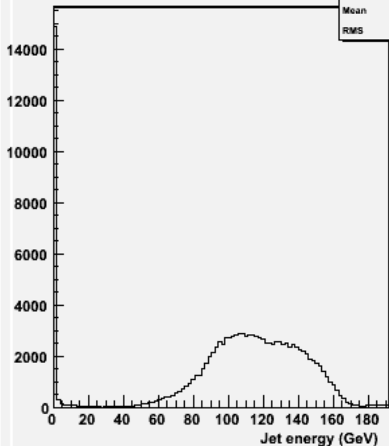
energy for 2-jets :w104437 ssh_o
