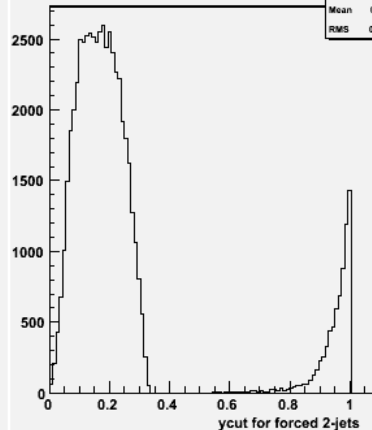
Ycut for 2-jets :w104437 ssh_o
