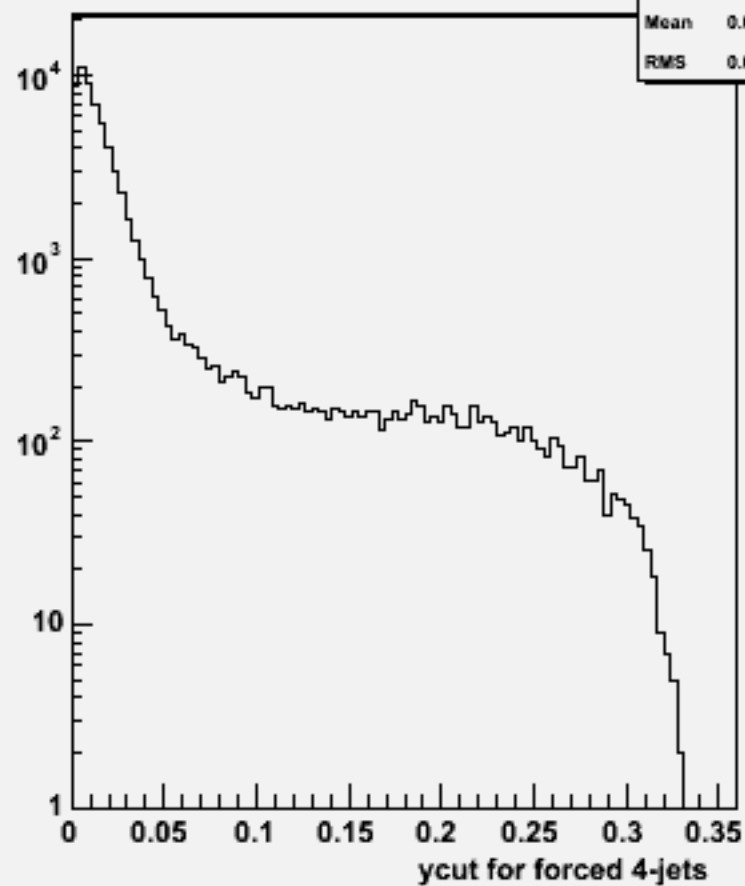
Ycut for 4-jets :w104437 ssh_o
