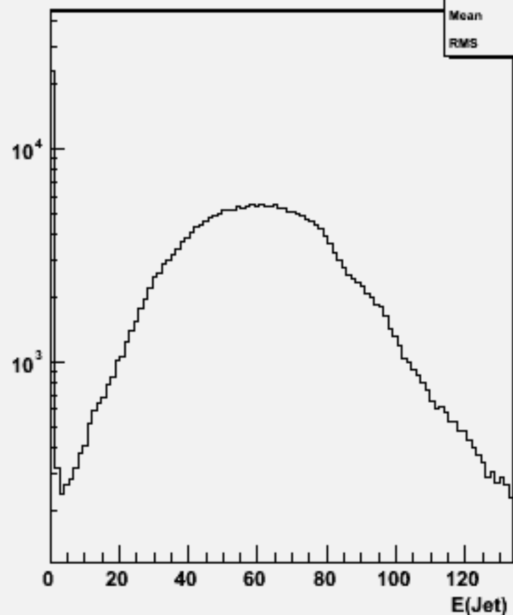
Jet energies(All jets)w104433 ddh_o
