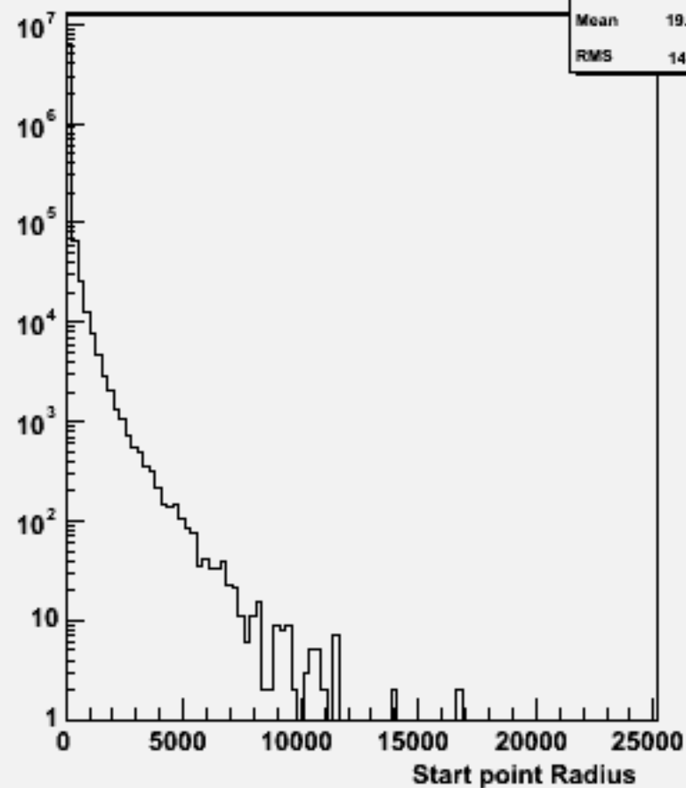
Start point R : w104433 ddh_o
