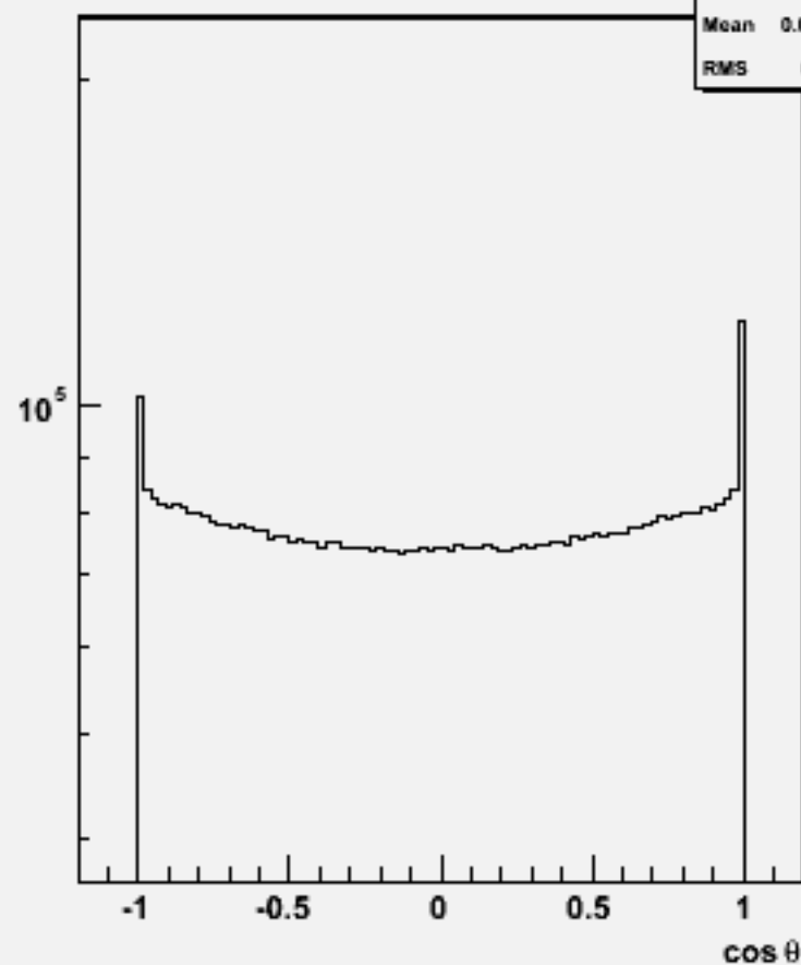
Particle \cos\theta : w104433 ddh_o
