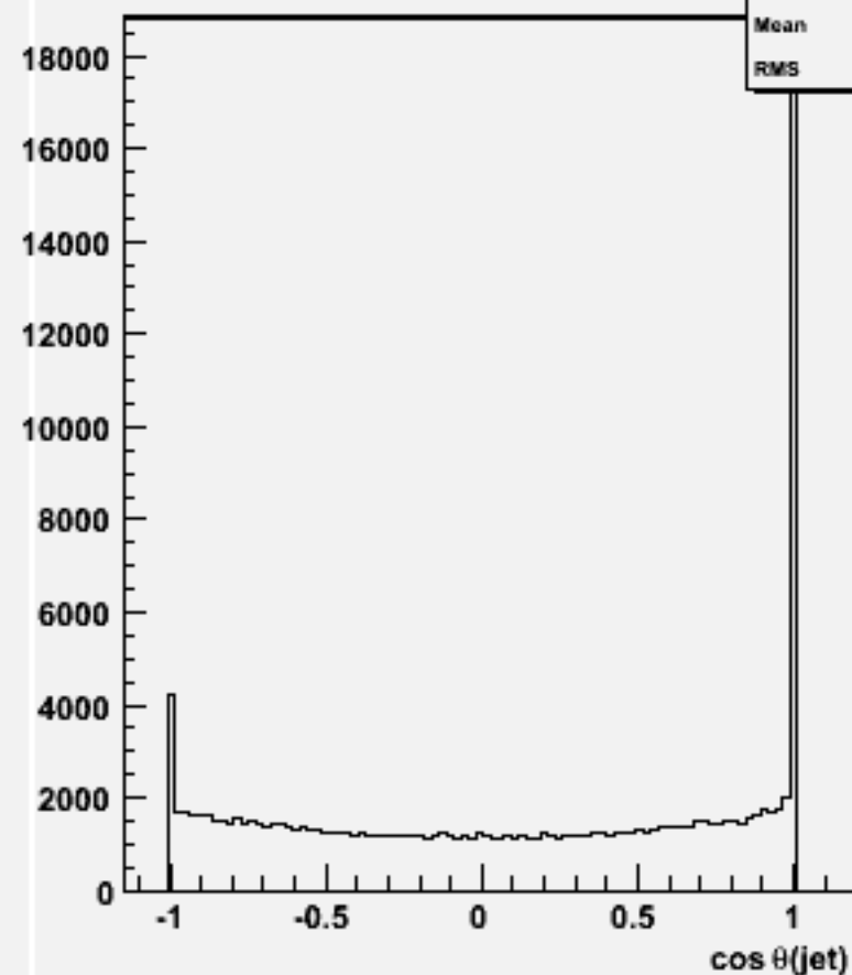
cos \theta for 2-jets :w104433 ddh_o
