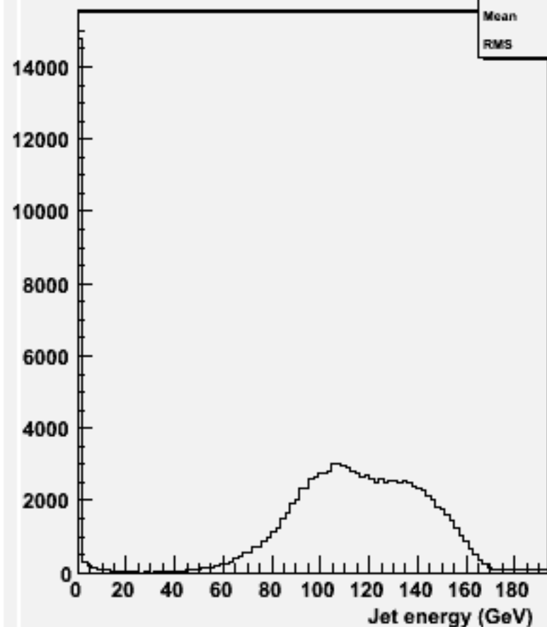
energy for 2-jets :w104433 ddh_o
