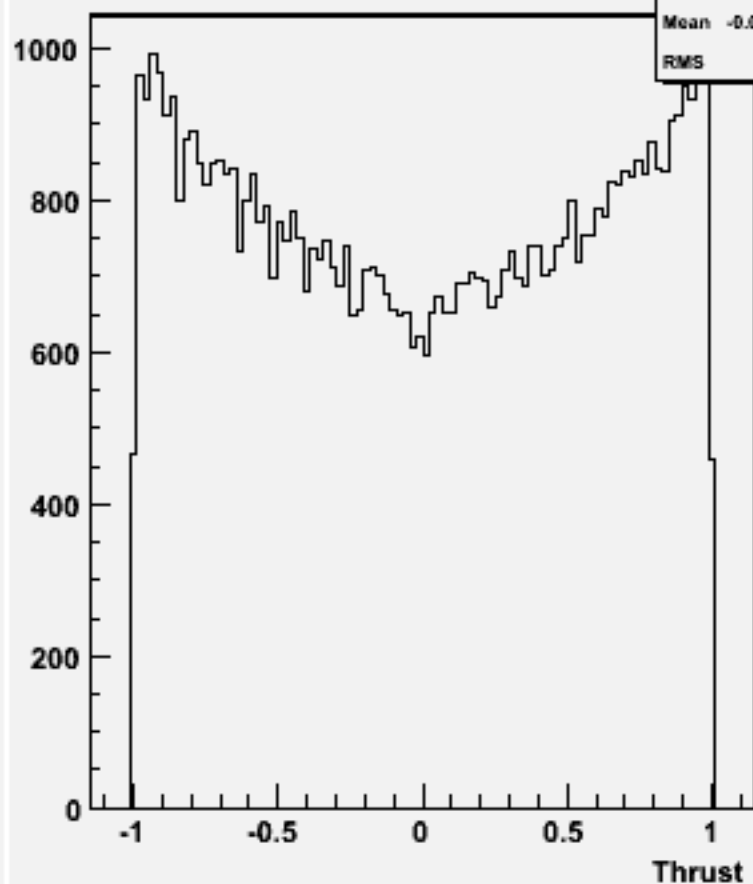
cos \Theta (thrust) w104433 ddh_o
