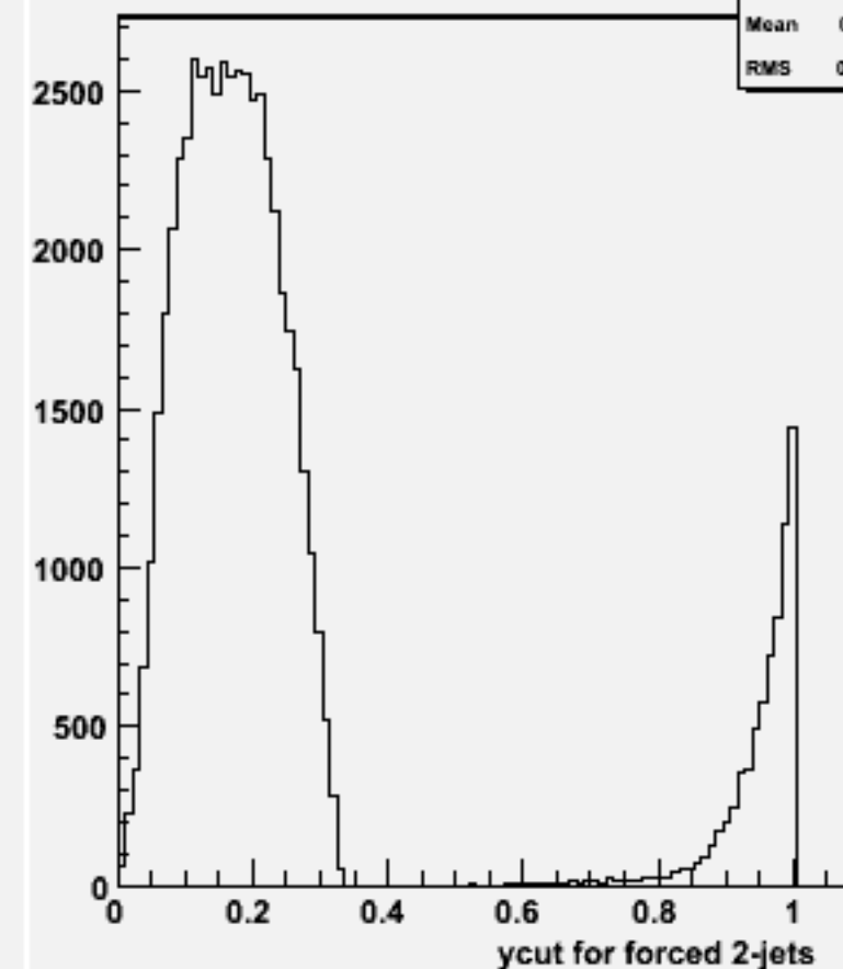
Ycut for 2-jets :w104433 ddh_o
