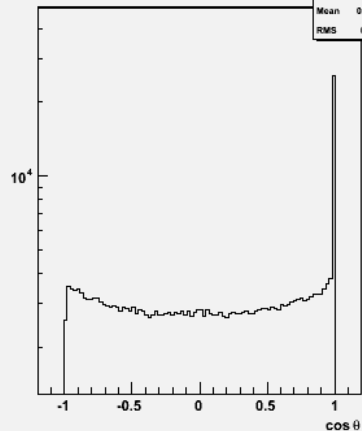
Jet cos \theta (All jets)w104433 ddh_o
