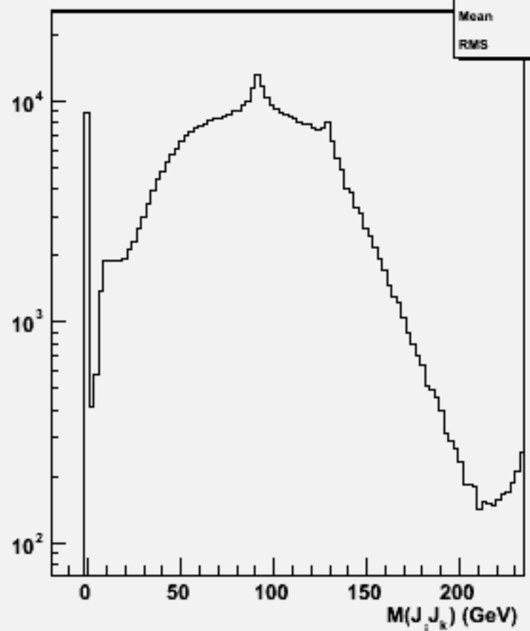
2jets mass(All comb)w104433 ddh_o
