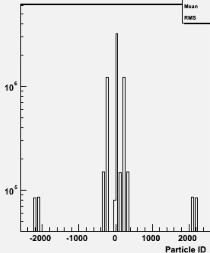
Particle ID : w104433 ddh_o
