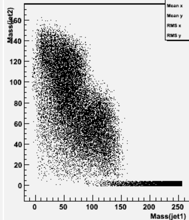
Jet mass for forced 2-jets : w104433 ddh_o
