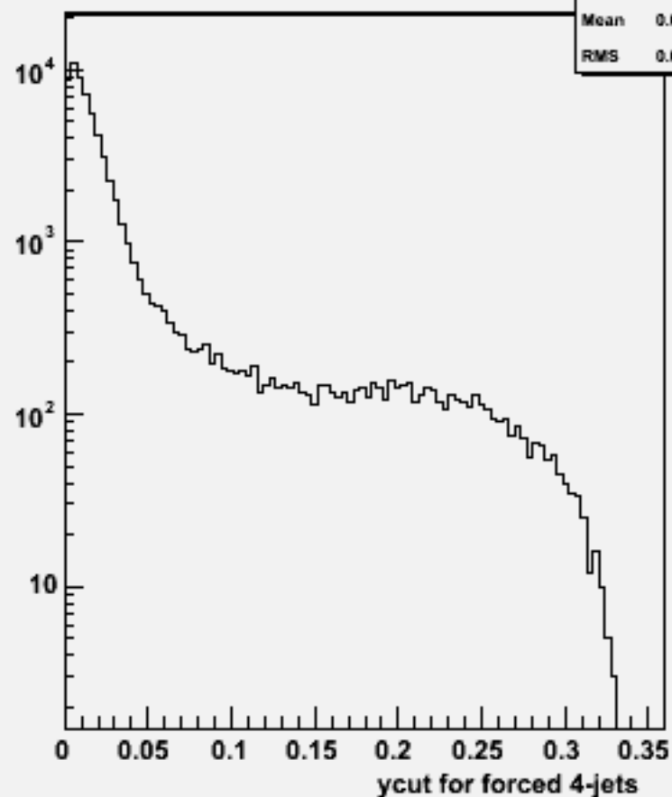
Ycut for 4-jets :w104433 ddh_o
