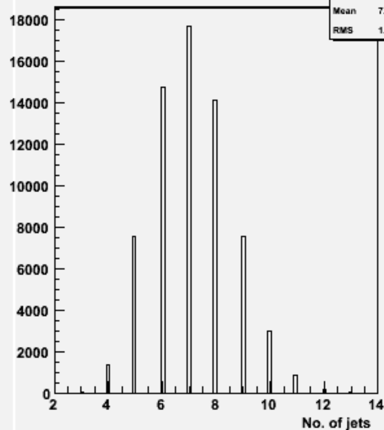
No. jets (ycut=0.001) : w104433 ddh_o
