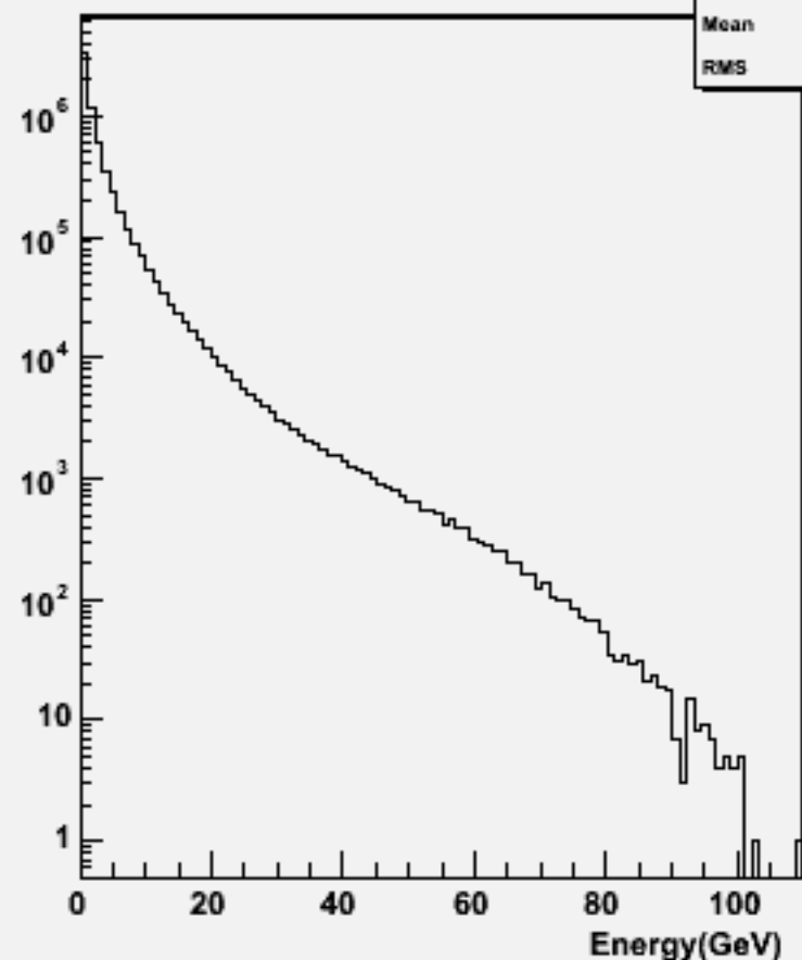
Particle Energy : w104433 ddh_o
