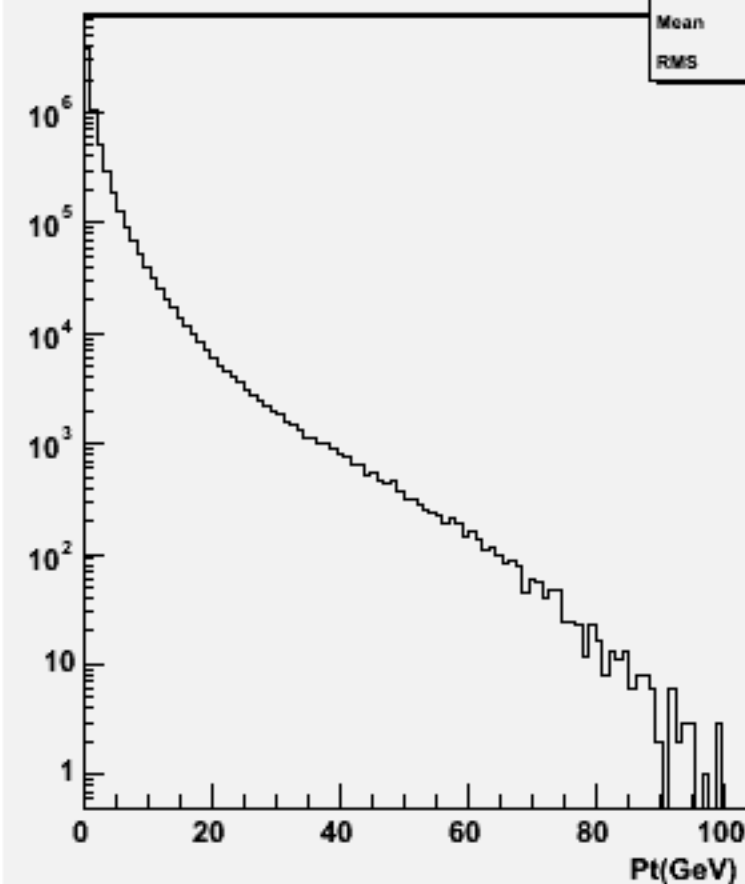
Particle Pt : w104433 ddh_o
