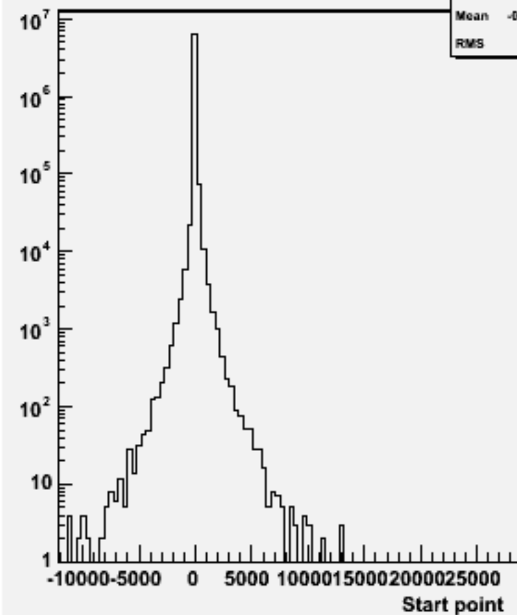
Start point Z : w104433 ddh_o
