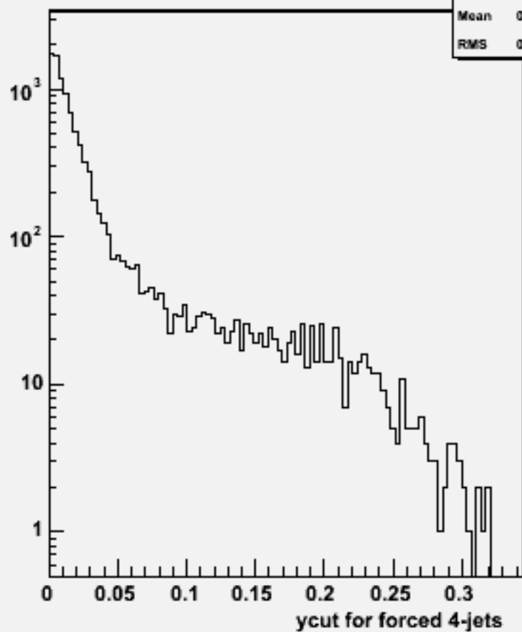
Ycut for 4-jets :w104430 e3e3h_o
