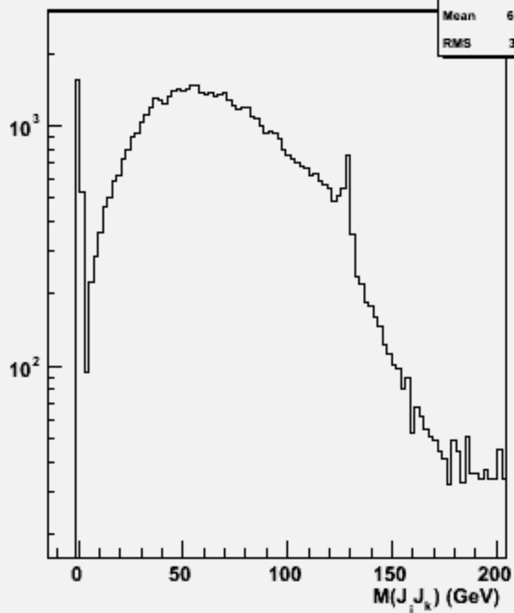
2jets mass(All comb)w104430 e3e3h_o
