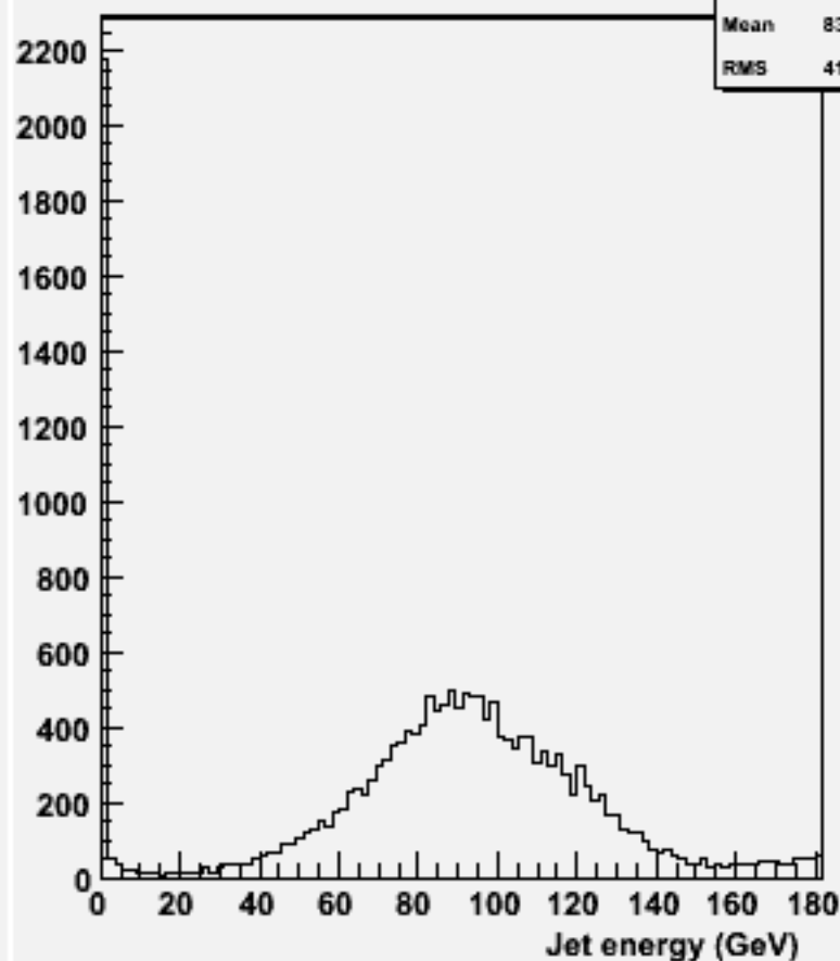
energy for 2-jets :w104430 e3e3h_o
