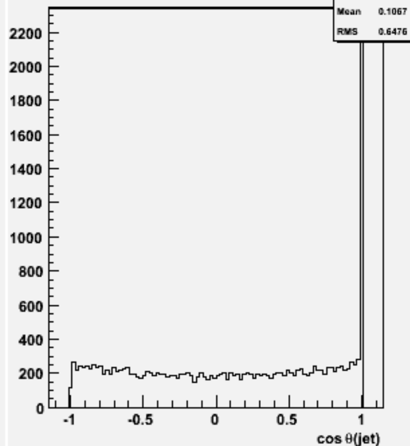
cos \theta for 2-jets :w104430 e3e3h_o
