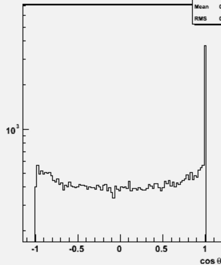
Jet cos \theta (All jets)w104430 e3e3h_o
