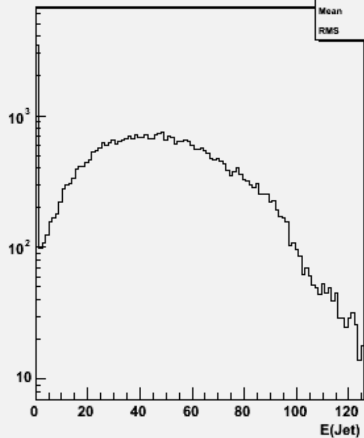
Jet energies(All jets)w104430 e3e3h_o
