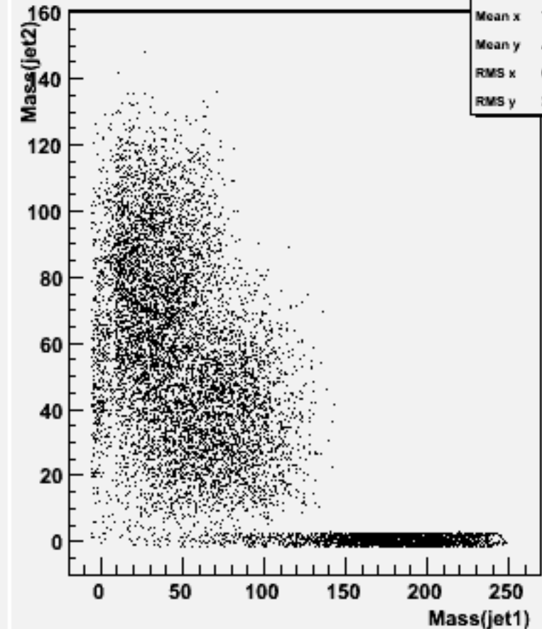
Jet mass for forced 2-jets : w104430 e3e3h_o
