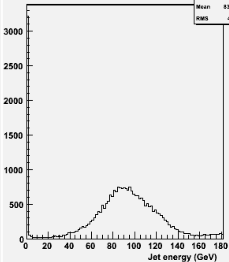
energy for 2-jets :w104429 e3e3h_o
