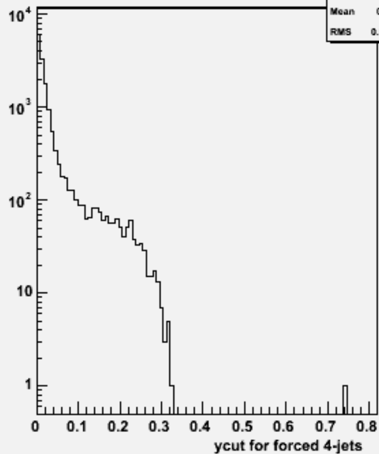
Ycut for 4-jets :w104429 e3e3h_o
