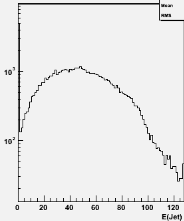
Jet energies(All jets)w104429 e3e3h_o
