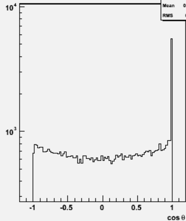
Jet cos \theta (All jets)w104429 e3e3h_o
