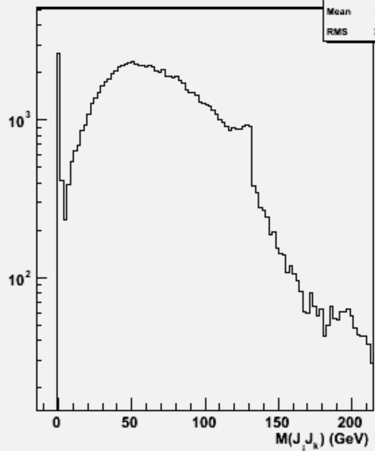
2jets mass(All comb)w104429 e3e3h_o
