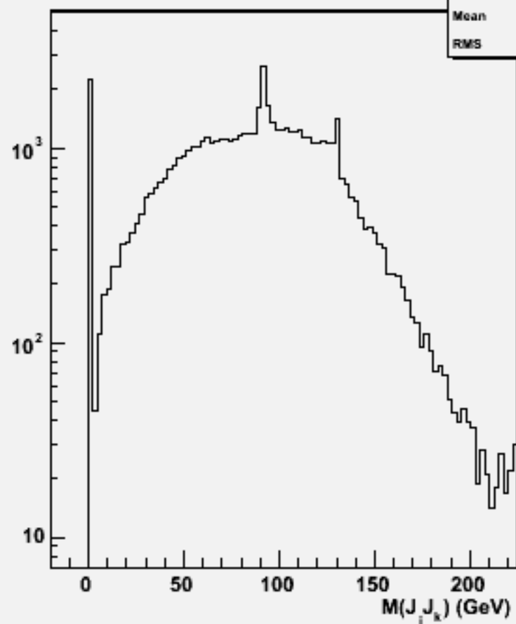
2jets mass(All comb)w104426 e2e2h_o
