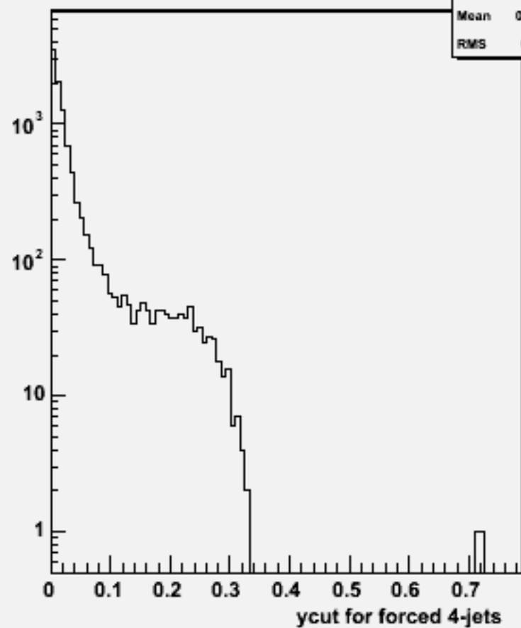
Ycut for 4-jets :w104426 e2e2h_o
