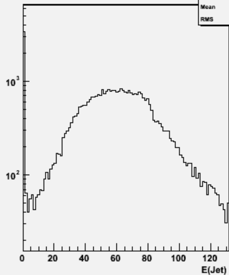
Jet energies(All jets)w104426 e2e2h_o
