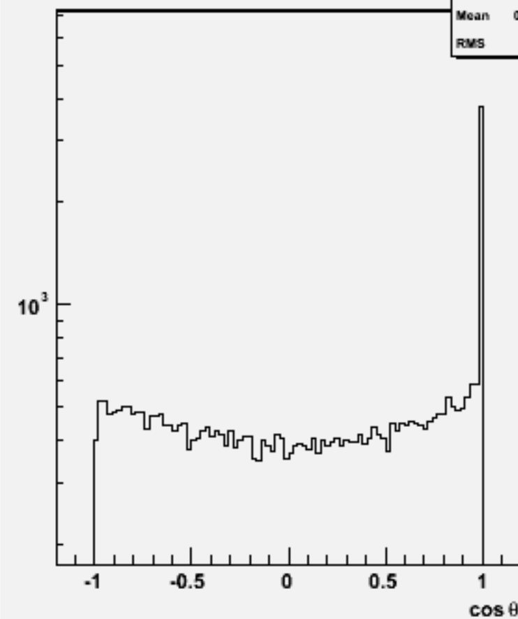
Jet cos \theta (All jets)w104426 e2e2h_o
