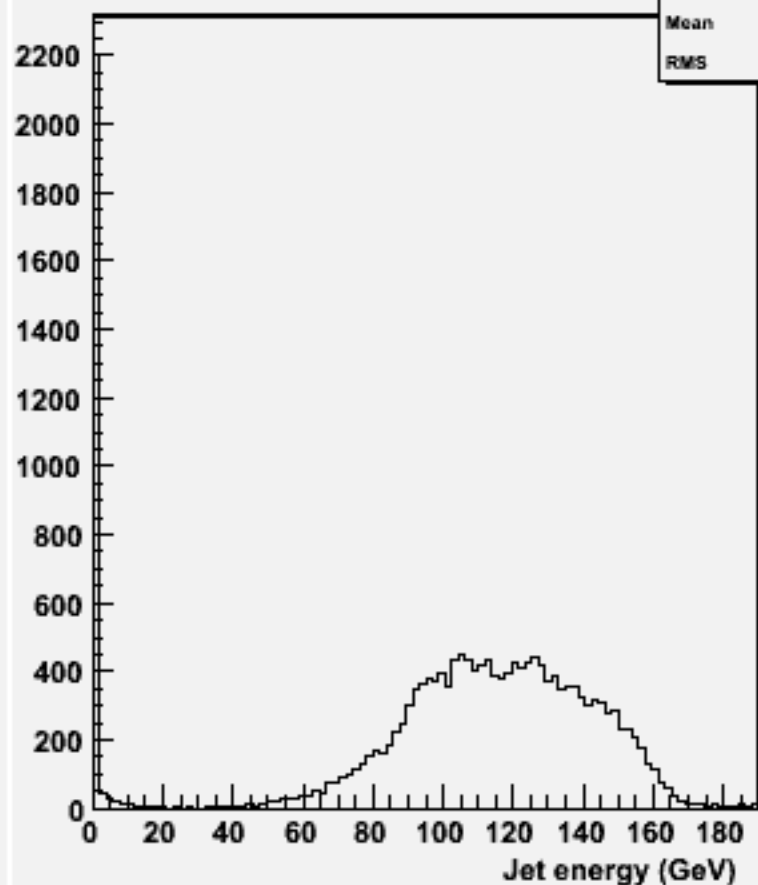
energy for 2-jets :w104426 e2e2h_o
