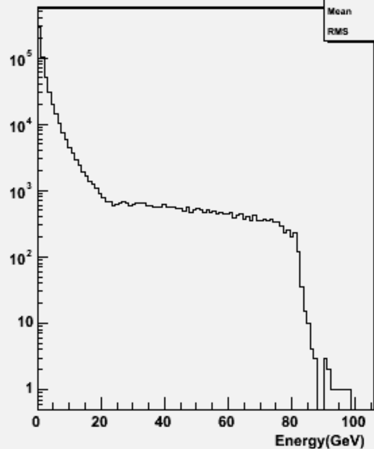
Particle Energy : w104426 e2e2h_o
