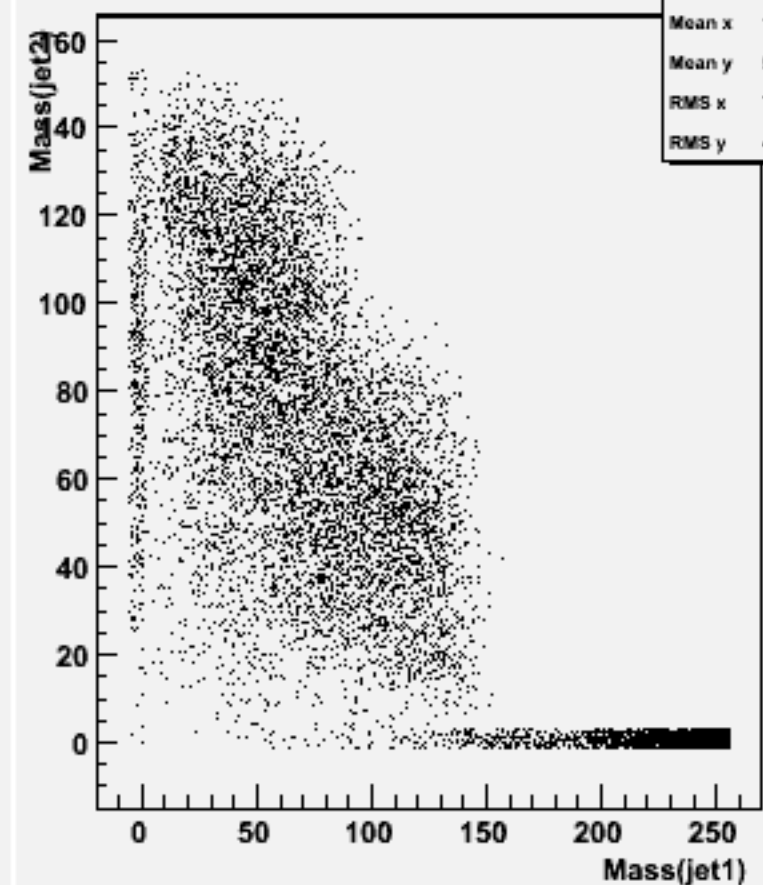
Jet mass for forced 2-jets : w104426 e2e2h_o
