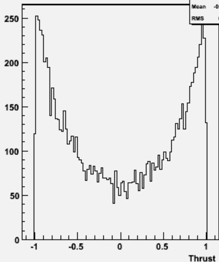
cos \Theta (thrust) w104423 e1e1h_o
