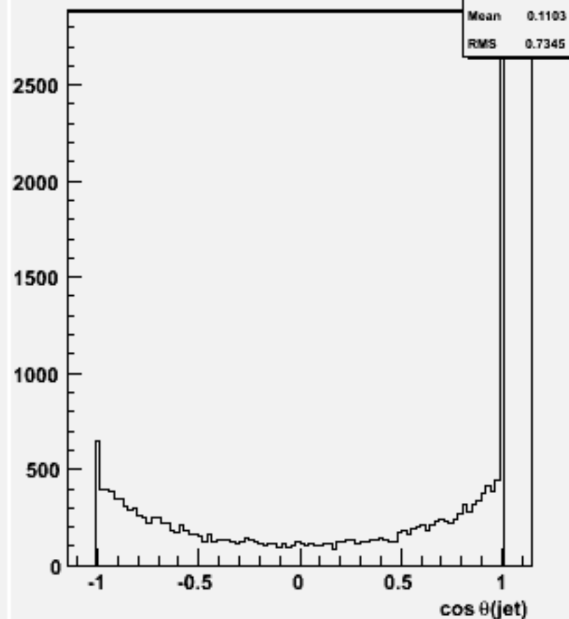
cos \theta for 2-jets :w104423 e1e1h_o
