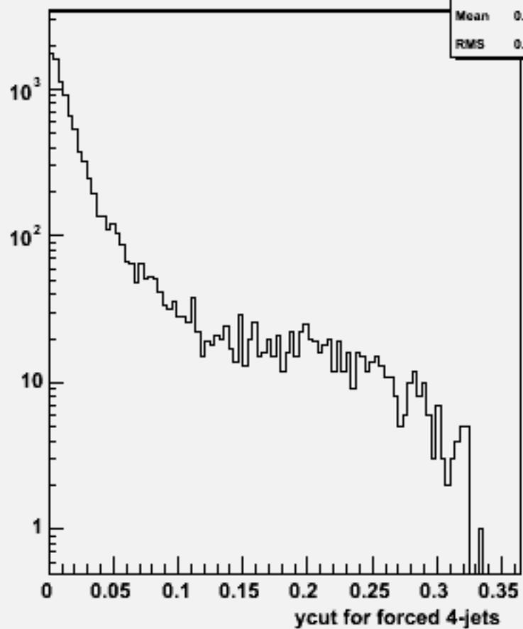
Ycut for 4-jets :w104423 e1e1h_o
