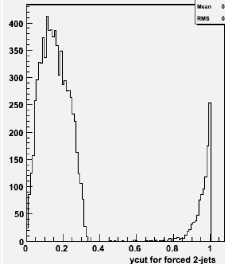
Ycut for 2-jets :w104423 e1e1h_o
