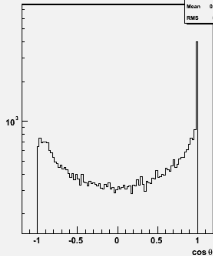
Jet cos \theta (All jets)w104423 e1e1h_o
