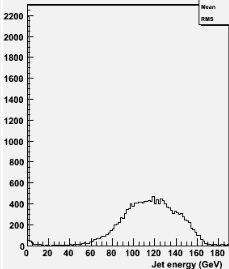
energy for 2-jets :w104423 e1e1h_o
