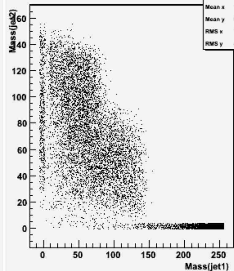
Jet mass for forced 2-jets : w104423 e1e1h_o
