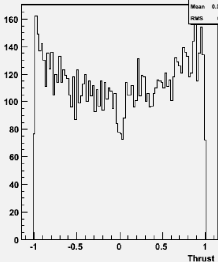
cos \Theta (thrust) w104422 e1e1h_o
