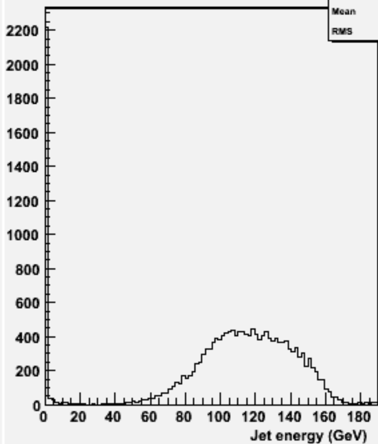
energy for 2-jets :w104422 e1e1h_o
