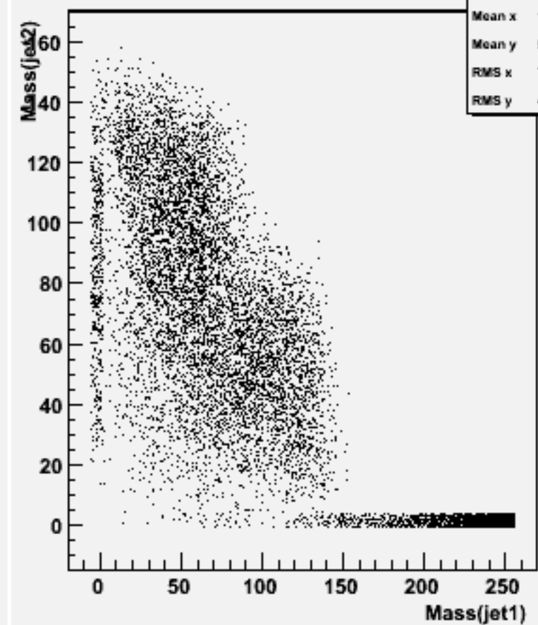
Jet mass for forced 2-jets : w104422 e1e1h_o
