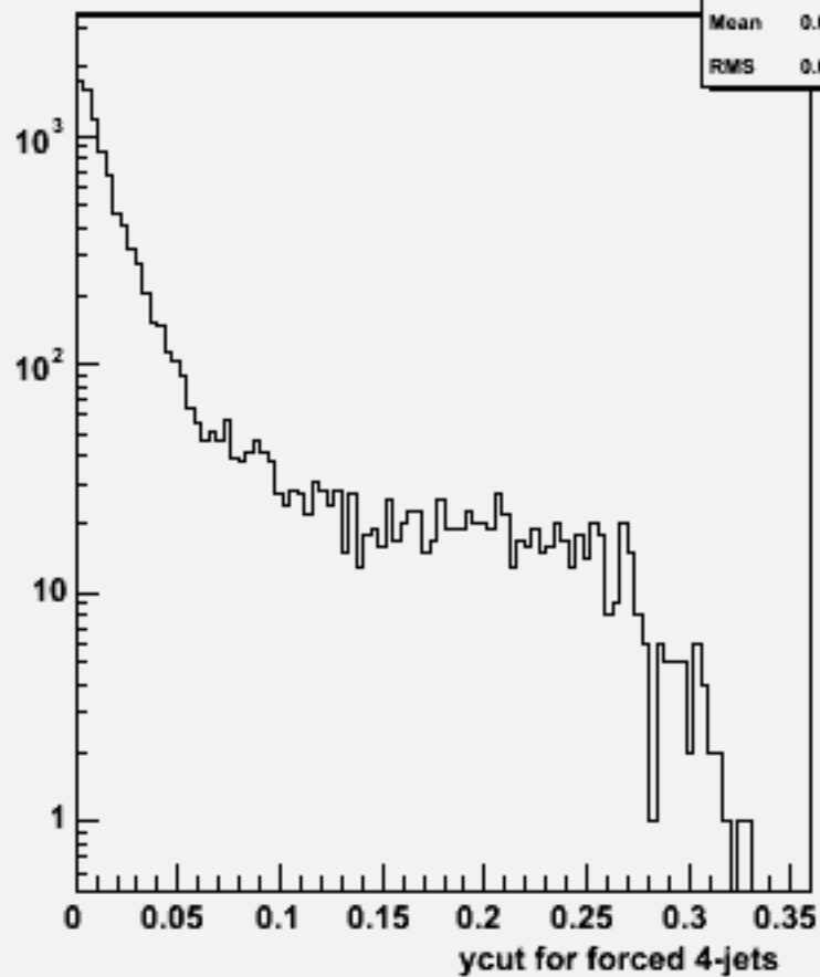
Ycut for 4-jets :w104422 e1e1h_o
