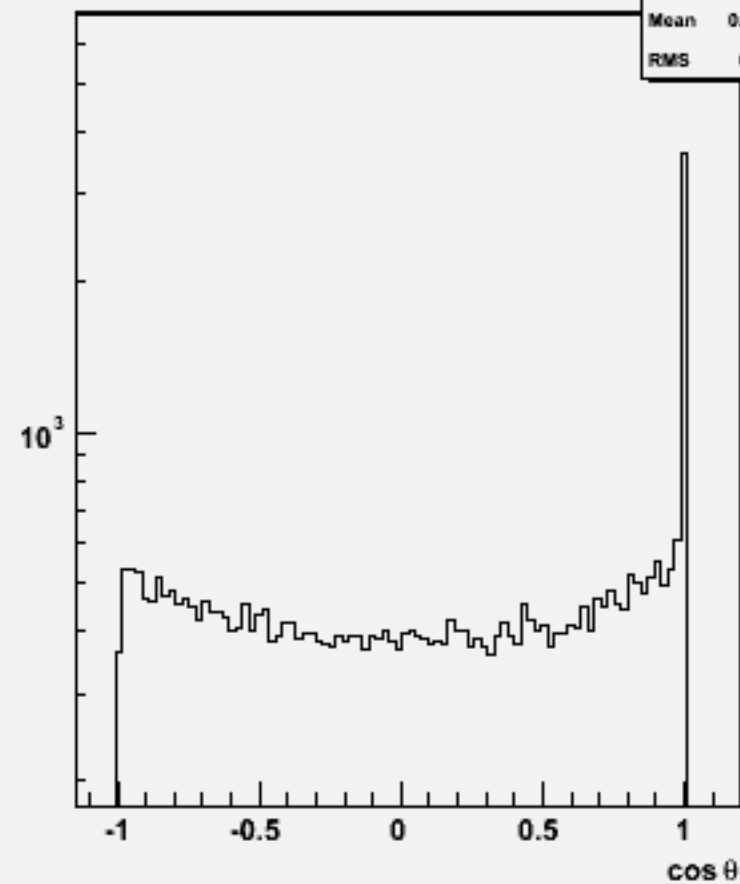
Jet cos \theta (All jets)w104422 e1e1h_o
