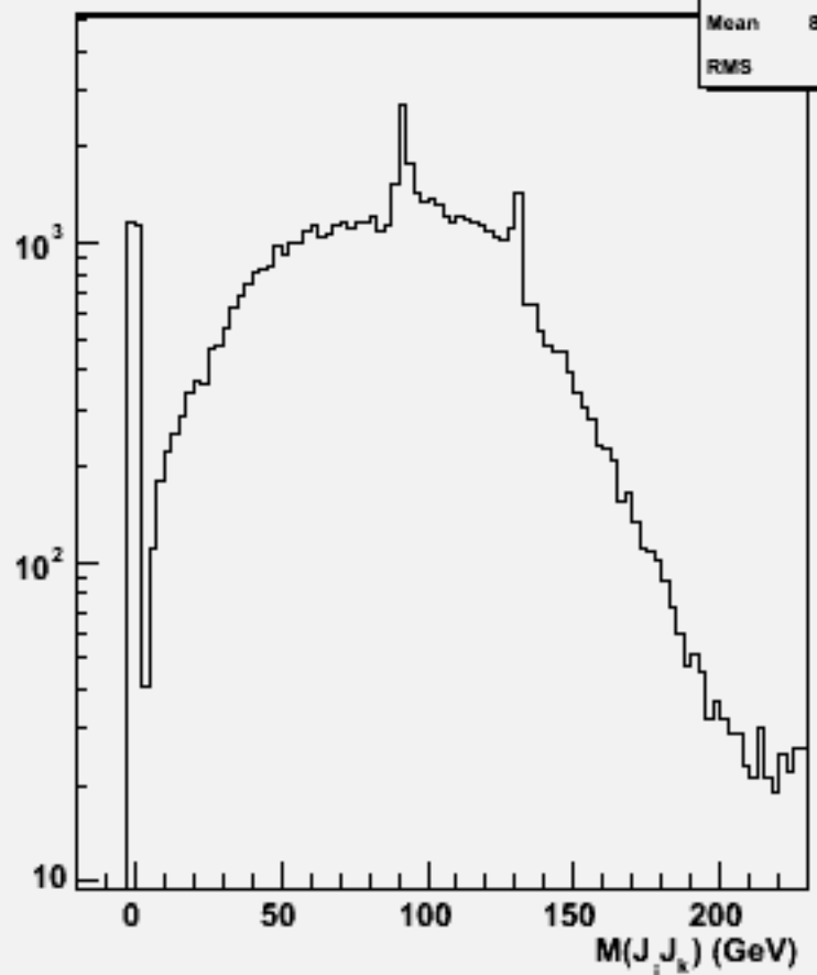
2jets mass(All comb)w104422 e1e1h_o
