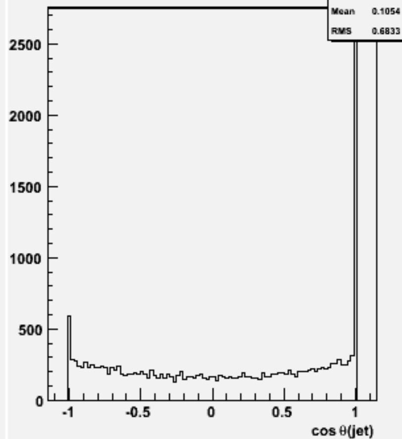
cos \theta for 2-jets :w104422 e1e1h_o
