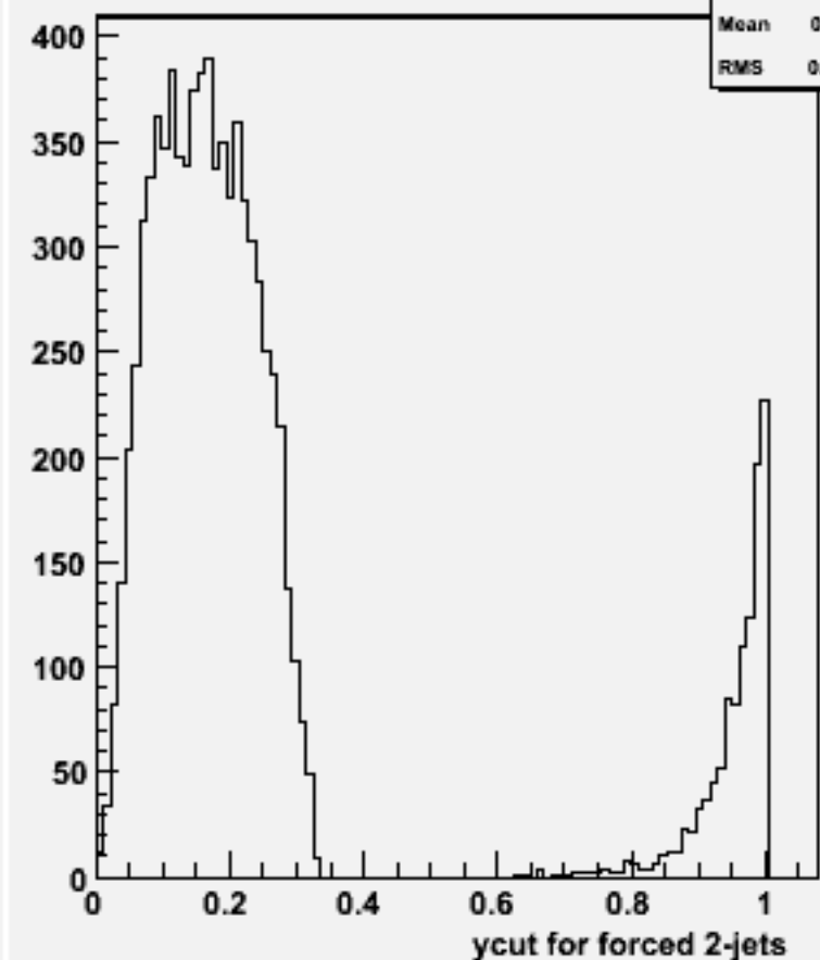
Ycut for 2-jets :w104422 e1e1h_o
