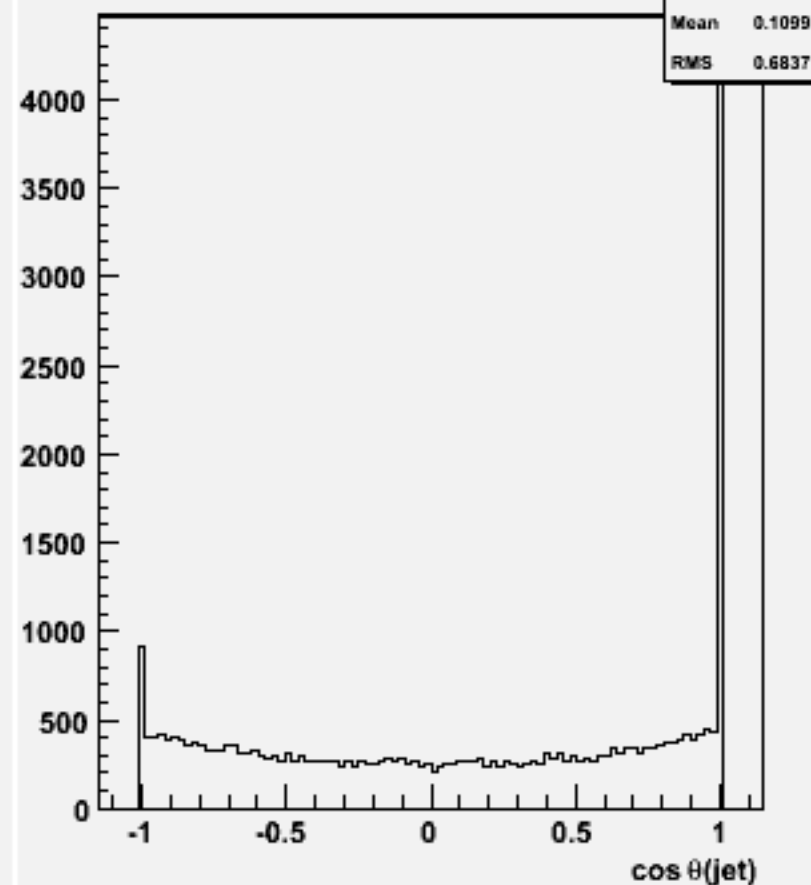
cos \theta for 2-jets :w104421 e1e1h_o
