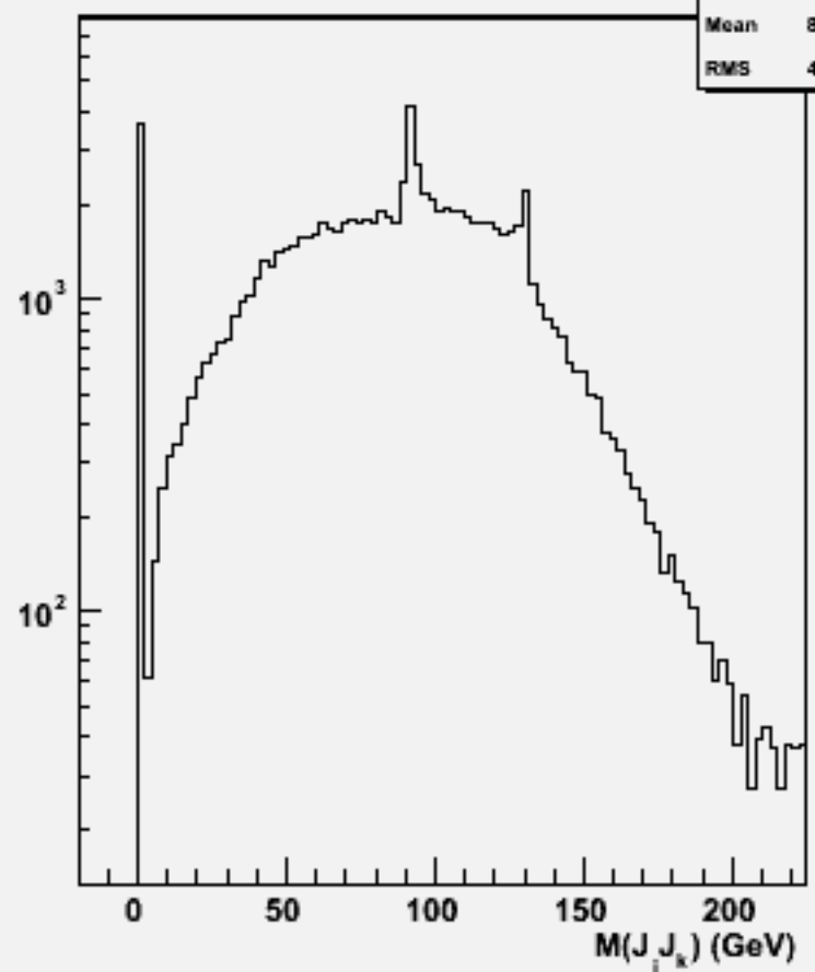
2jets mass(All comb)w104421 e1e1h_o
