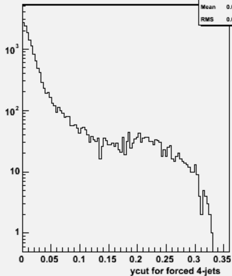
Ycut for 4-jets :w104421 e1e1h_o
