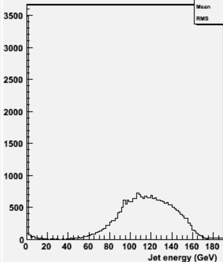
energy for 2-jets :w104421 e1e1h_o
