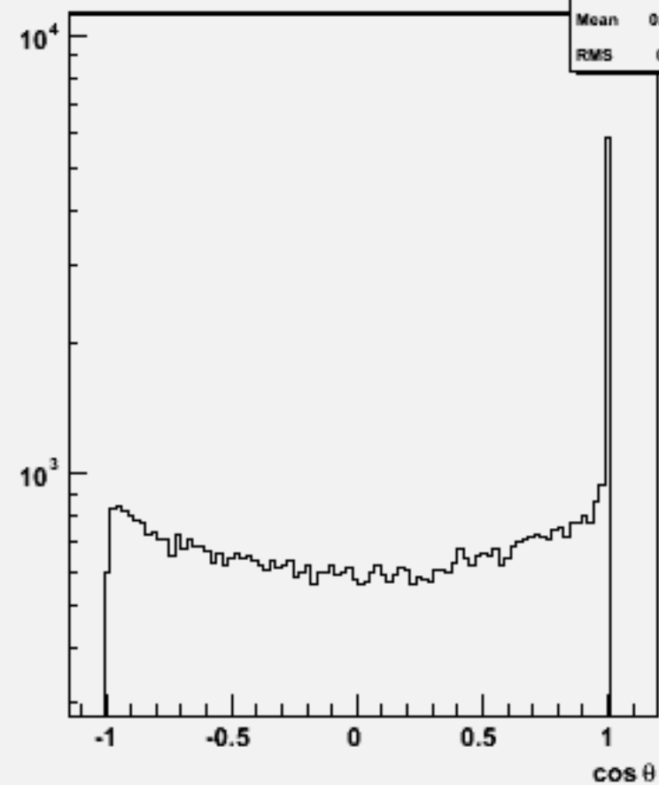
Jet cos \theta (All jets)w104421 e1e1h_o
