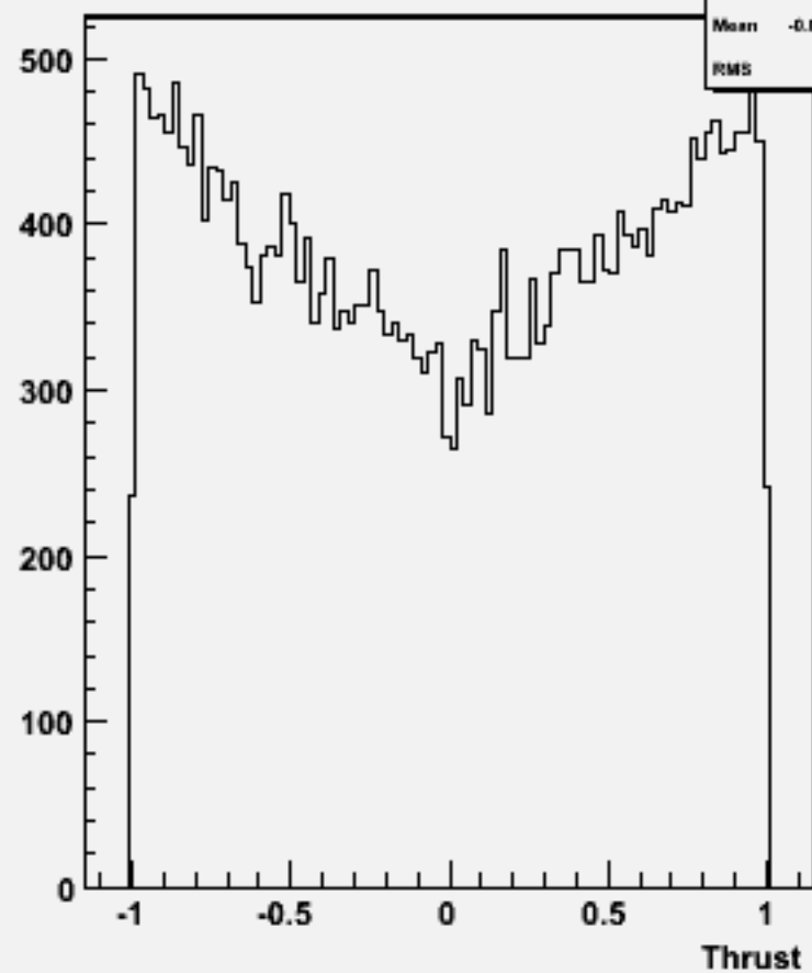
cos \Theta (thrust) w104418 cch_o
