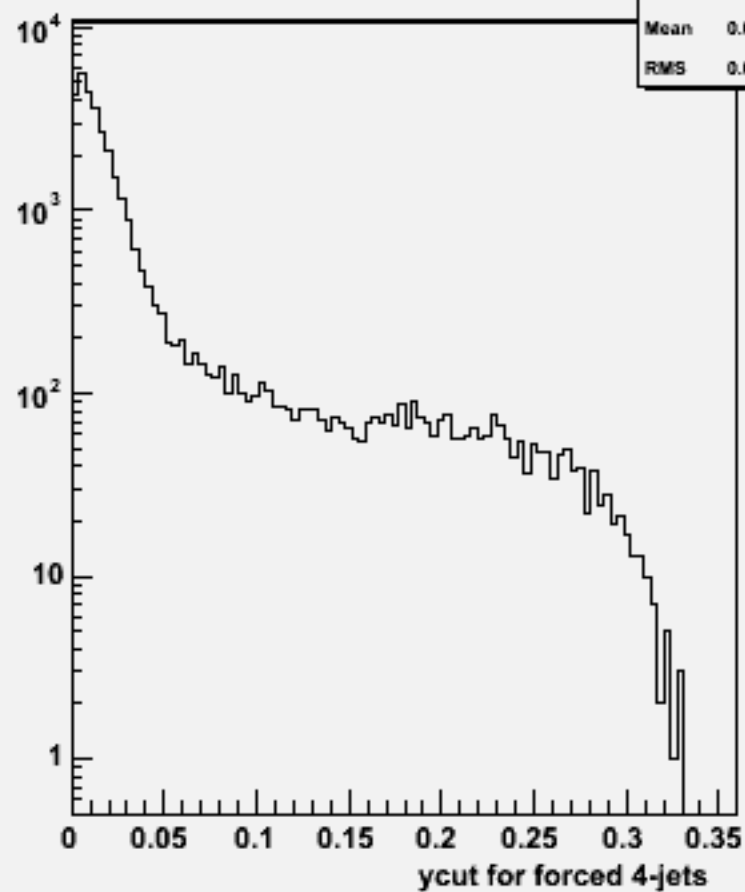
Ycut for 4-jets :w104418 cch_o
