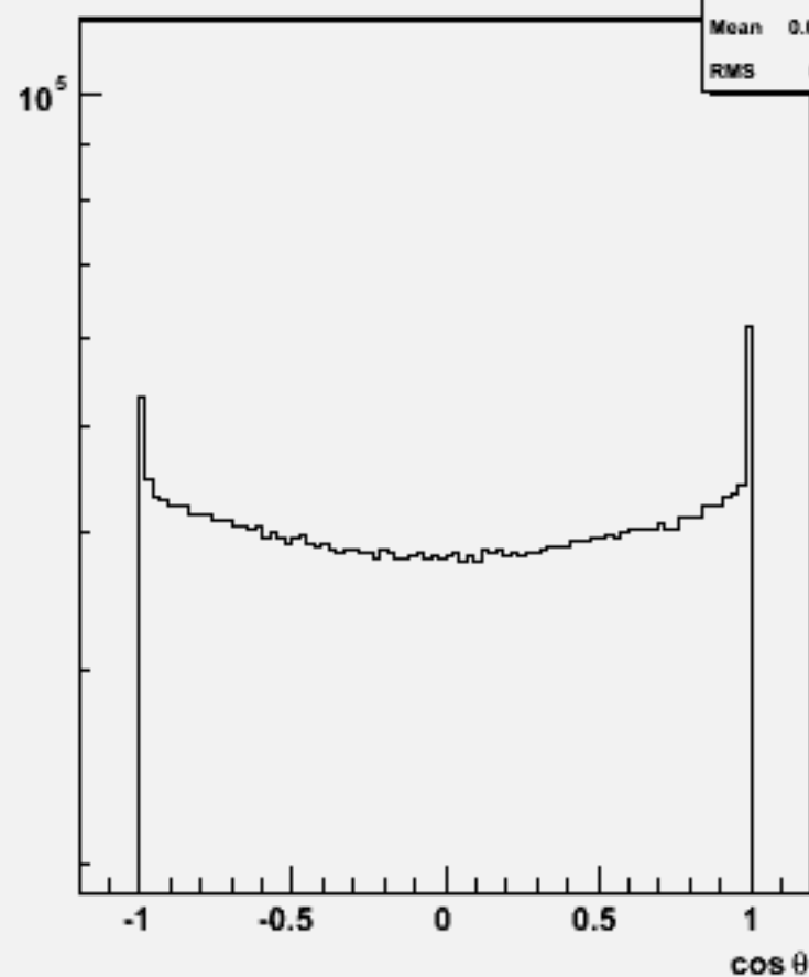
Particle cos \theta : w104418 cch_o
