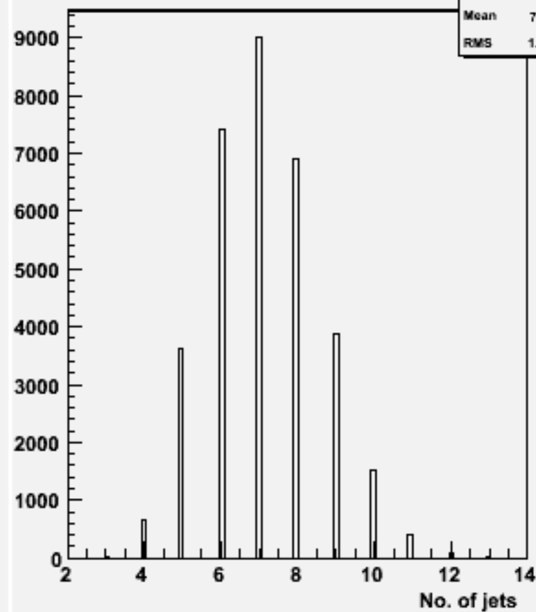
No. jets (ycut=0.001) : w104418 cch_o
