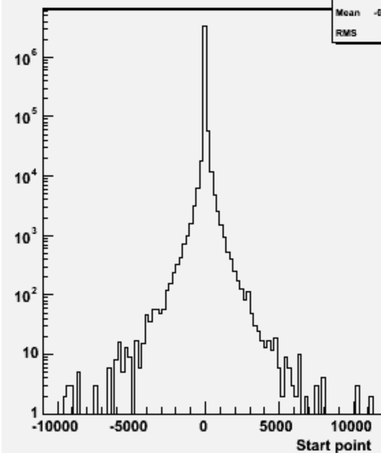
Start point Z : w104418 cch_o
