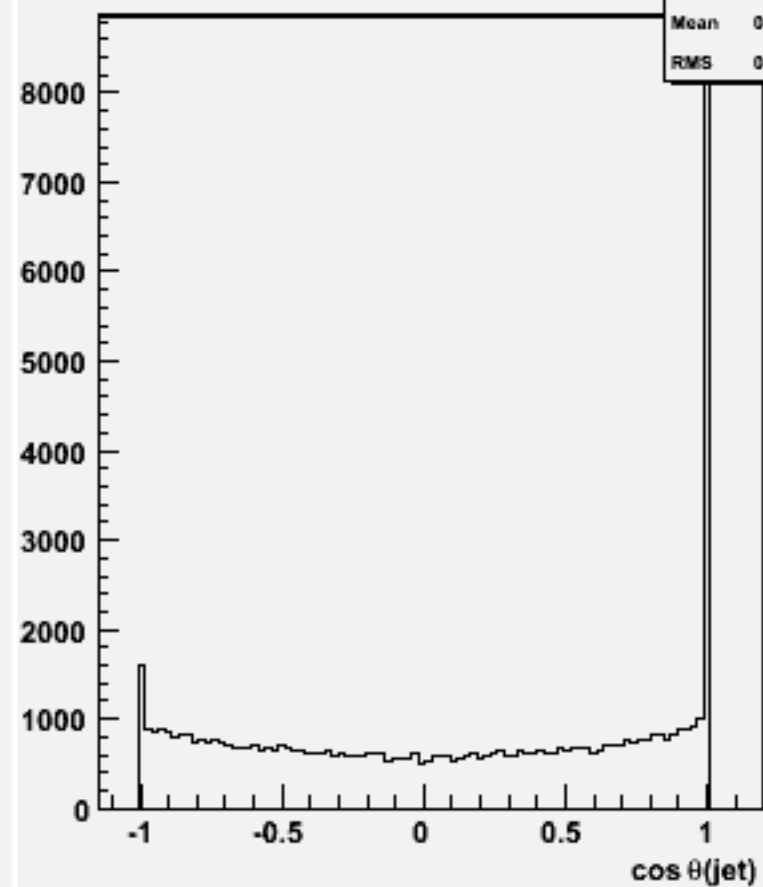
cos \Theta for 2-jets :w104418 cch_o
