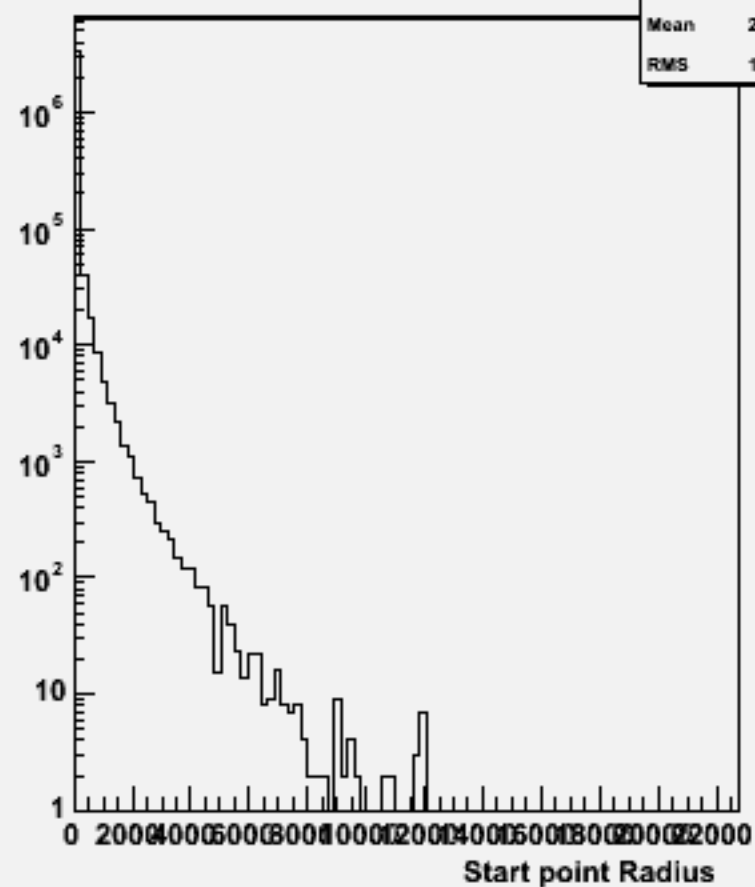
Start point R : w104418 cch_o
