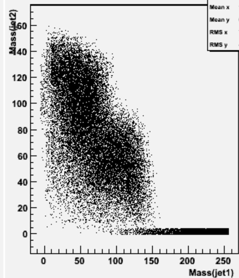
Jet mass for forced 2-jets : w104418 cch_o
