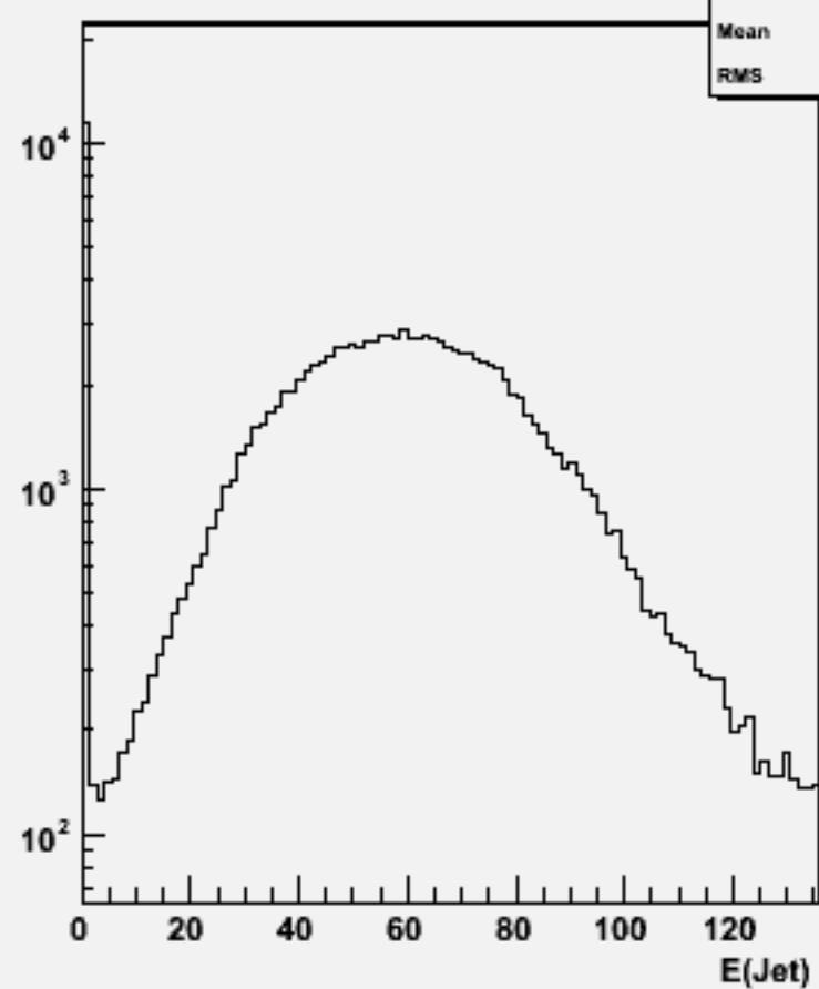
Jet energies(All jets)w104418 cch_o
