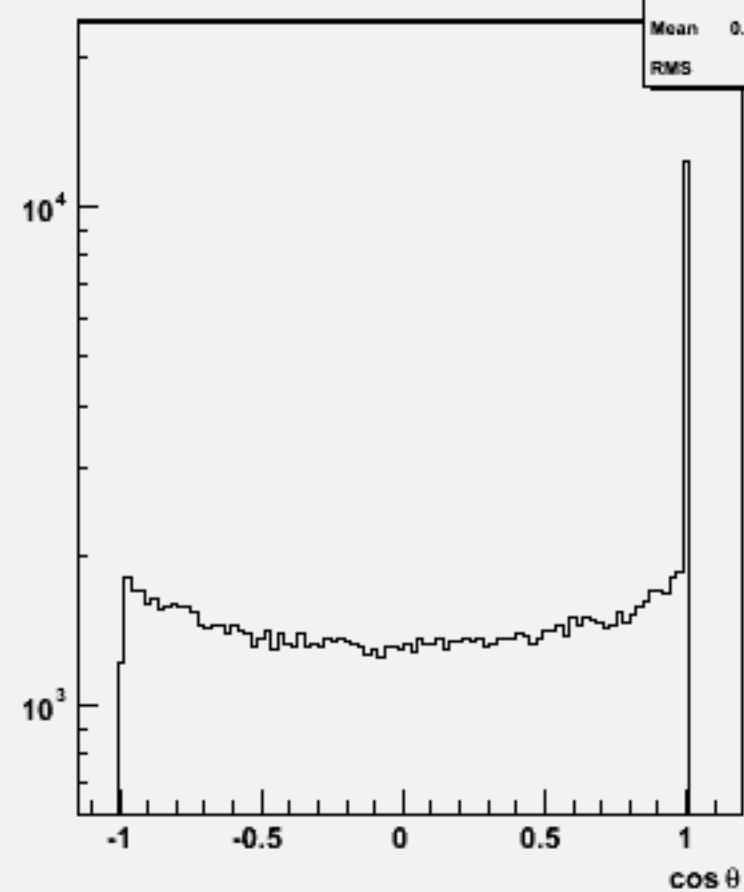
Jet cosθ (All jets)w104418 cch_o
