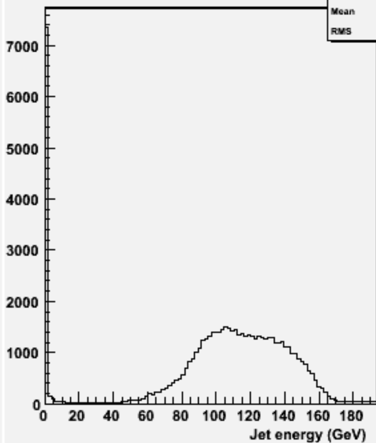
energy for 2-jets :w104418 cch_o
