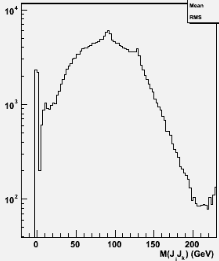
2jets mass(All comb)w104418 cch_o
