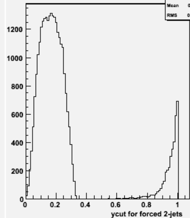
Ycut for 2-jets :w104418 cch_o
