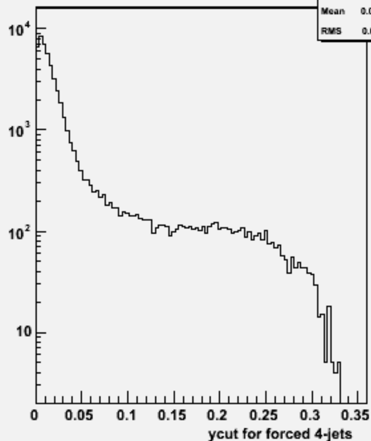
Ycut for 4-jets :w104413 uuh_o
