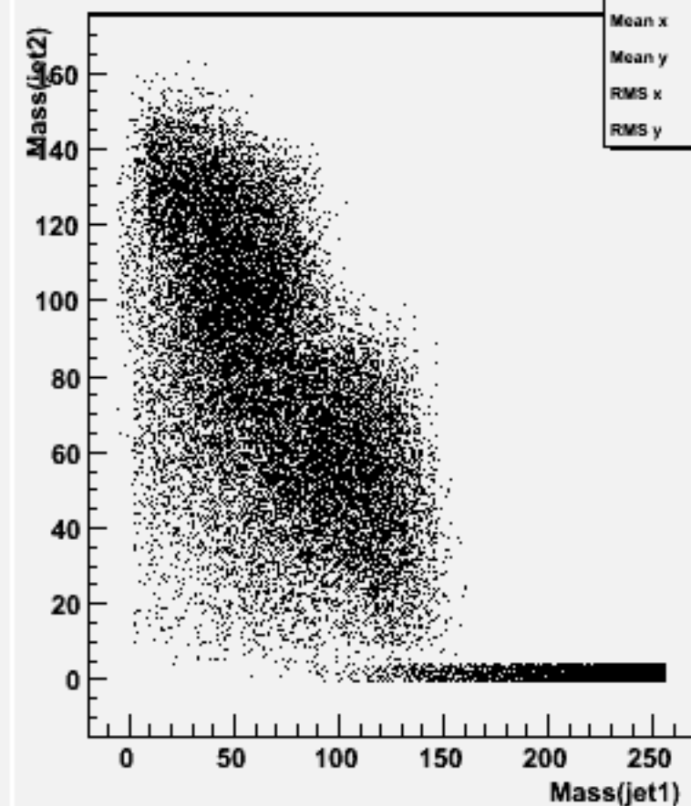
Jet mass for forced 2-jets : w104413 uuh_o
