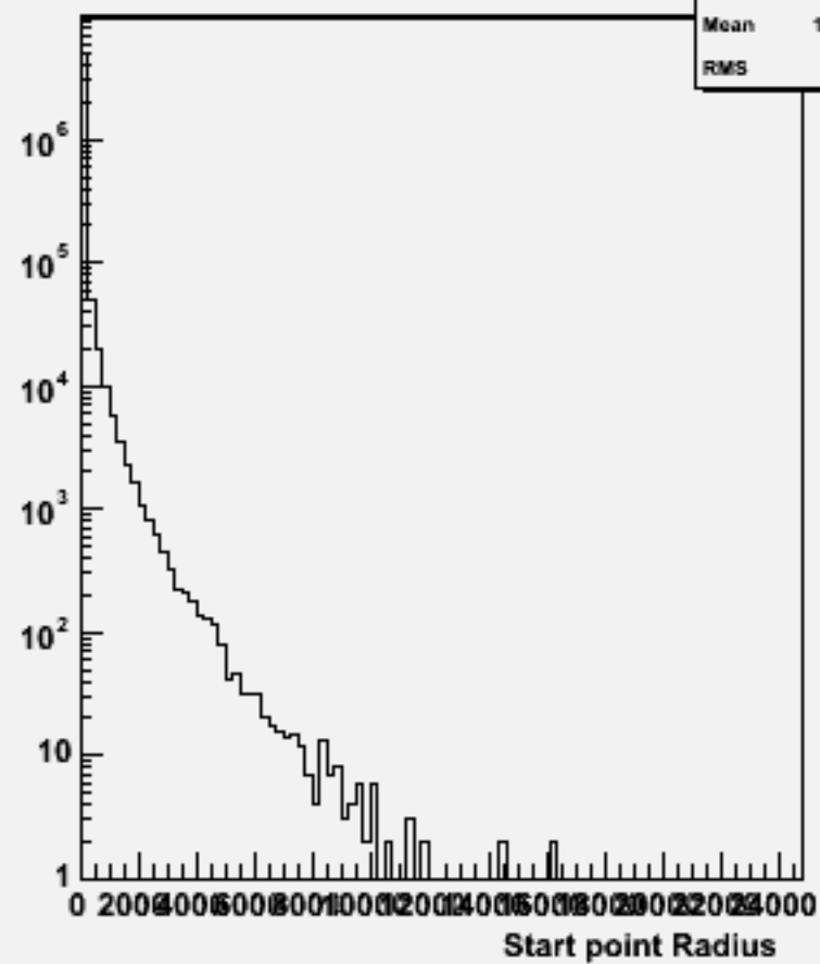
Start point R : w104413 uuh_o
