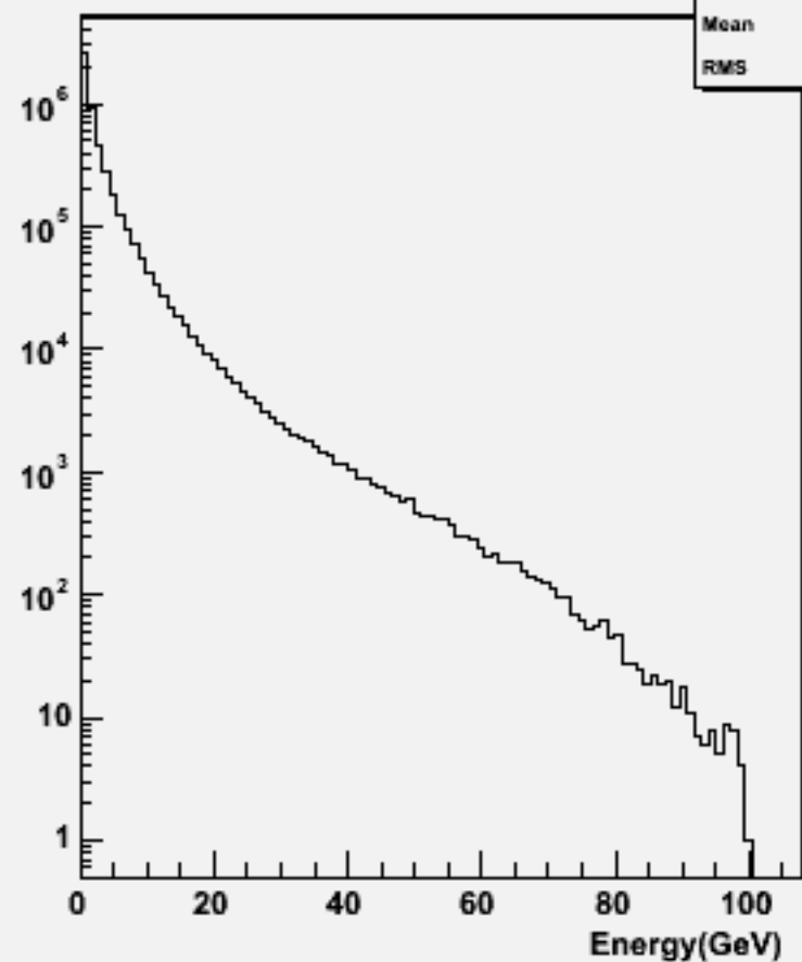
Particle Energy : w104413 uuh_o
