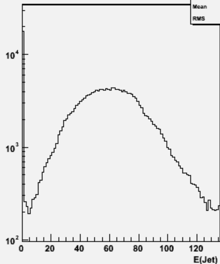
Jet energies(All jets)w104413 uuh_o
