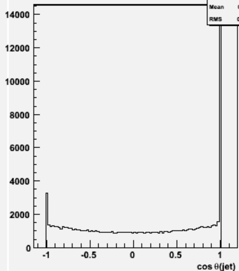
cos \theta for 2-jets :w104413 uuh_o
