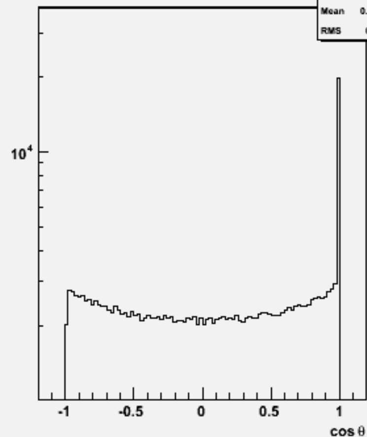
Jet cos \theta (All jets)w104413 uuh_o
