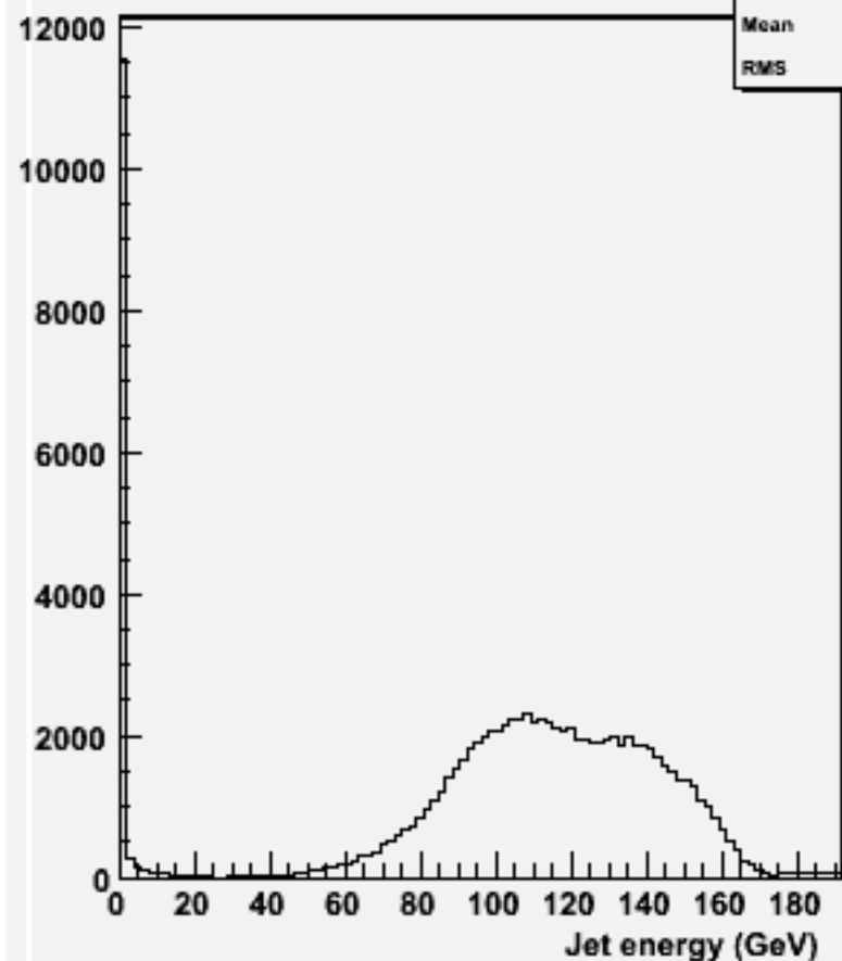
energy for 2-jets :w104413 uuh_o
