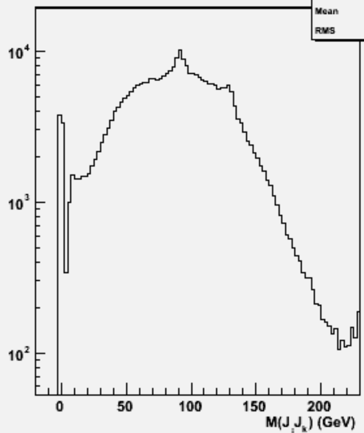
2jets mass(All comb)w104413 uuh_o
