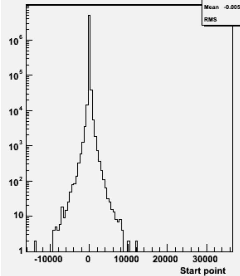
Start point Z : w104413 uuh_o
