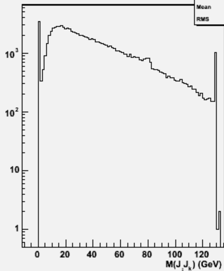
2jets mass(All comb)w104410 n3n3h_o
