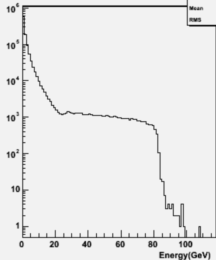
Particle Energy : w104410 n3n3h_o
