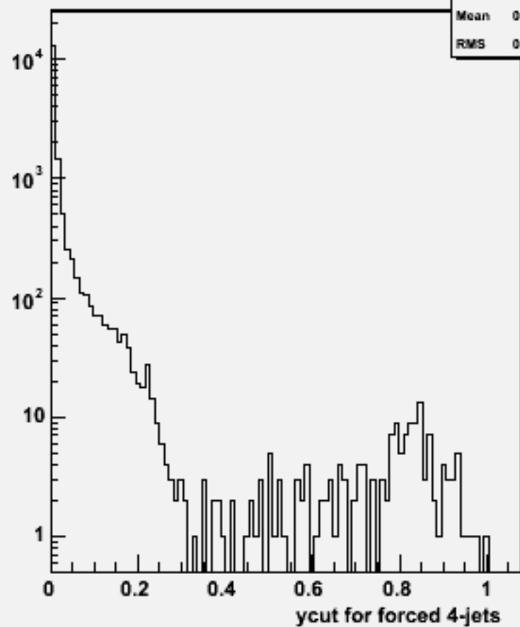
Ycut for 4-jets :w104410 n3n3h_o
