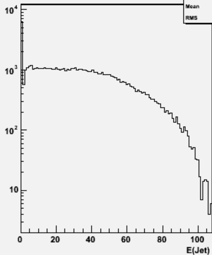
Jet energies(All jets)w104410 n3n3h_o
