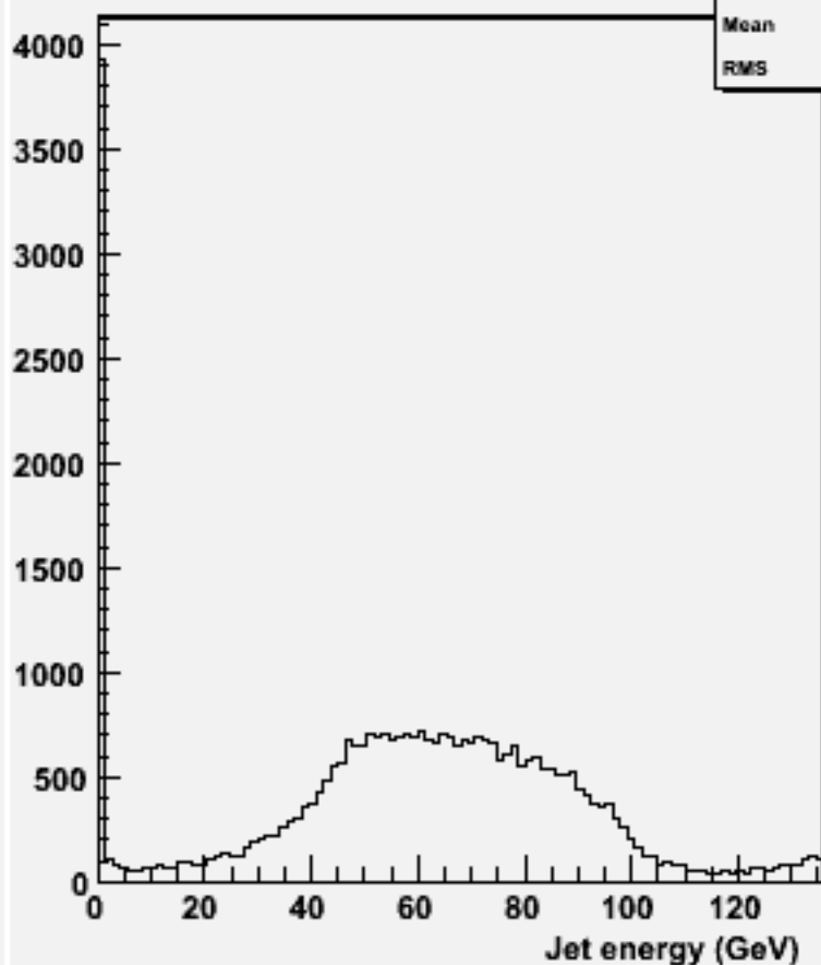
energy for 2-jets :w104410 n3n3h_o
