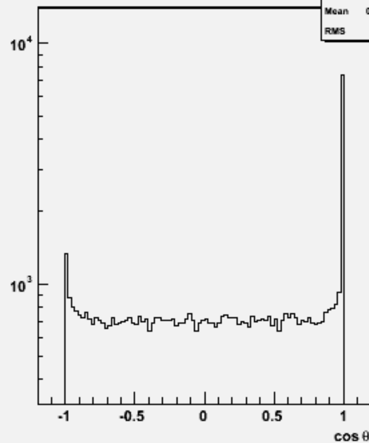
Jet cos \theta (All jets)w104410 n3n3h_o
