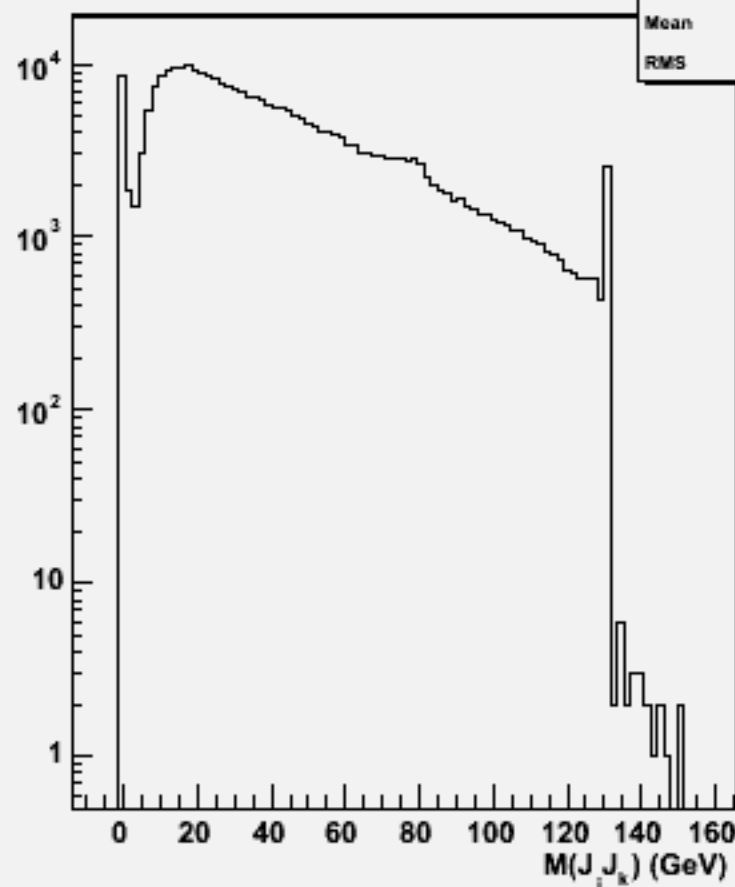
2jets mass(All comb)w104401 n1n1h_o
