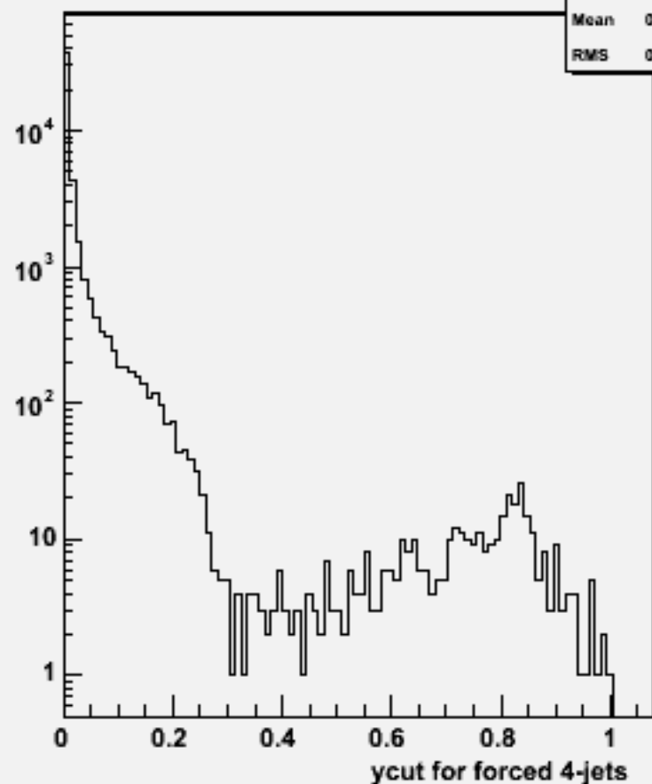
Ycut for 4-jets :w104401 n1n1h_o
