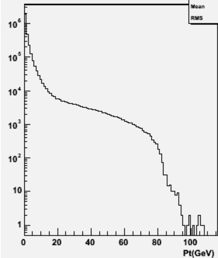
Particle Pt : w104401 n1n1h_o
