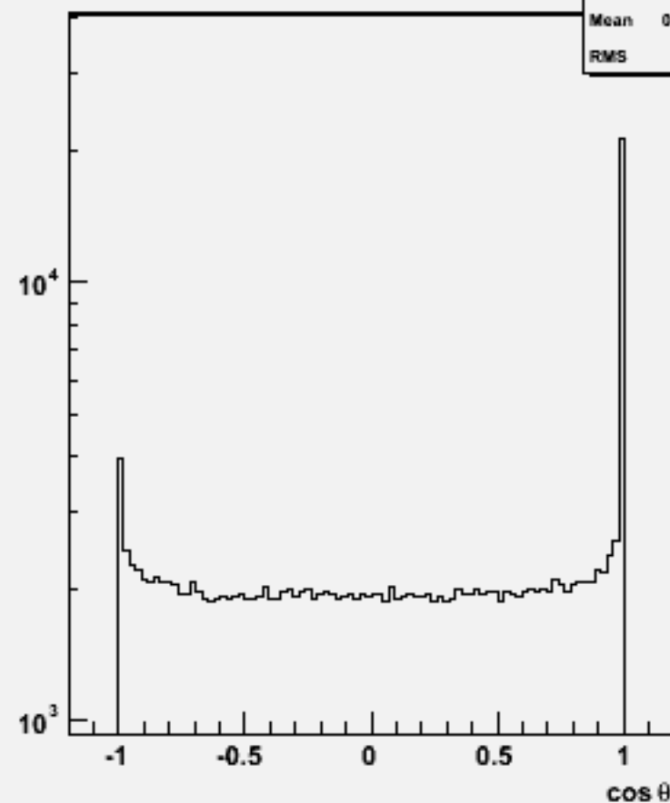
Jet cos \theta (All jets)w104401 n1n1h_o
