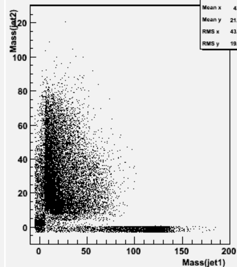
Jet mass for forced 2-jets : w104401 n1n1h_o
