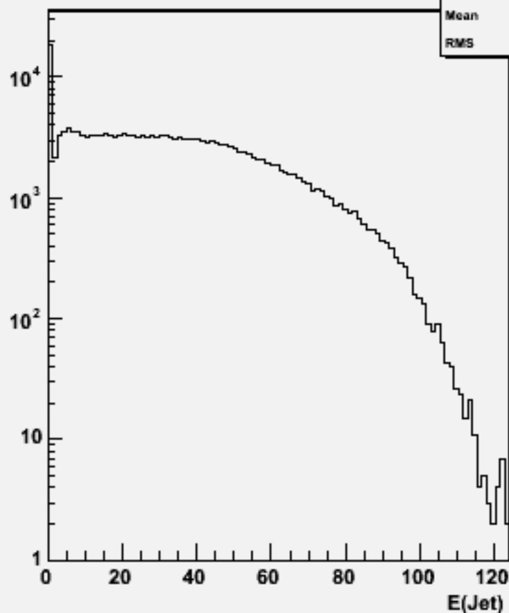
Jet energies(All jets)w104401 n1n1h_o
