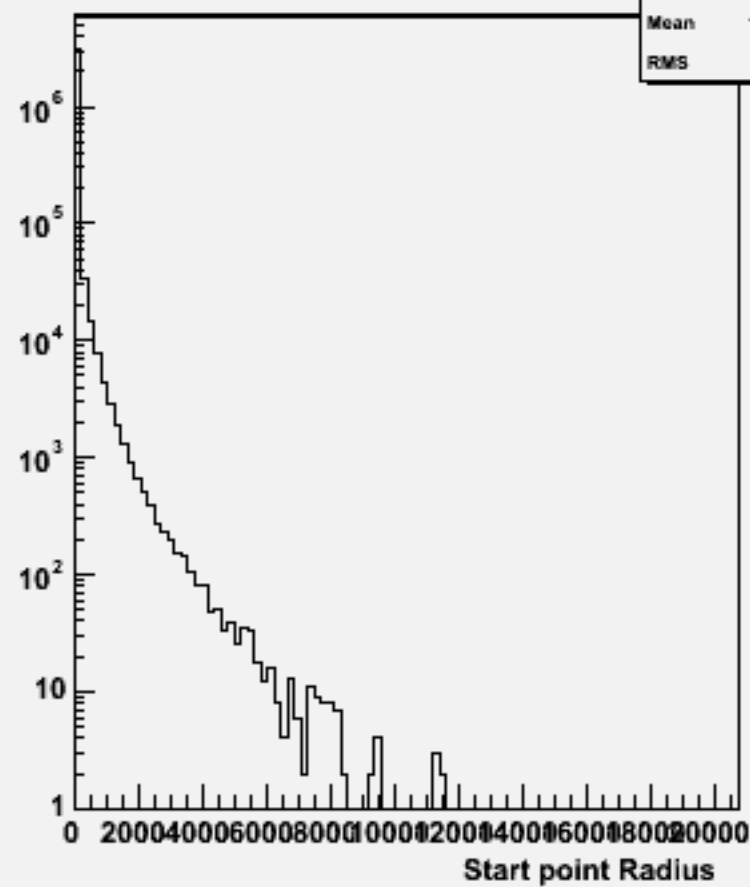
Start point R : w104401 n1n1h_o
