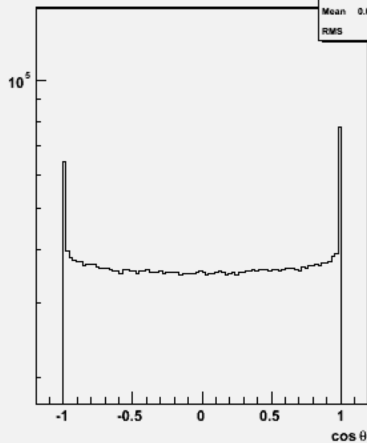
Particle cosθ : w104401 n1n1h_o
