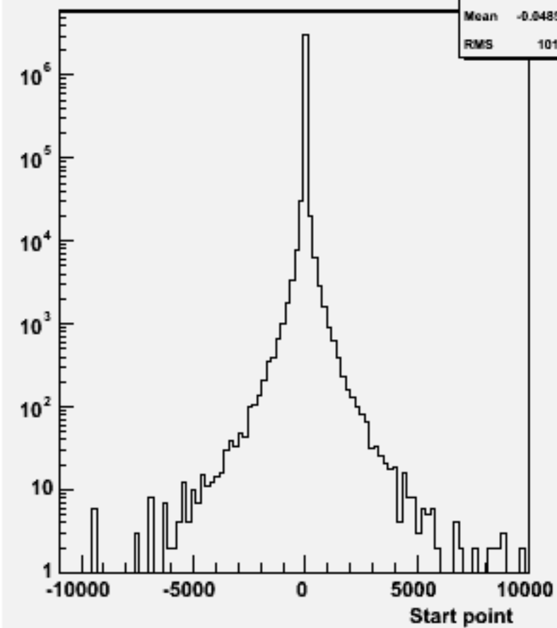
Start point Z : w104401 n1n1h_o
