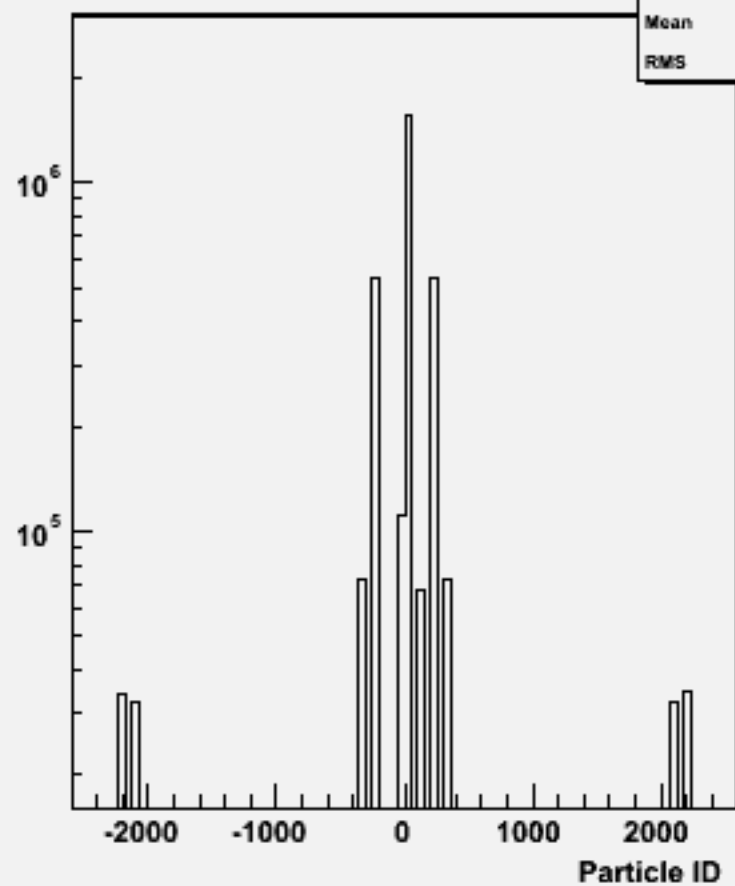
Particle ID : w104401 n1n1h_o
