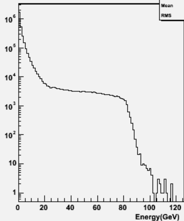
Particle Energy : w104401 n1n1h_o
