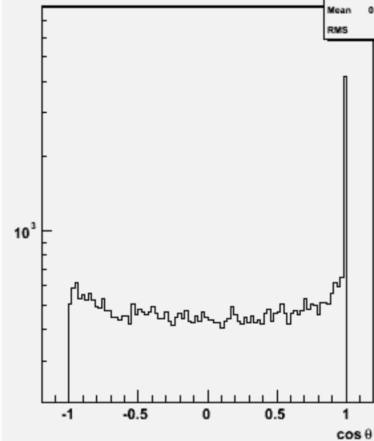
Jet cos \theta (All jets)w104380 e3e3h_o
