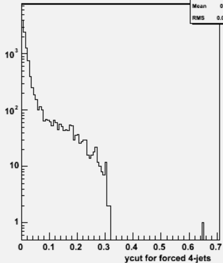
Ycut for 4-jets :w104380 e3e3h_o
