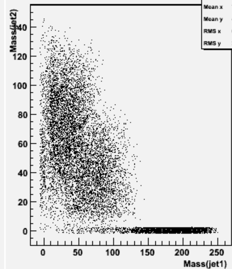
Jet mass for forced 2-jets : w104380 e3e3h_o
