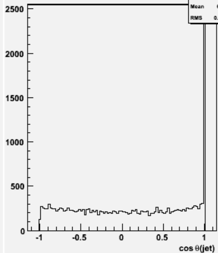
cos \theta for 2-jets :w104380 e3e3h_o
