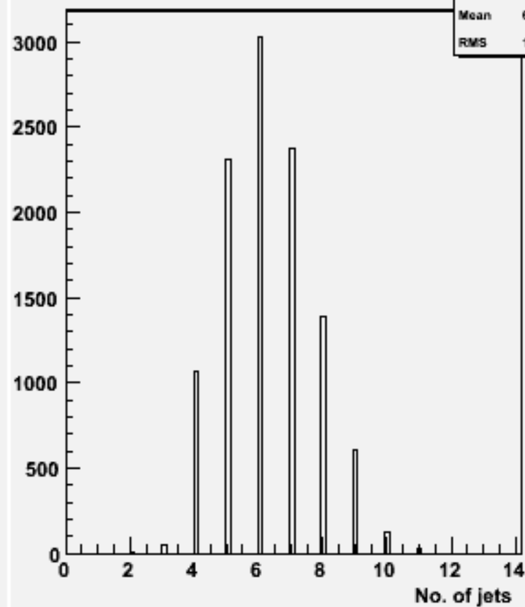
No. jets (ycut=0.001) : w104380 e3e3h_o
