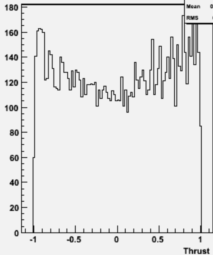
cos \Theta (thrust) w104380 e3e3h_o
