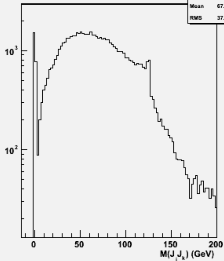
2jets mass(All comb)w104380 e3e3h_o
