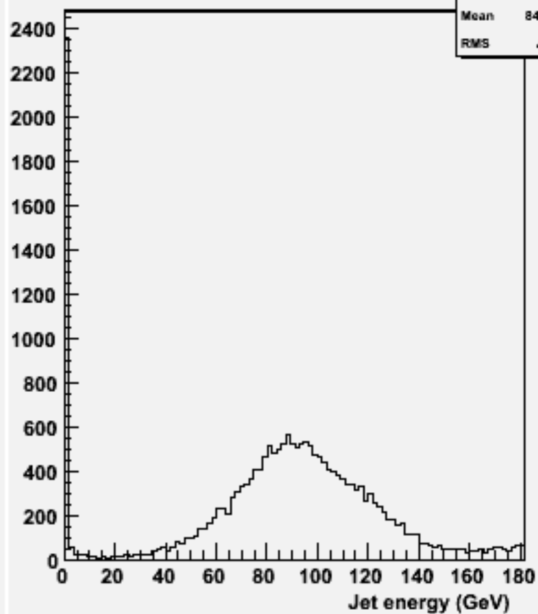
energy for 2-jets :w104380 e3e3h_o
