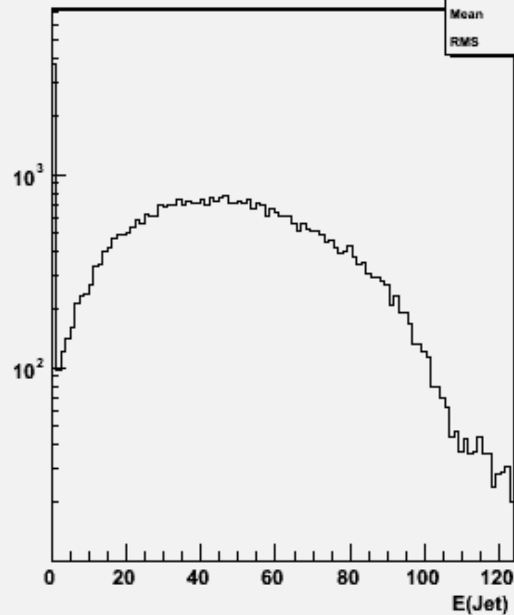
Jet energies(All jets)w104380 e3e3h_o
