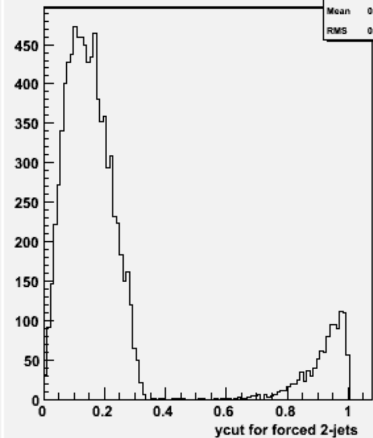
Ycut for 2-jets :w104380 e3e3h_o
