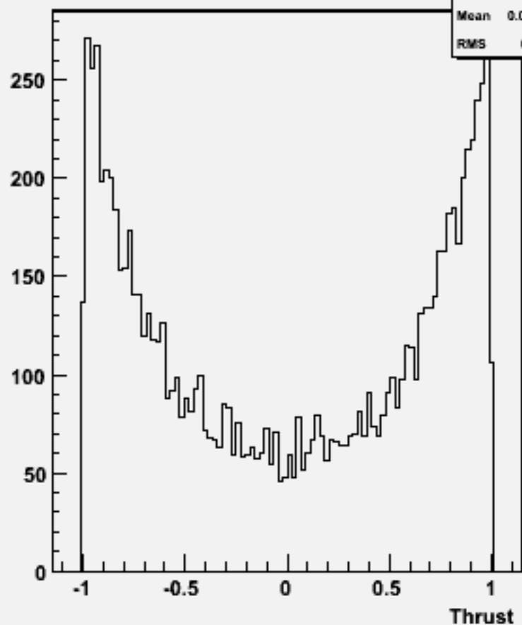
cos \Theta (thrust) w104370 e1e1h_o
