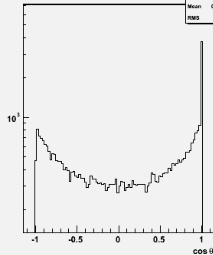
Jet cos \theta (All jets)w104370 e1e1h_o
