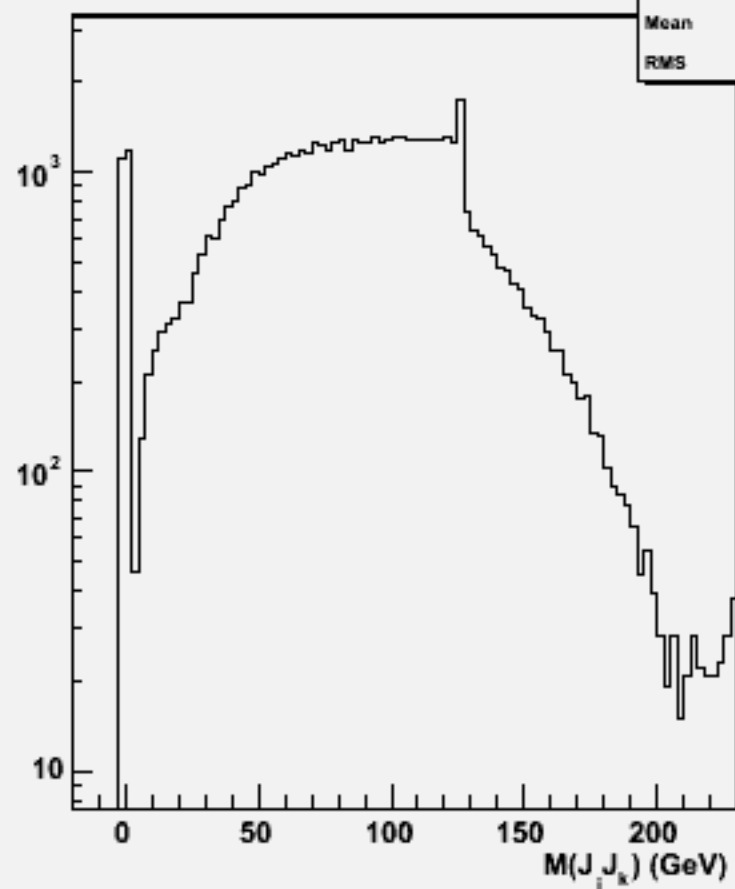
2jets mass(All comb)w104370 e1e1h_o
