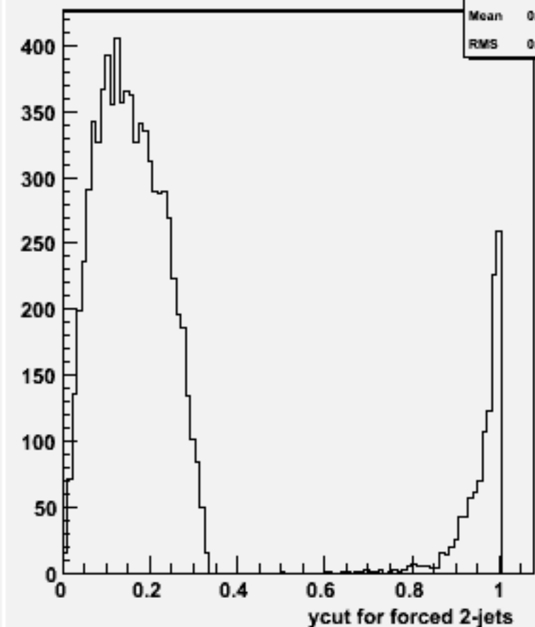
Ycut for 2-jets :w104370 e1e1h_o
