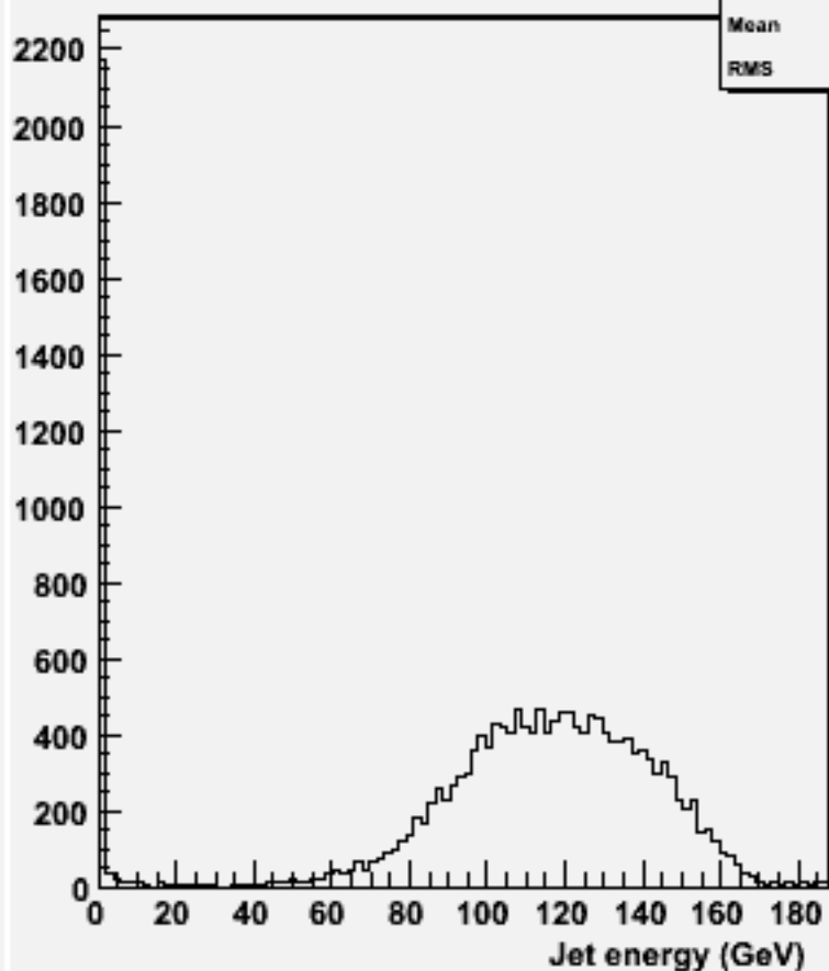
energy for 2-jets :w104370 e1e1h_o
