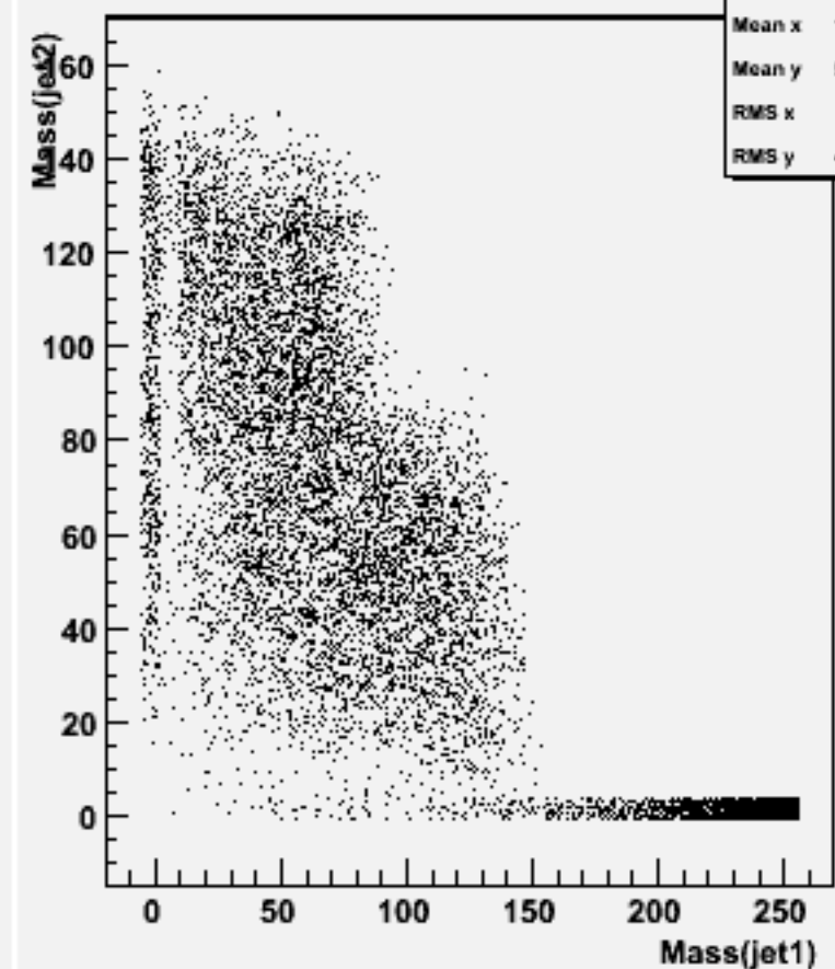
Jet mass for forced 2-jets : w104370 e1e1h_o
