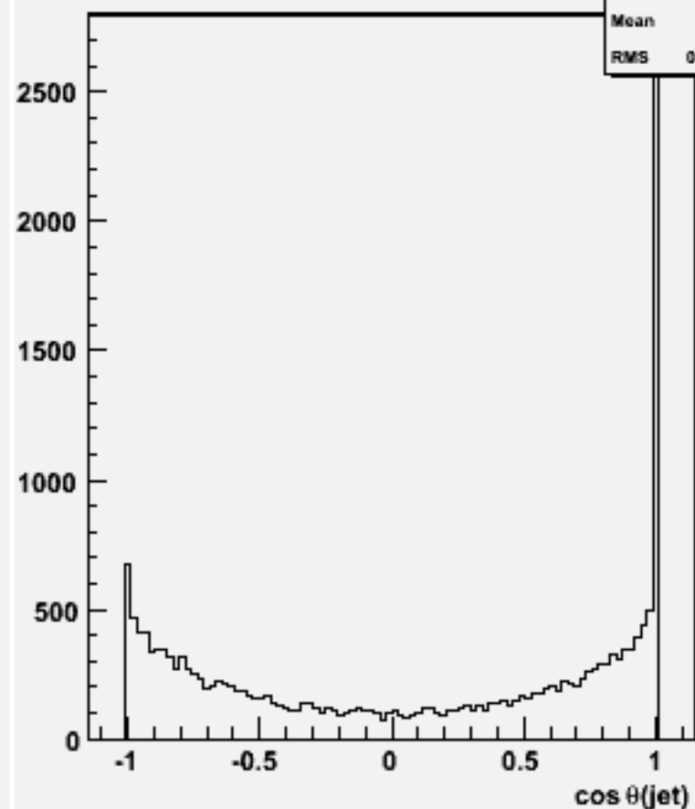
cos \theta for 2-jets :w104370 e1e1h_o
