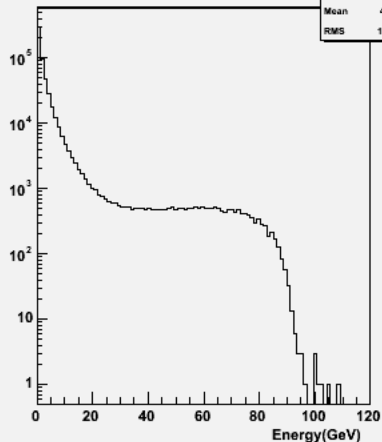
Particle Energy : w104370 e1e1h_o
