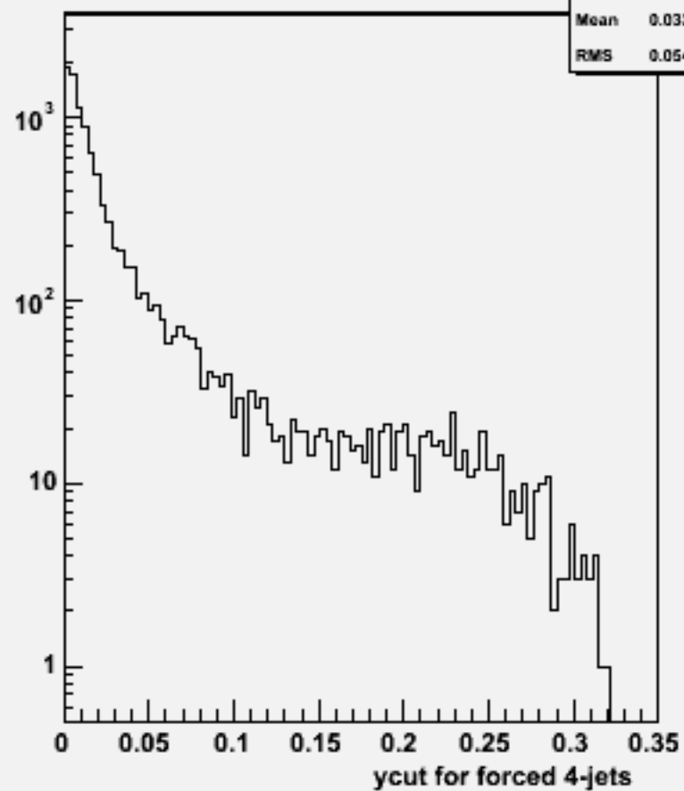
Ycut for 4-jets :w104370 e1e1h_o
