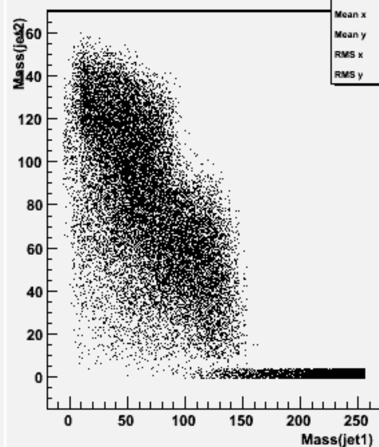
Jet mass for forced 2-jets : w104364 uuh_o
