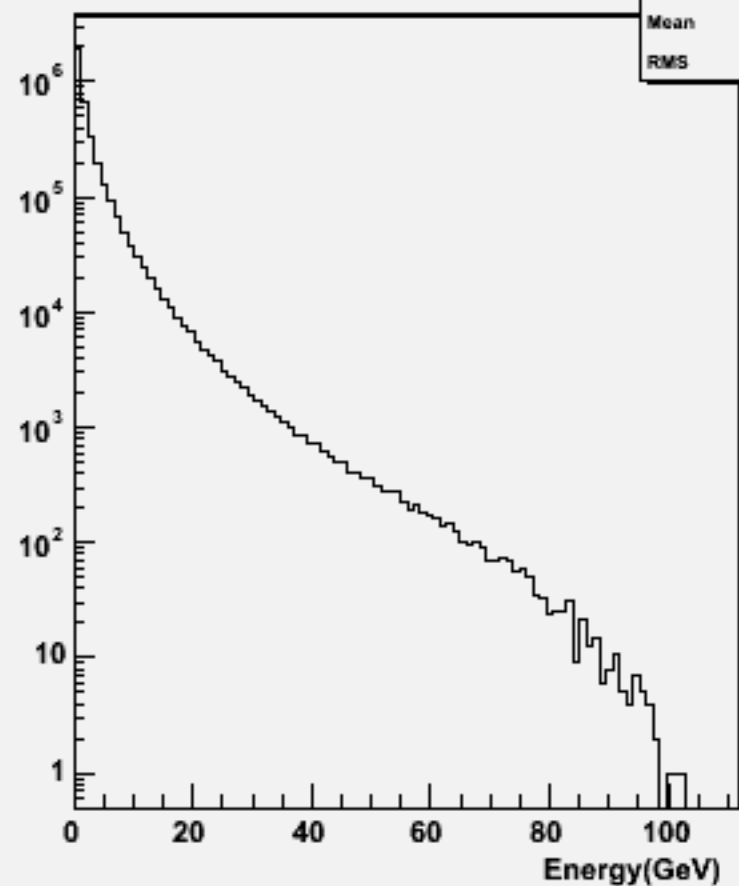
Particle Energy : w104364 uuh_o
