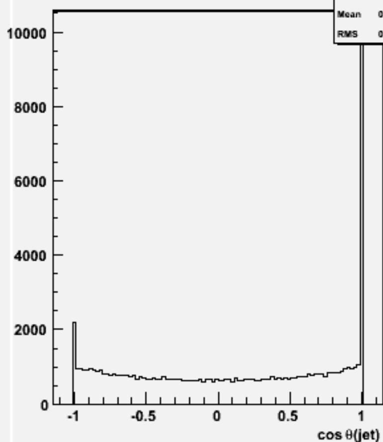
cos \theta for 2-jets :w104364 uuh_o
