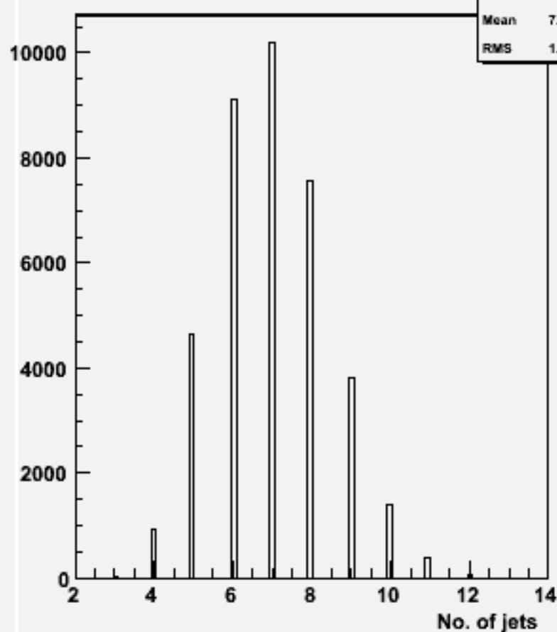
No. jets (ycut=0.001) : w104364 uuh_o
