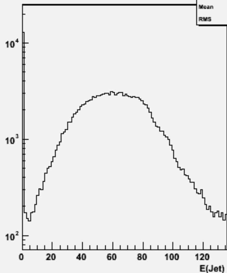
Jet energies(All jets)w104364 uuh_o
