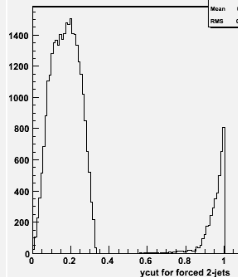
Ycut for 2-jets :w104364 uuh_o
