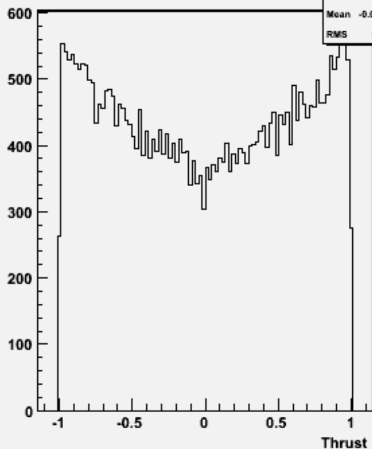
cos \Theta (thrust) w104364 uuh_o
