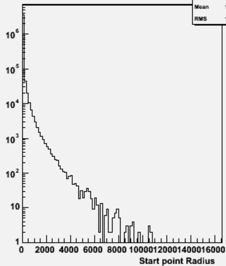
Start point R : w104364 uuh_o
