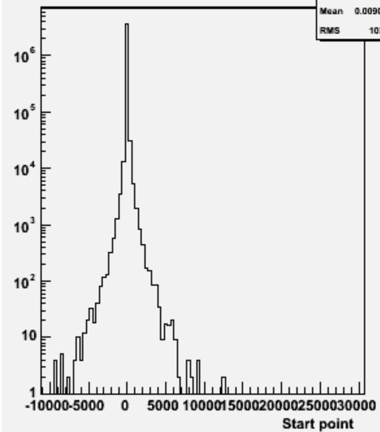
Start point Z : w104364 uuh_o
