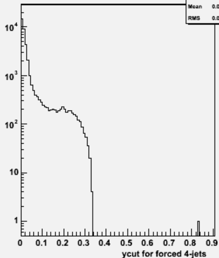
Ycut for 4-jets :w104364 uuh_o
