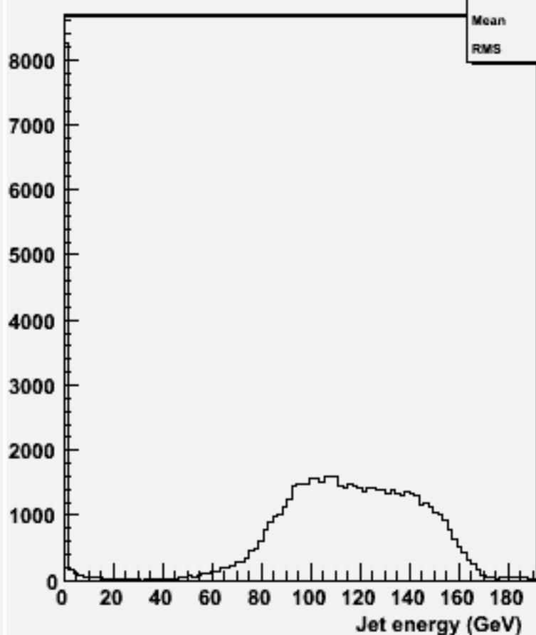
energy for 2-jets :w104364 uuh_o
