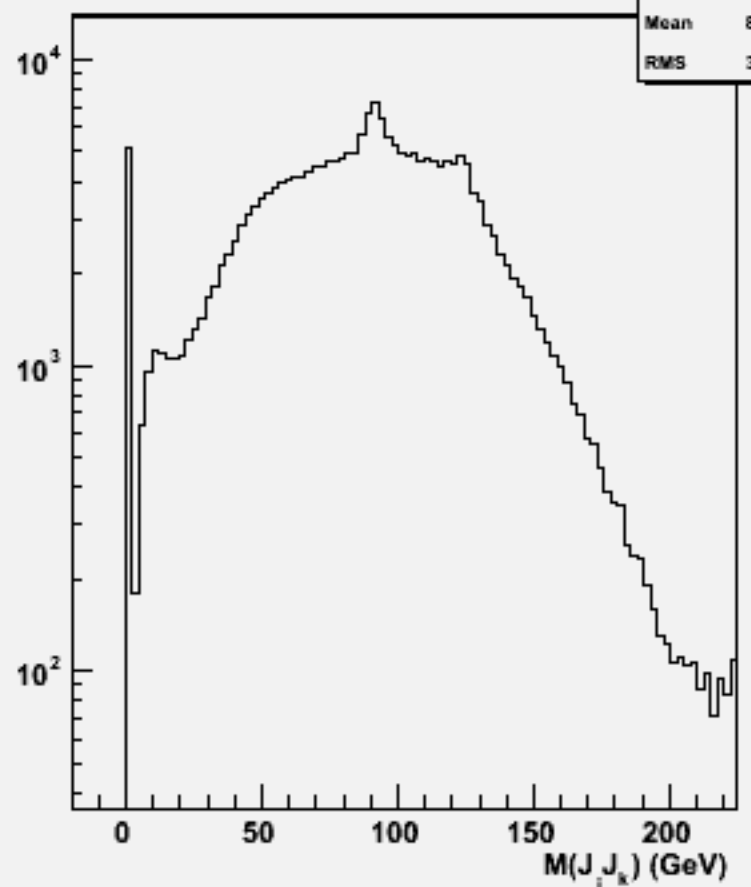
2jets mass(All comb)w104364 uuh_o
