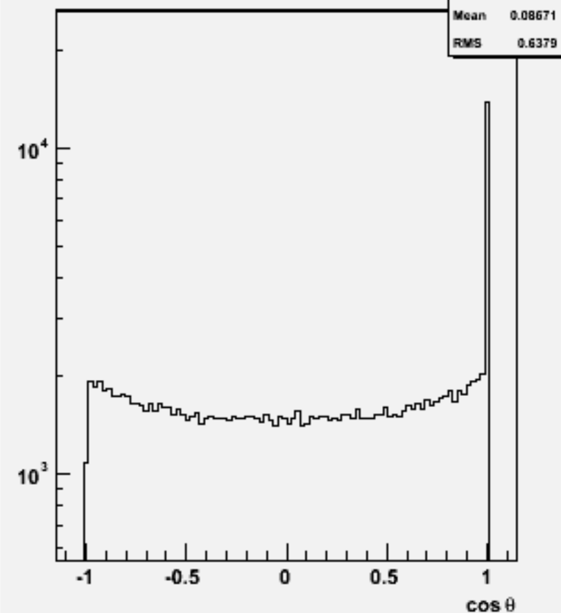
Jet cos \theta (All jets)w104364 uuh_o
