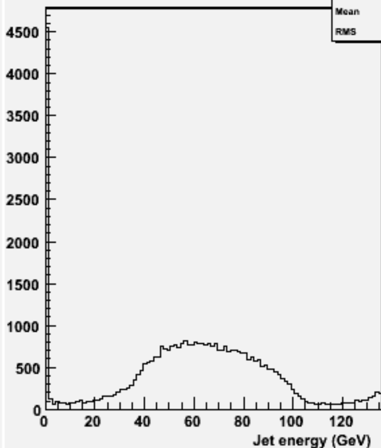
energy for 2-jets :w104360 n3n3h_o
