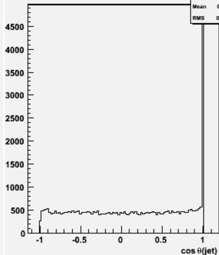
cos \theta for 2-jets :w104360 n3n3h_o
