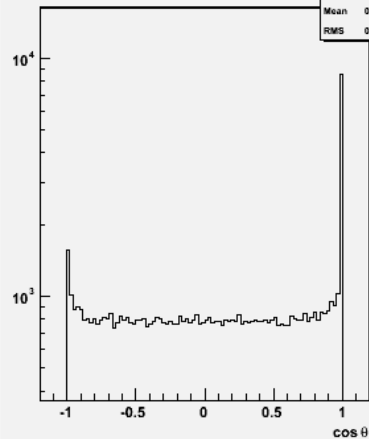
Jet cos \theta (All jets)w104360 n3n3h_o
