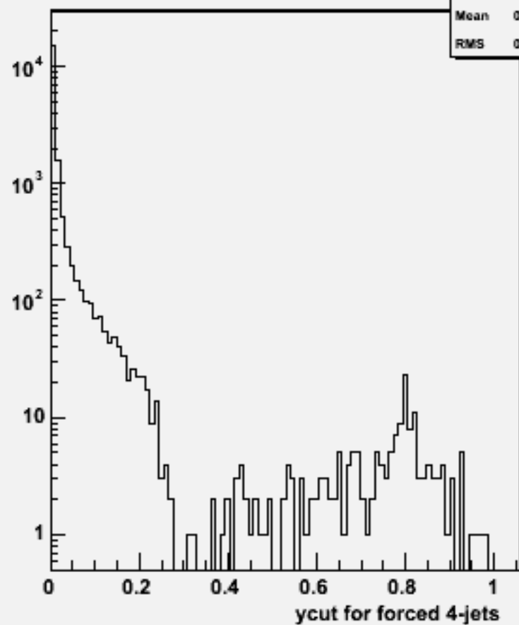
Ycut for 4-jets :w104360 n3n3h_o
