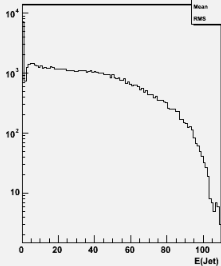
Jet energies(All jets)w104360 n3n3h_o
