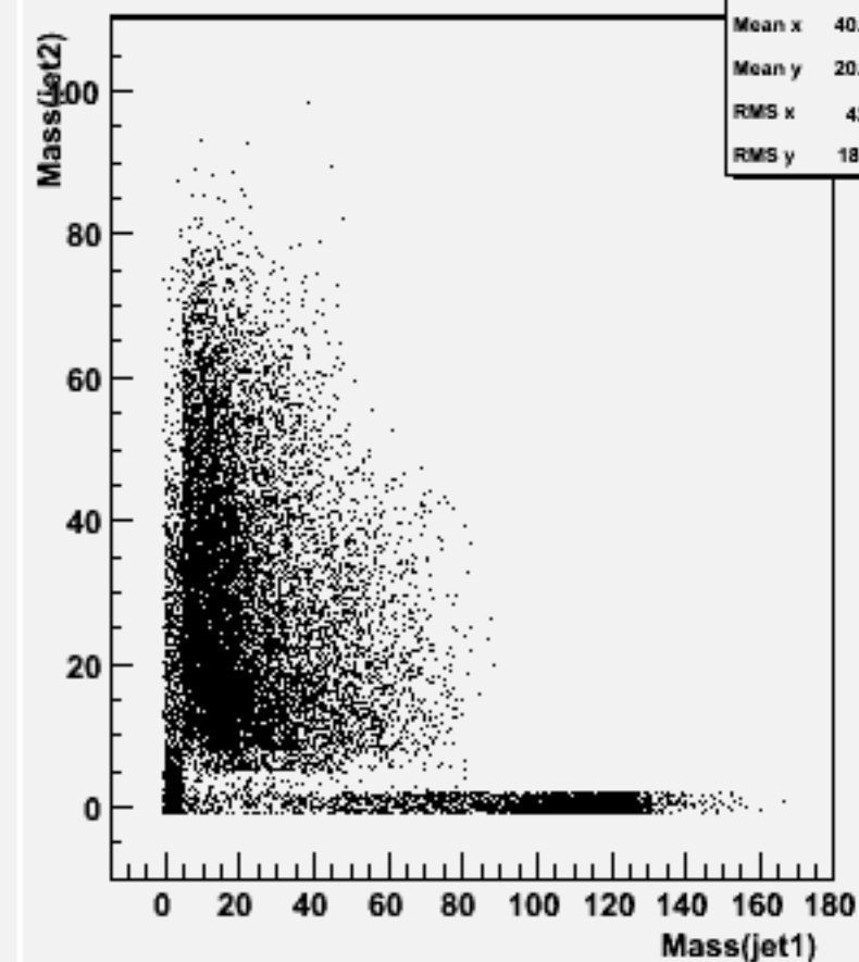
Jet mass for forced 2-jets : w104360 n3n3h_o
