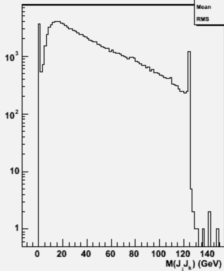
2jets mass(All comb)w104360 n3n3h_o
