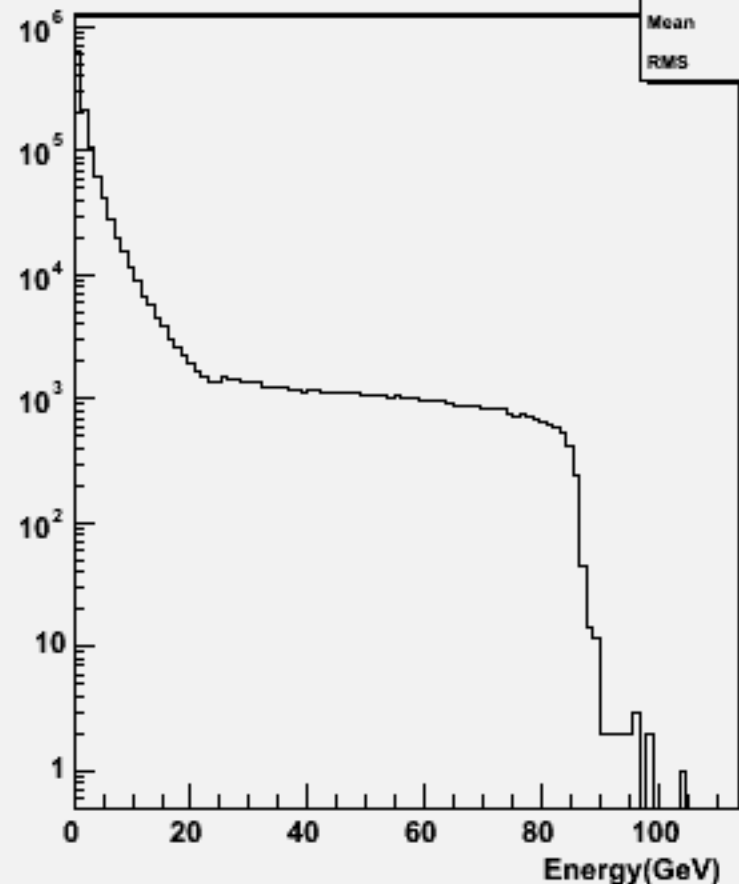
Particle Energy : w104360 n3n3h_o
