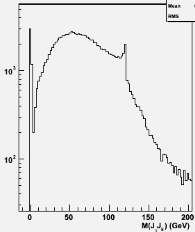
2jets mass(All comb)w104329 e3e3h_o
