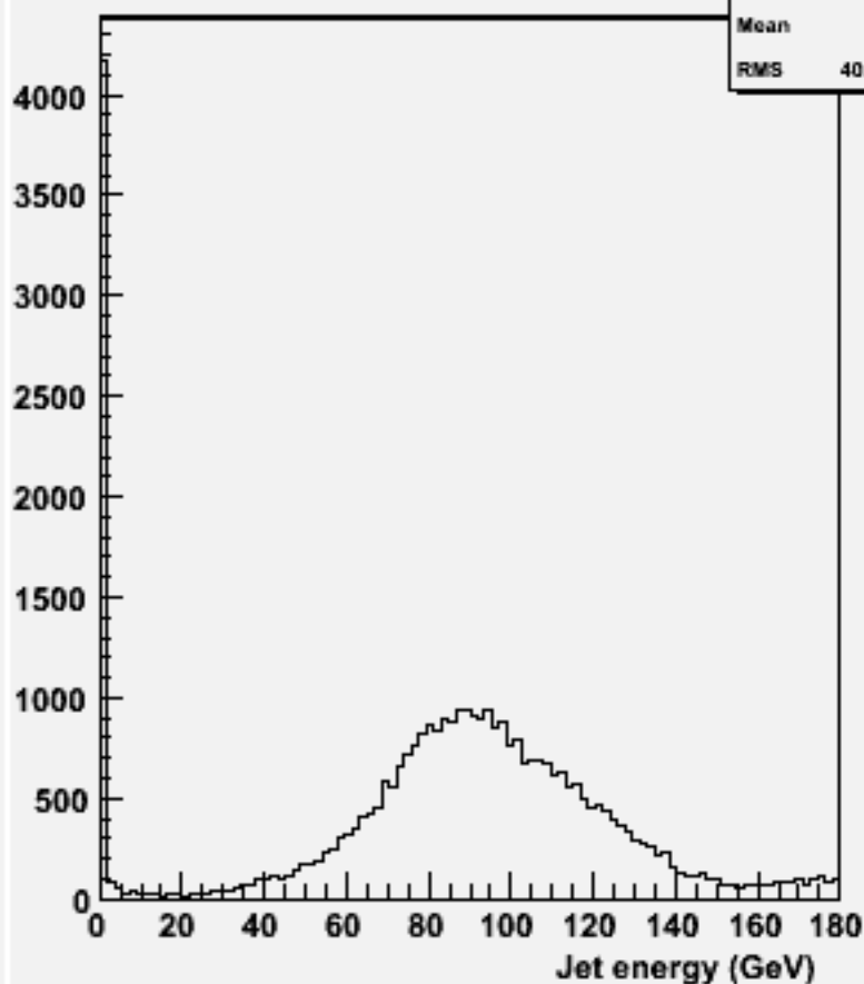
energy for 2-jets :w104329 e3e3h_o
