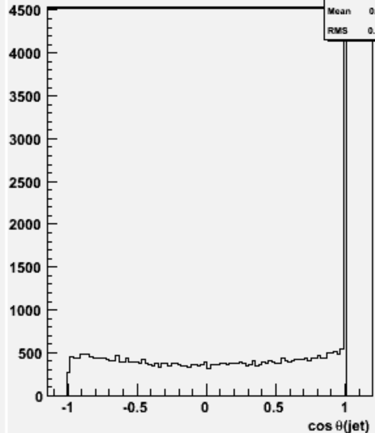
cos \theta for 2-jets :w104329 e3e3h_o
