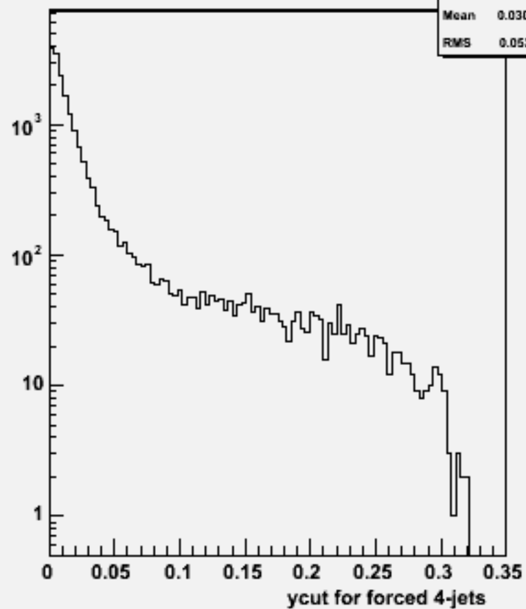
Ycut for 4-jets :w104329 e3e3h_o
