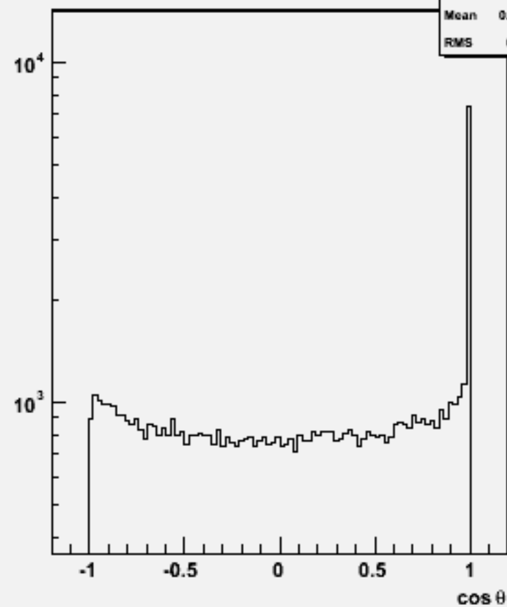
Jet cosθ (All jets)w104329 e3e3h_o
