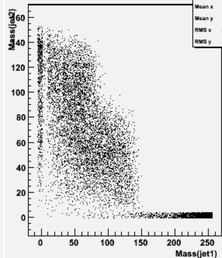
Jet mass for forced 2-jets : w104323 e1e1h_o
