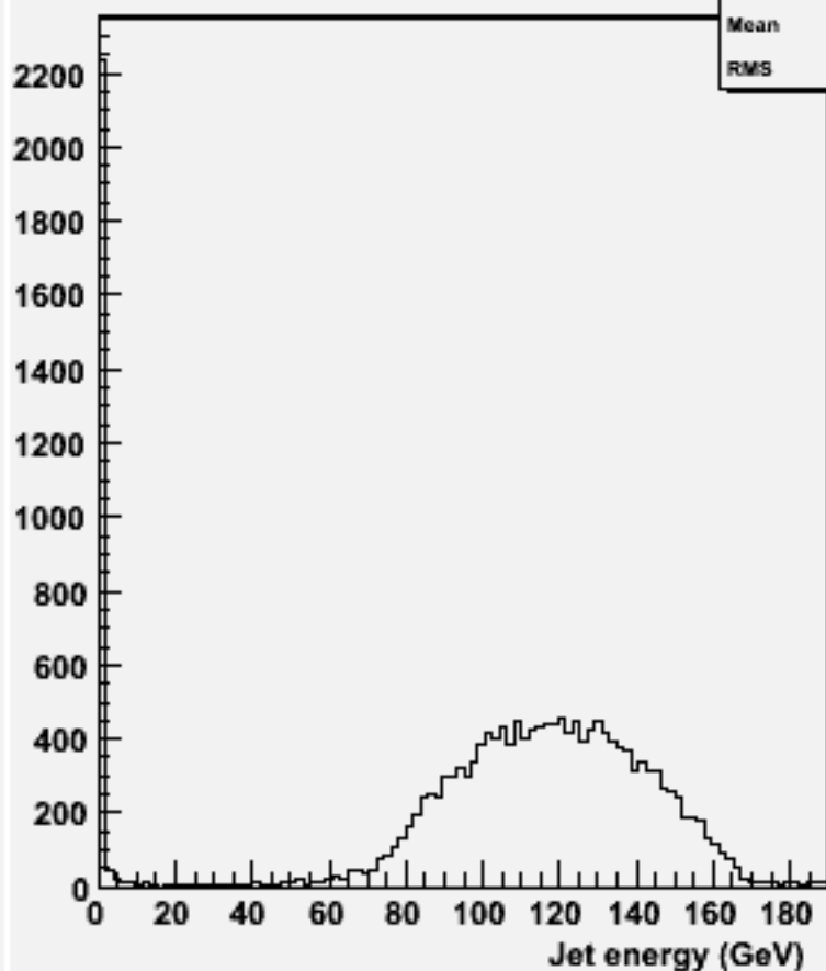
energy for 2-jets :w104323 e1e1h_o
