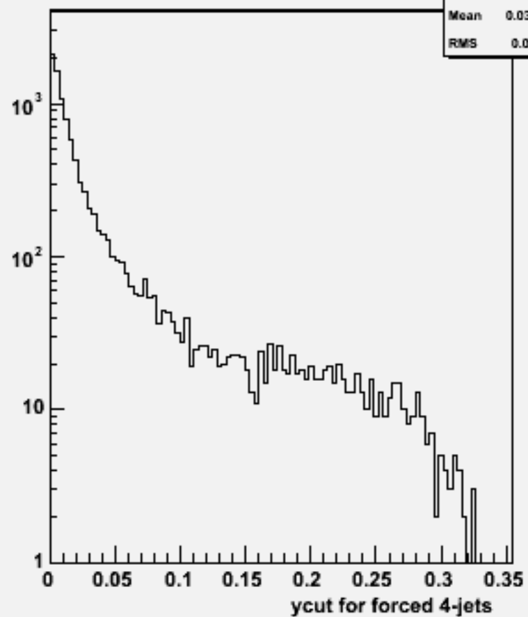
Ycut for 4-jets :w104323 e1e1h_o
