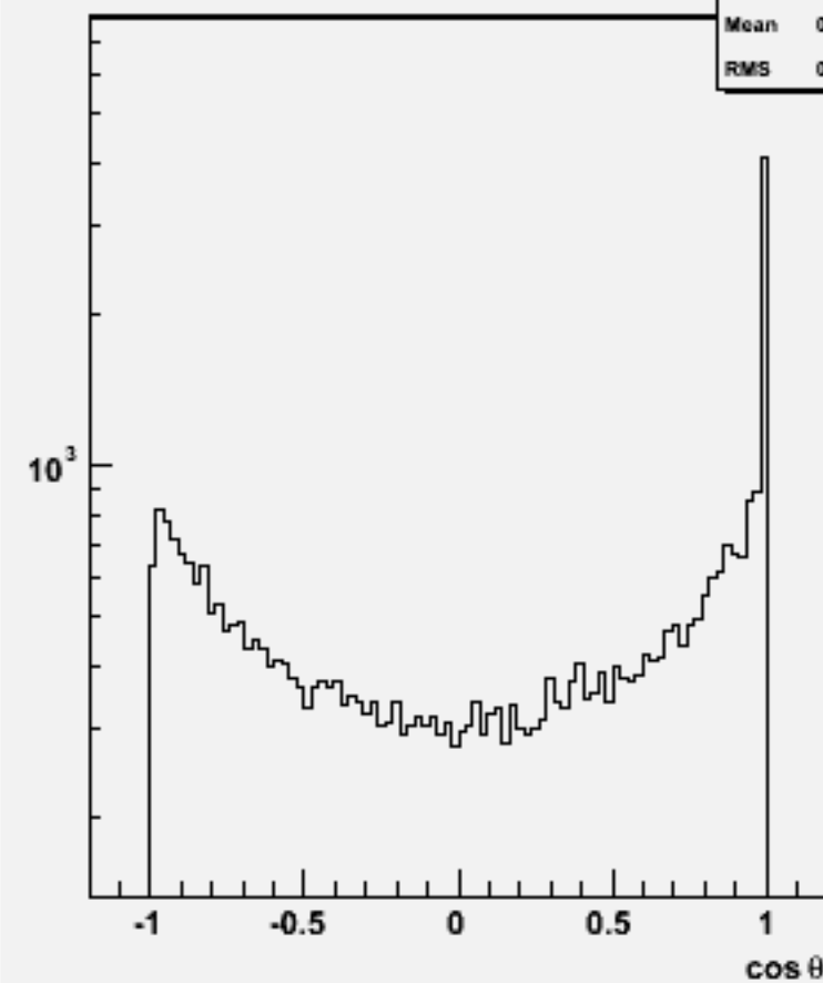
Jet cos \theta (All jets)w104323 e1e1h_o
