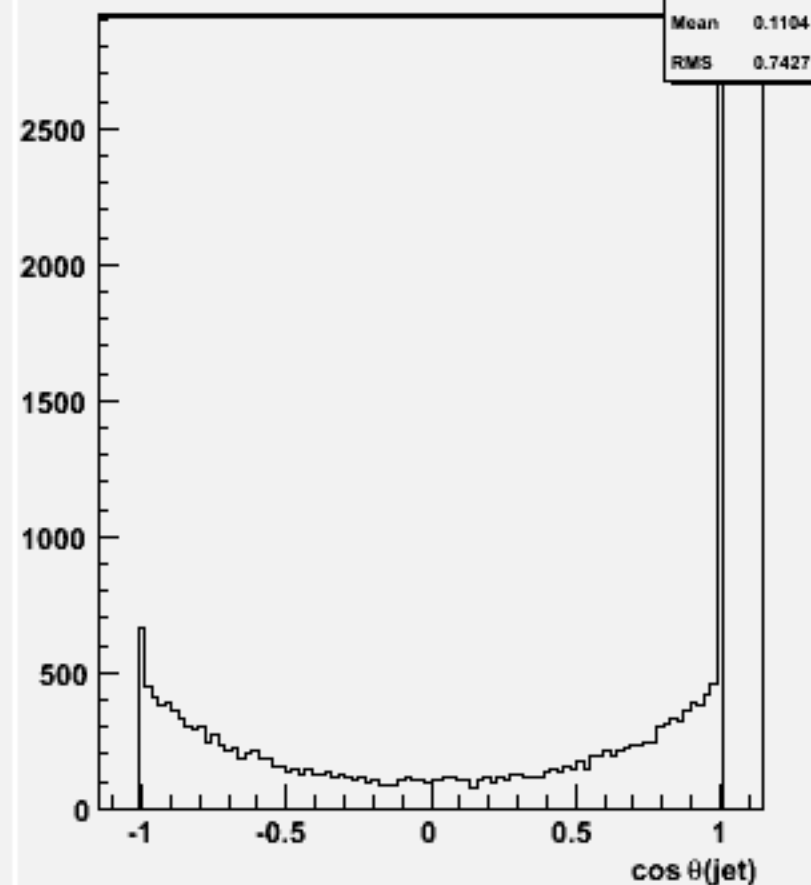
cos \theta for 2-jets :w104323 e1e1h_o
