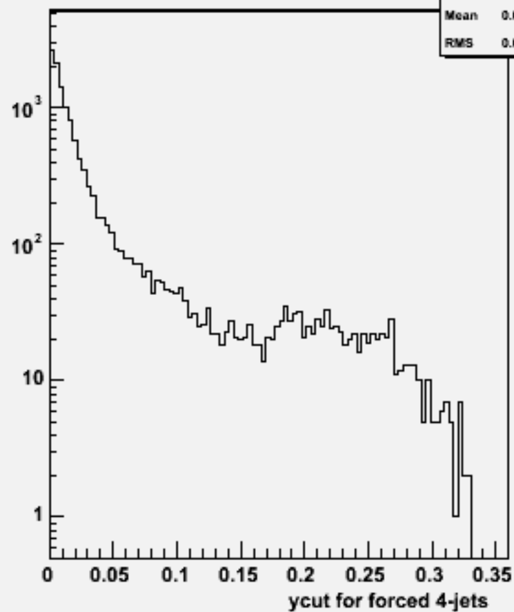
Ycut for 4-jets :w104322 e1e1h_o
