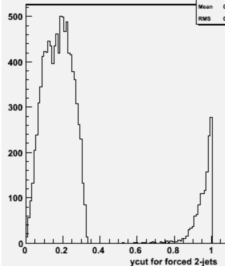
Ycut for 2-jets :w104322 e1e1h_o
