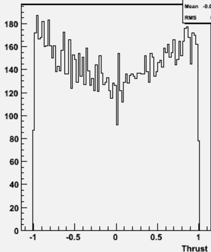
cos \Theta (thrust) w104322 e1e1h_o
