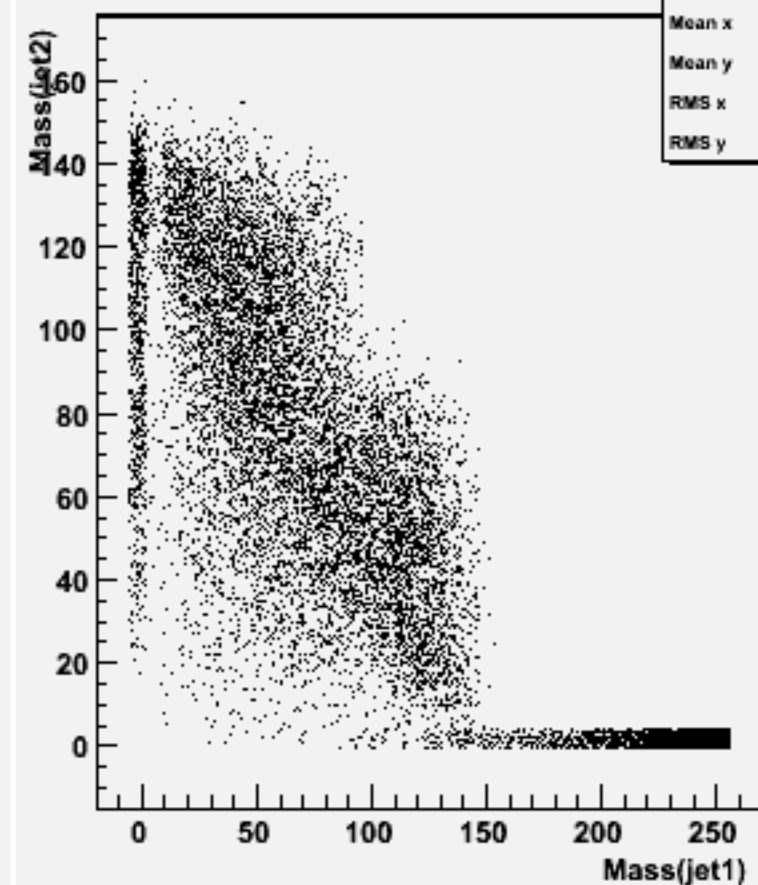
Jet mass for forced 2-jets : w104322 e1e1h_o
