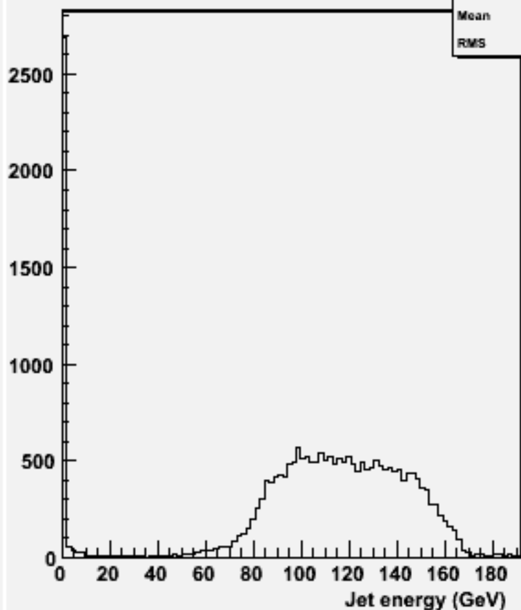
energy for 2-jets :w104322 e1e1h_o
