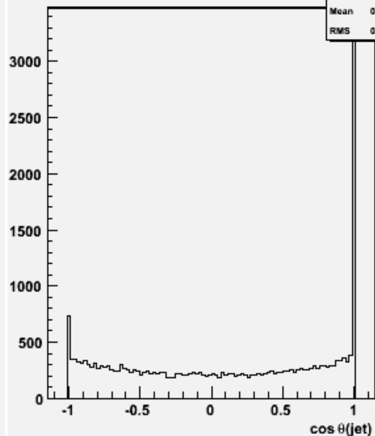
cos \theta for 2-jets :w104322 e1e1h_o
