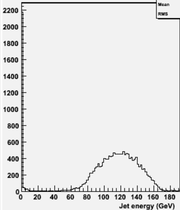
energy for 2-jets :w104320 e1e1h_o
