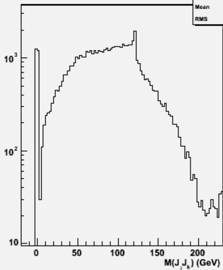
2jets mass(All comb)w104320 e1e1h_o
