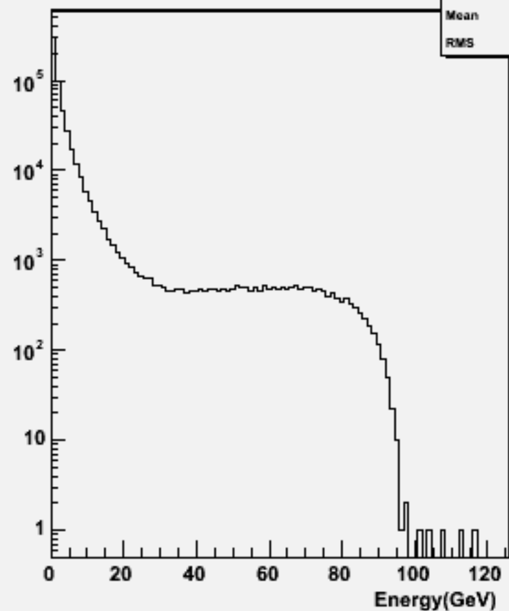
Particle Energy : w104320 e1e1h_o
