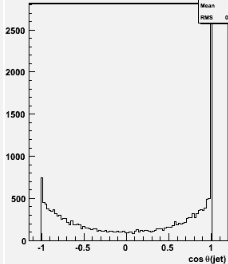
cos \theta for 2-jets :w104320 e1e1h_o
