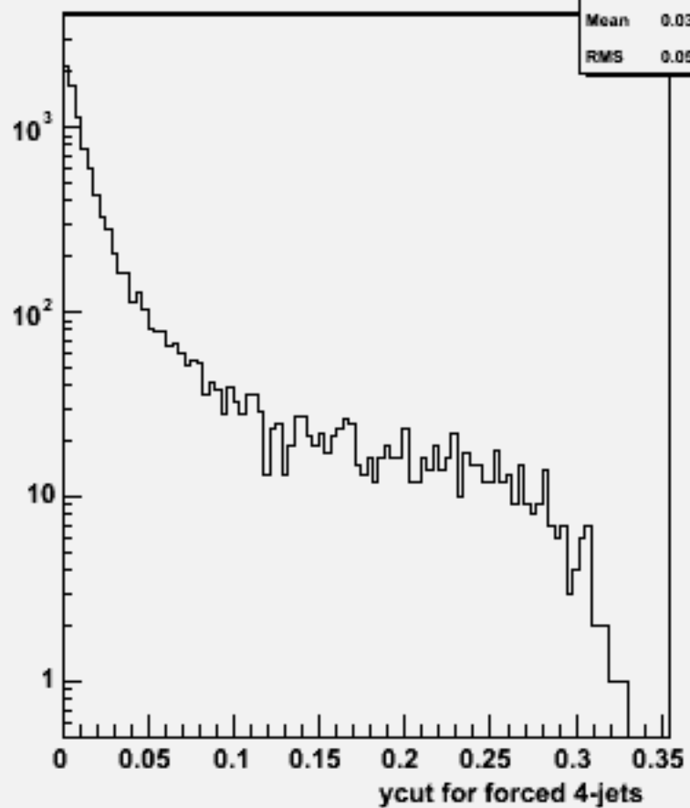
Ycut for 4-jets :w104320 e1e1h_o
