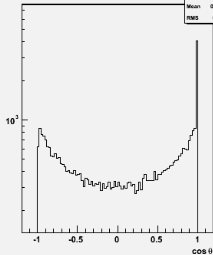
Jet cos \theta (All jets)w104320 e1e1h_o
