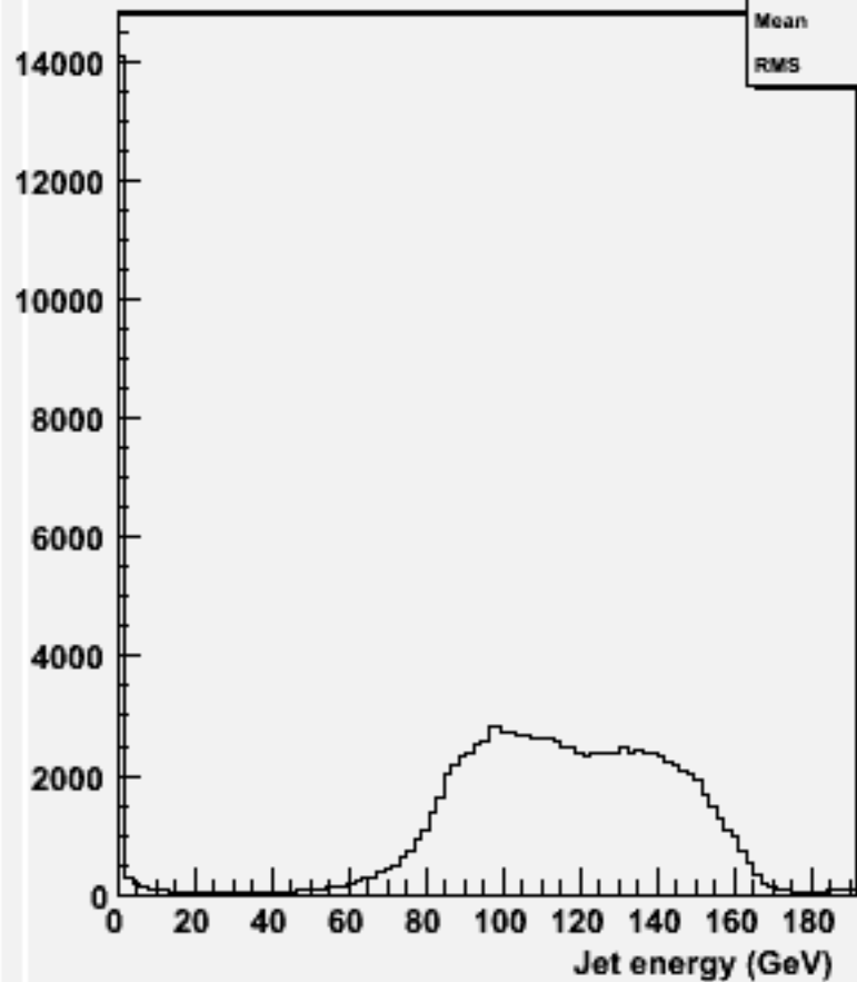
energy for 2-jets :w104317 cch_o
