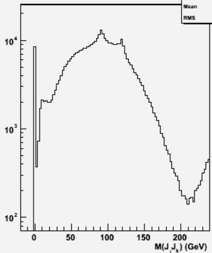
2jets mass(All comb)w104317 cch_o
