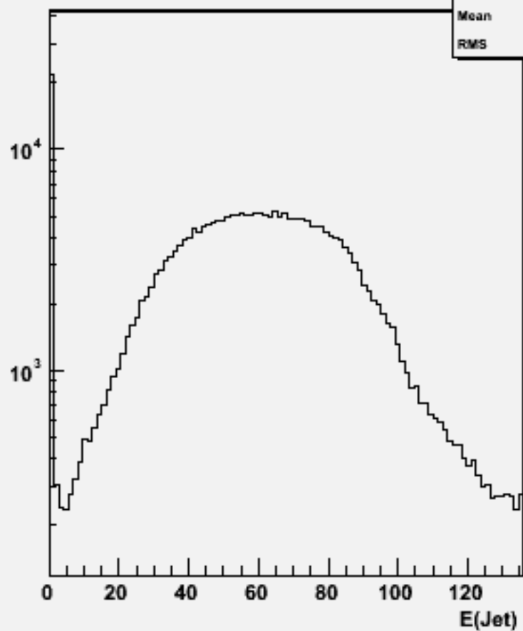
Jet energies(All jets)w104317 cch_o
