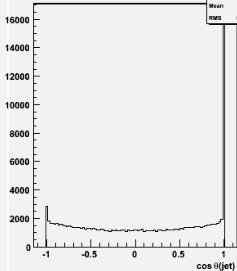
cos \Theta for 2-jets :w104317 cch_o
