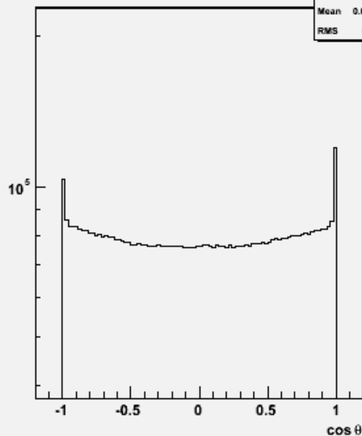
Particle \cos\theta : w104317 cch_o
