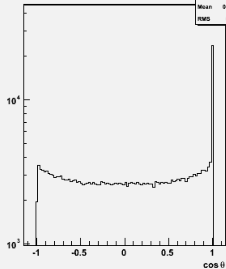
Jet cosθ (All jets)w104317 cch_o
