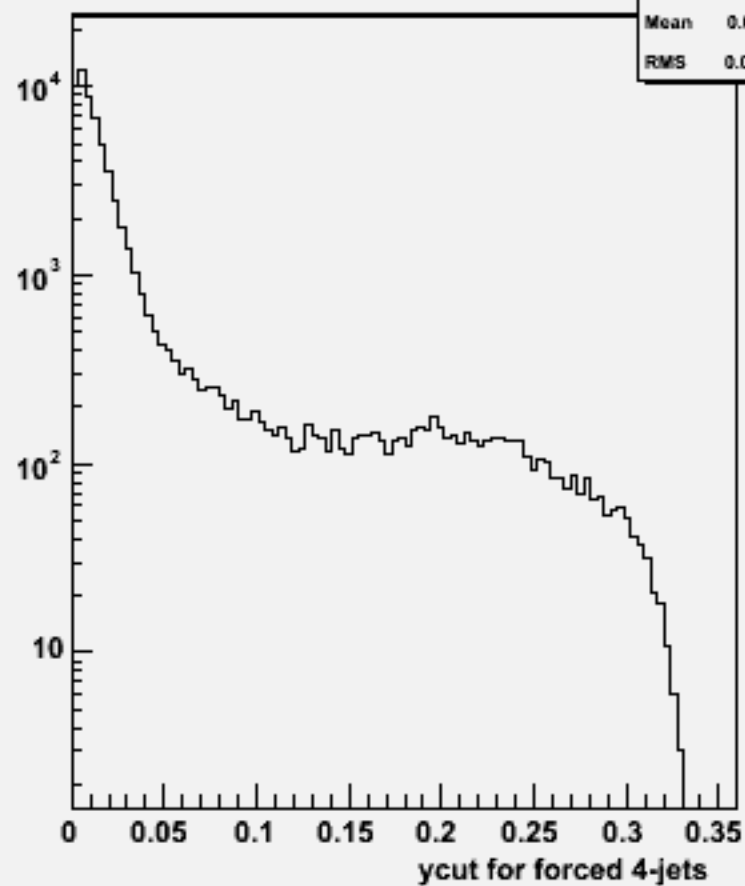
Ycut for 4-jets :w104317 cch_o
