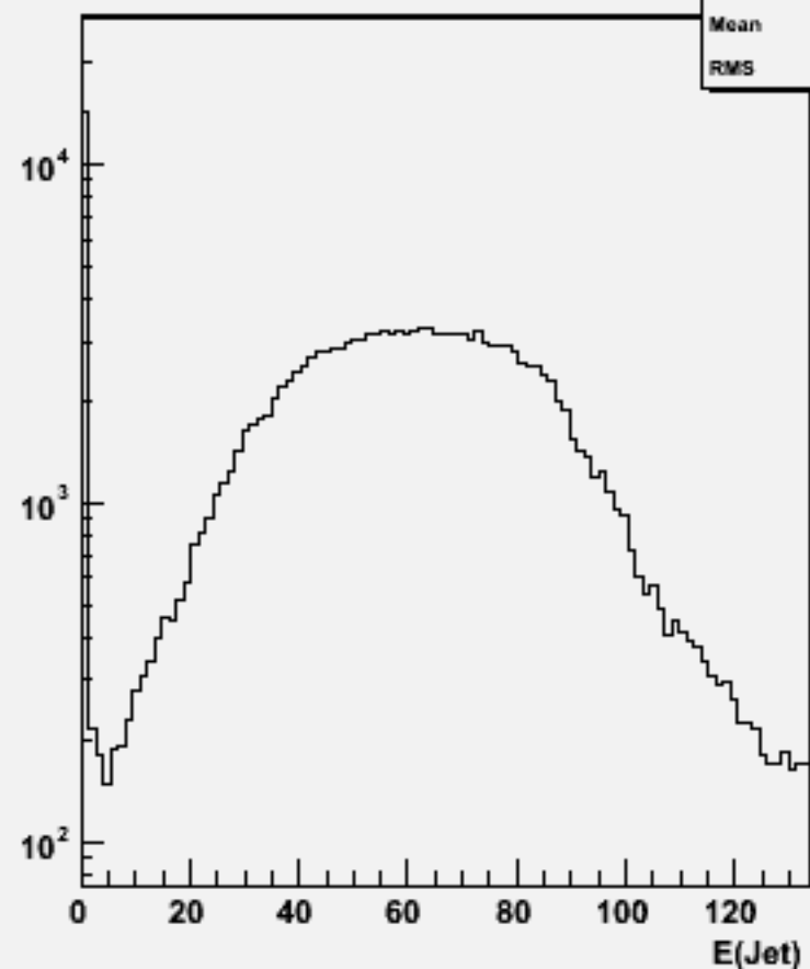
Jet energies(All jets)w104314 uuh_o
