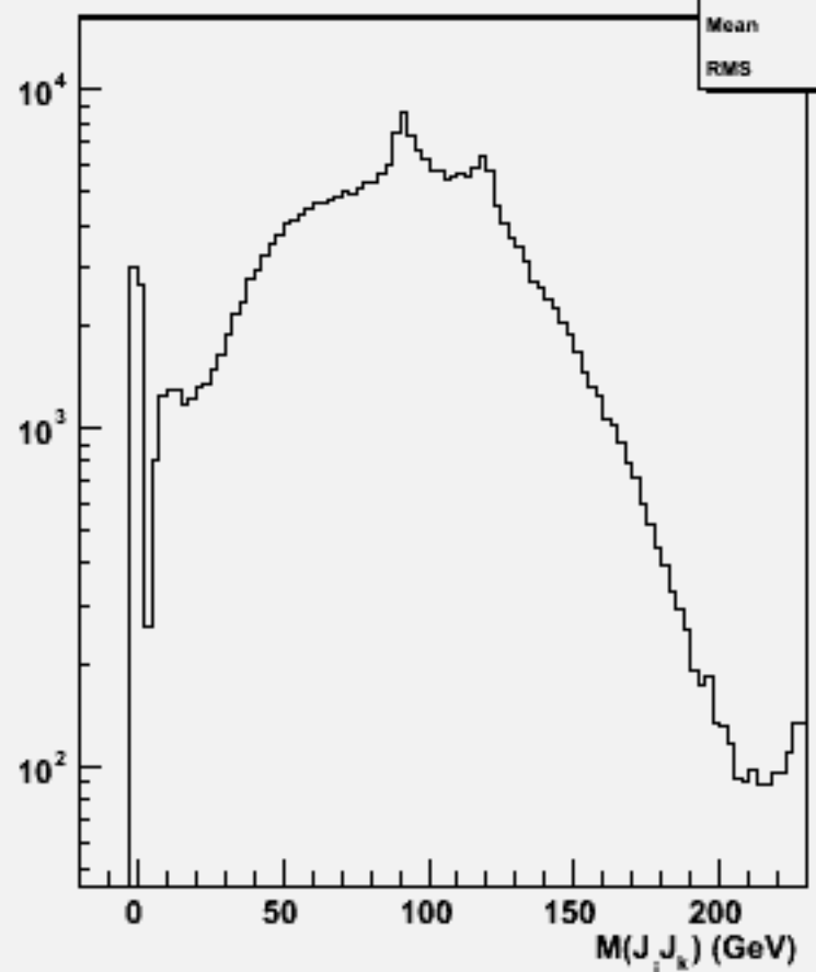
2jets mass(All comb)w104314 uuh_o
