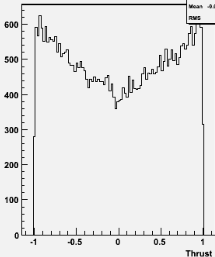
cos \Theta (thrust) w104314 uuh_o
