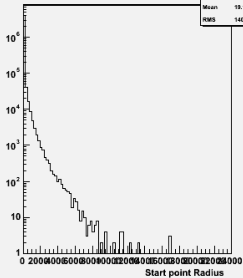
Start point R : w104314 uuh_o
