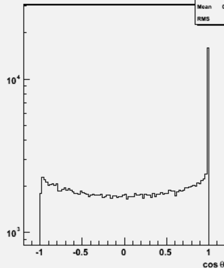
Jet cosθ (All jets)w104314 uuh_o
