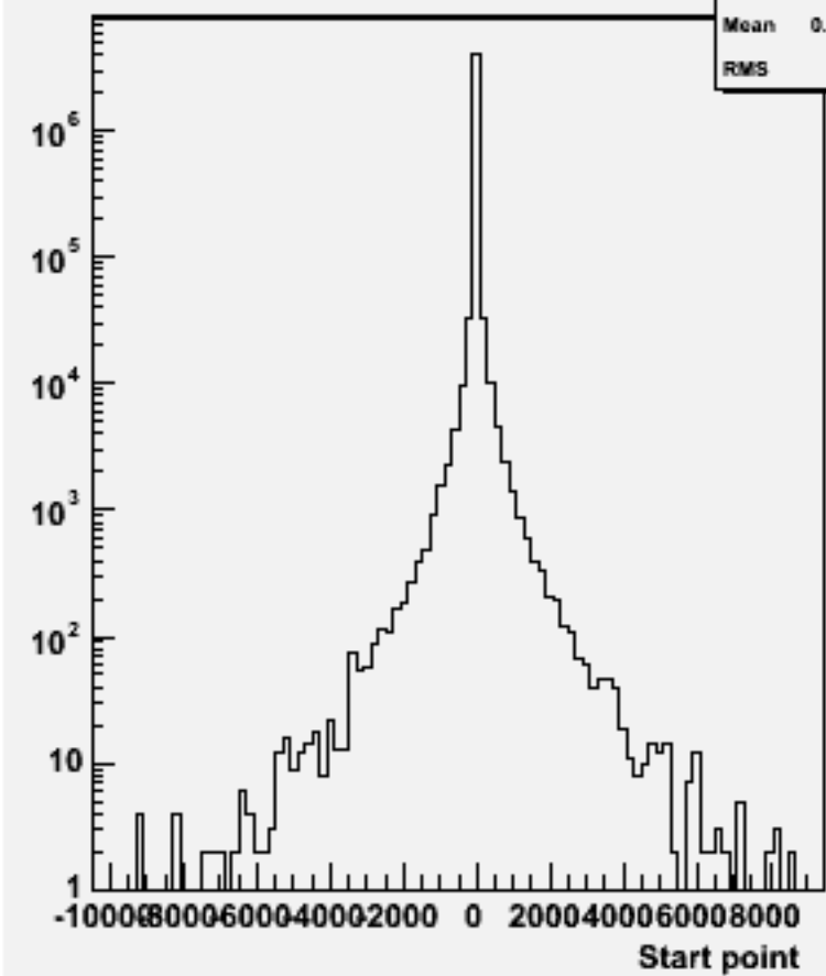
Start point Z : w104314 uuh_o
