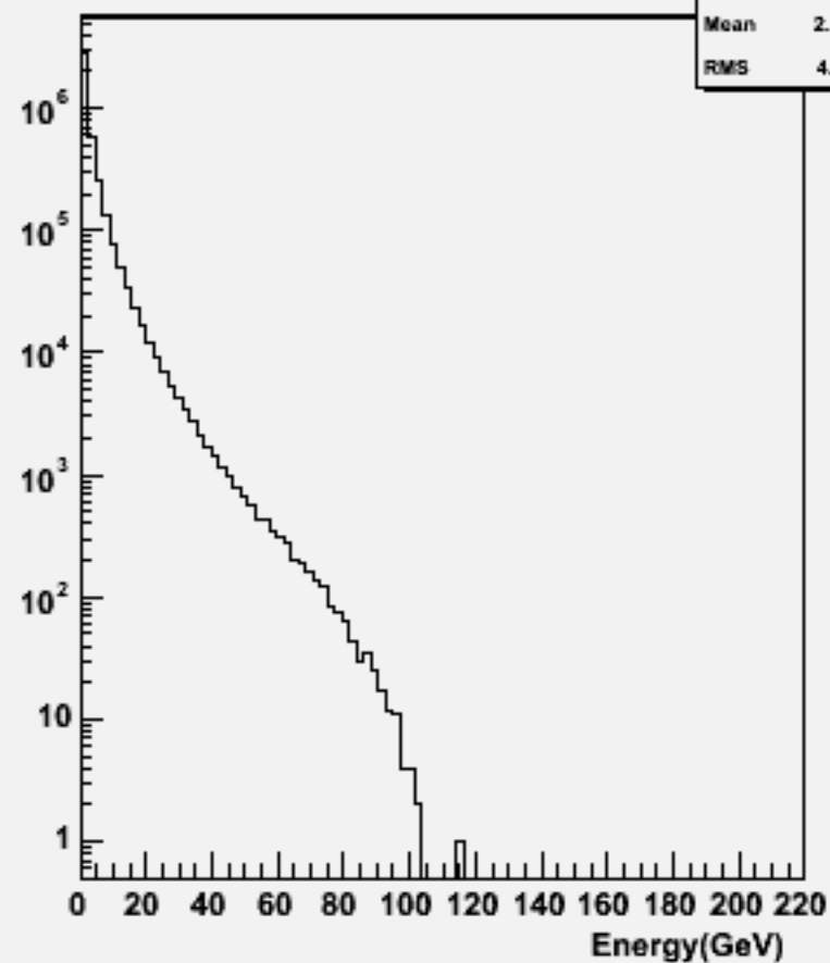
Particle Energy : w104314 uuh_o
