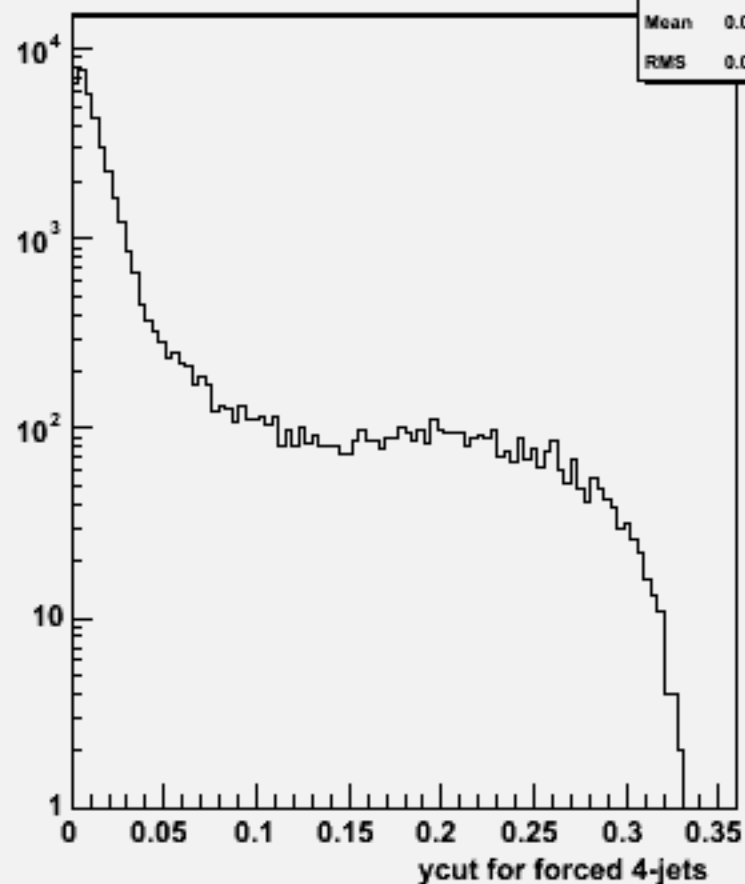
Ycut for 4-jets :w104314 uuh_o
