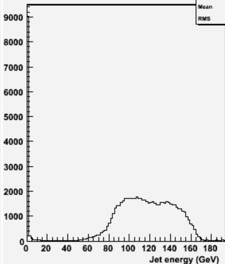
energy for 2-jets :w104314 uuh_o
