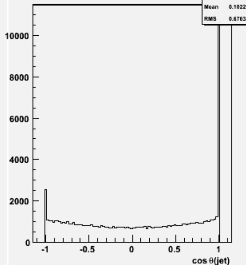
cos \theta for 2-jets :w104314 uuh_o
