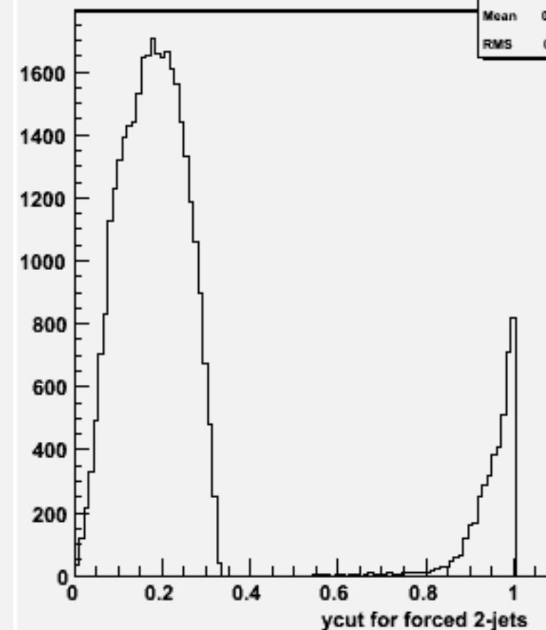
Ycut for 2-jets :w104314 uuh_o
