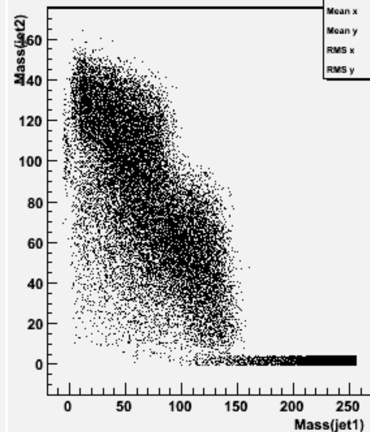
Jet mass for forced 2-jets : w104314 uuh_o
