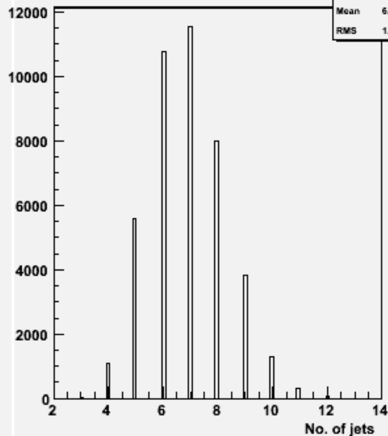
No. jets (ycut=0.001) : w104314 uuh_o
