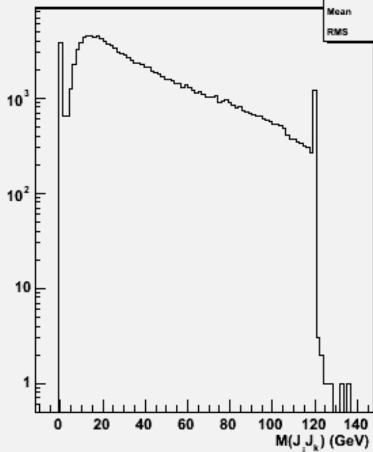
2jets mass(All comb)w104310 n3n3h_o
