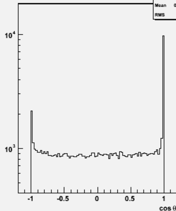
Jet cosθ (All jets)w104310 n3n3h_o
