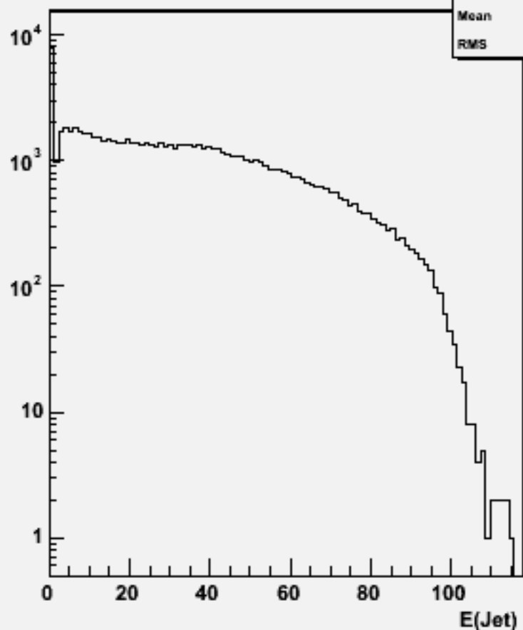
Jet energies(All jets)w104310 n3n3h_o
