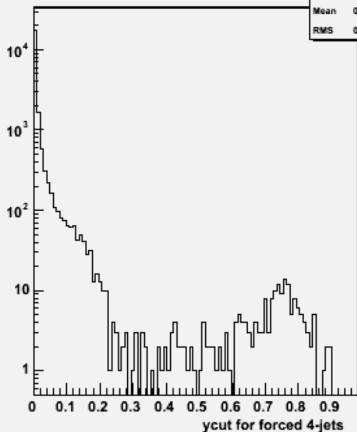
Ycut for 4-jets :w104310 n3n3h_o
