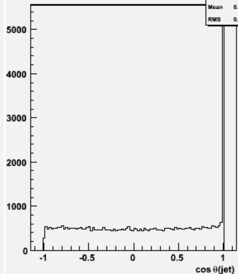
cos \theta for 2-jets :w104310 n3n3h_o
