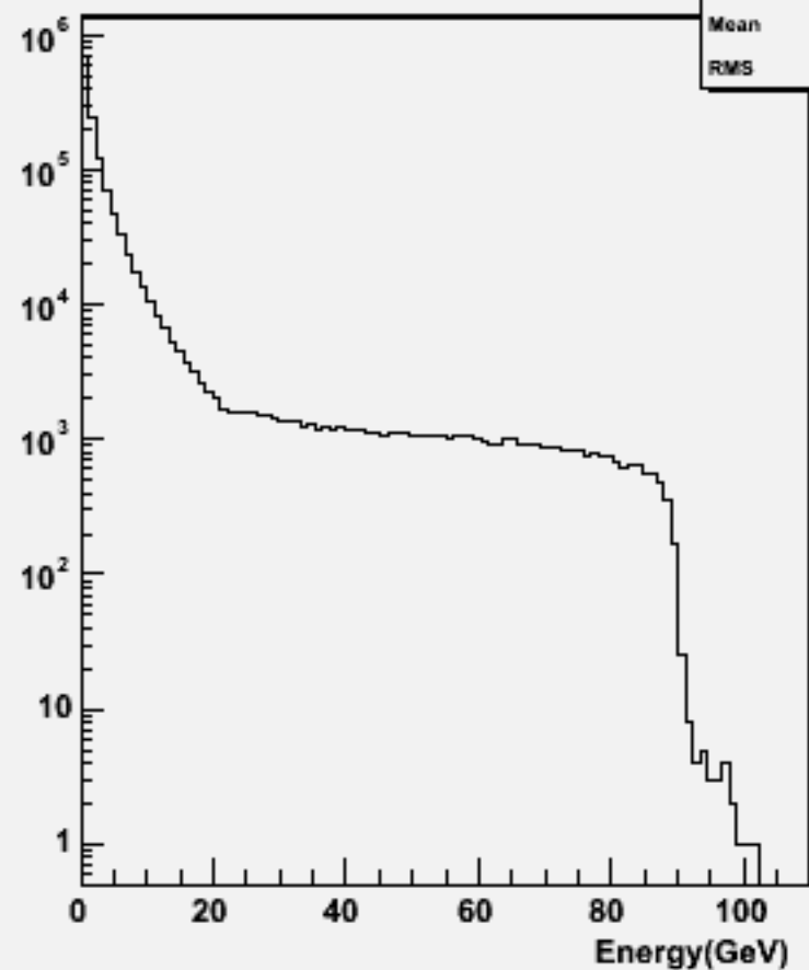
Particle Energy : w104310 n3n3h_o
