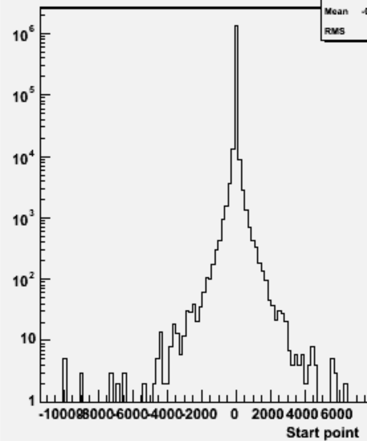
Start point Z : w104310 n3n3h_o
