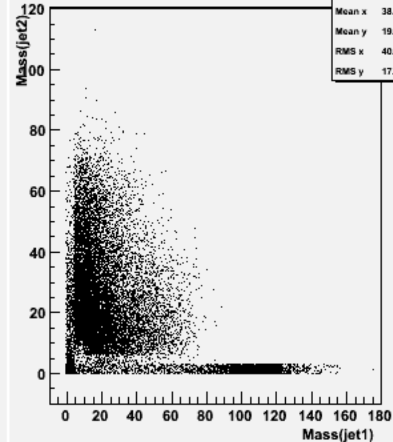
Jet mass for forced 2-jets : w104310 n3n3h_o
