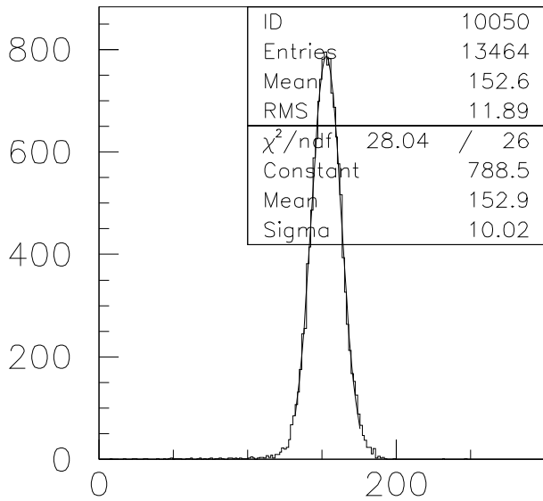
hcal-pi50GeV
