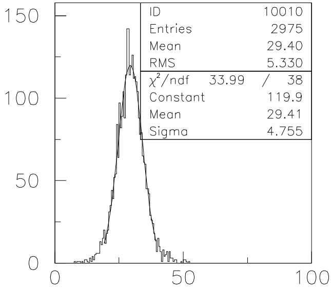
hcal-pi10GeV
