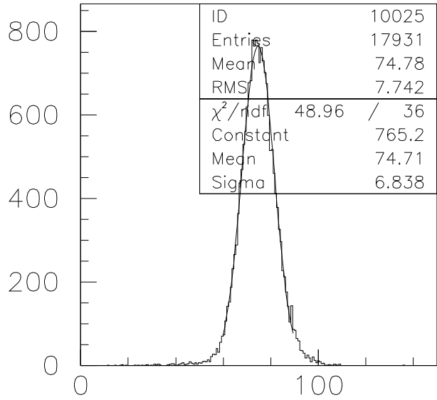
hcal-pi25GeV
