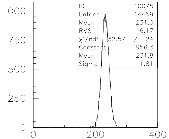
hcal-pi75GeV
