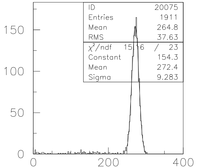
hcal-e75GeV
