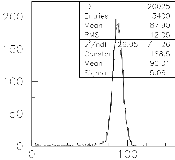
hcal-e25GeV
