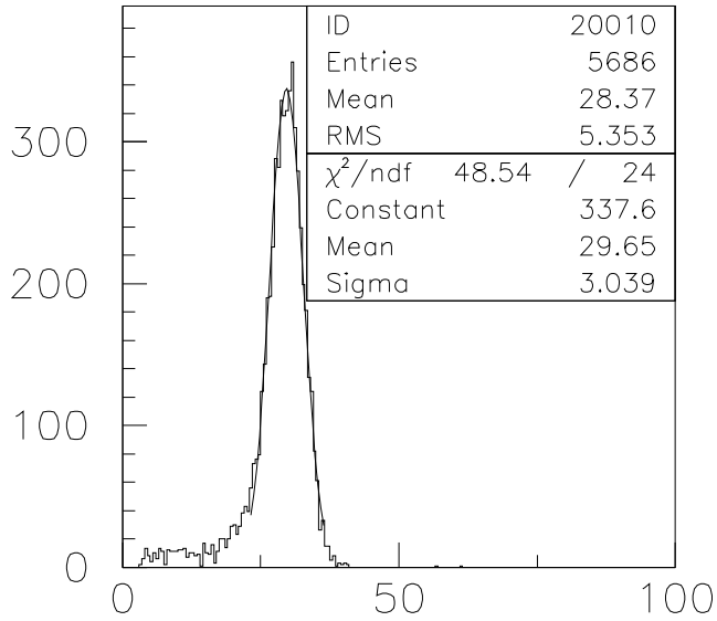
hcal-e10GeV
