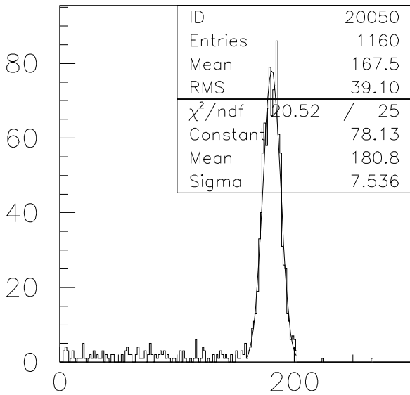
hcal-e50GeV
