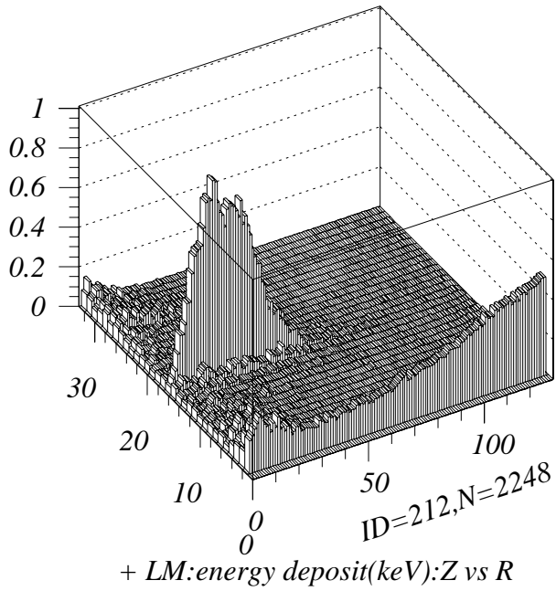
a 50 GeV electron with 100 bunch crossings: Luminosity monitor
