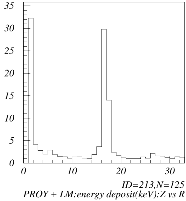
a 50 GeV electron with 100 bunch crossings: Luminosity monitor
