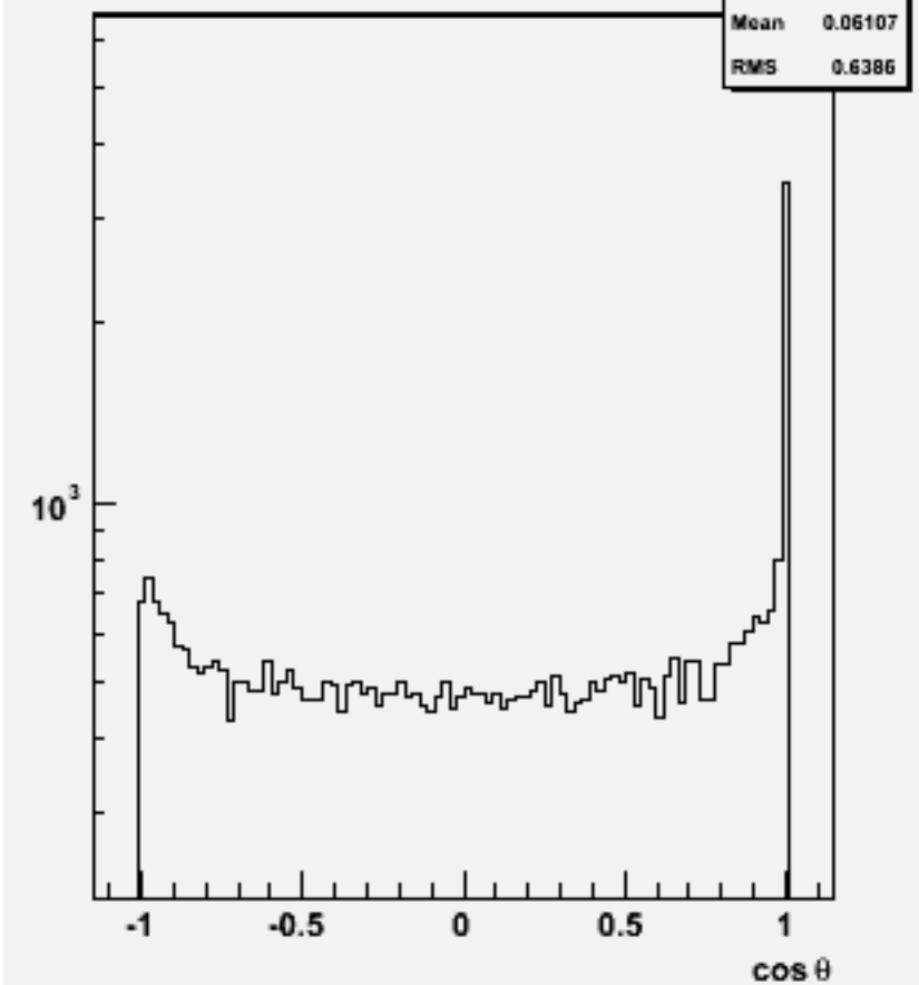
Jet cos \theta (All jets)106412 physsim-tth-ln4q-hnonbb
