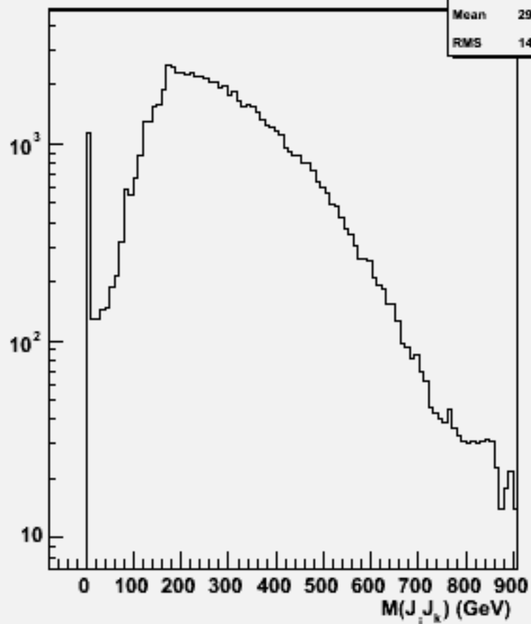
Zjets mass(All comb)106412 physsim-tth-ln4q-hnonbb
