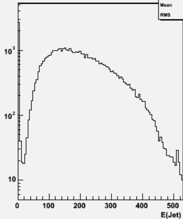
Jet energies(All jets)106412 physsim-tth-ln4q-hnonbb
