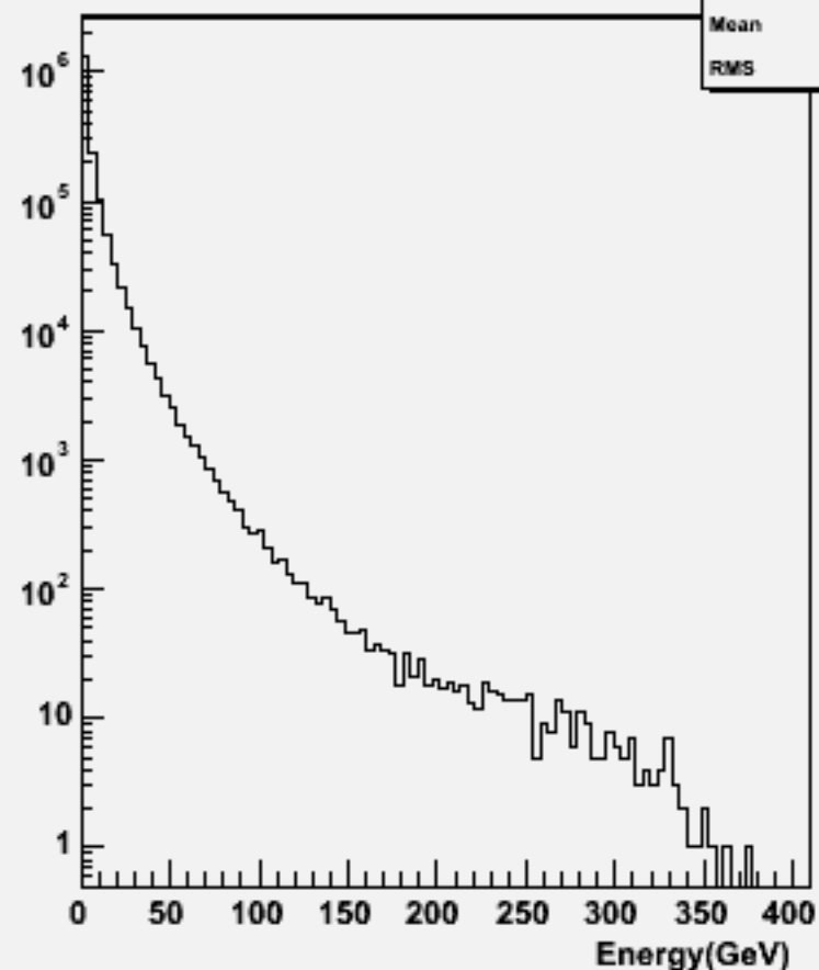
Particle Energy : 106451 physsim-tth-6q-hbb
