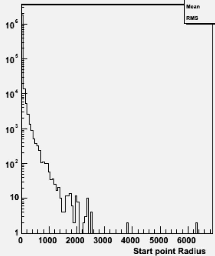
Start point R : 106451 physsim-tth-6q-hbb
