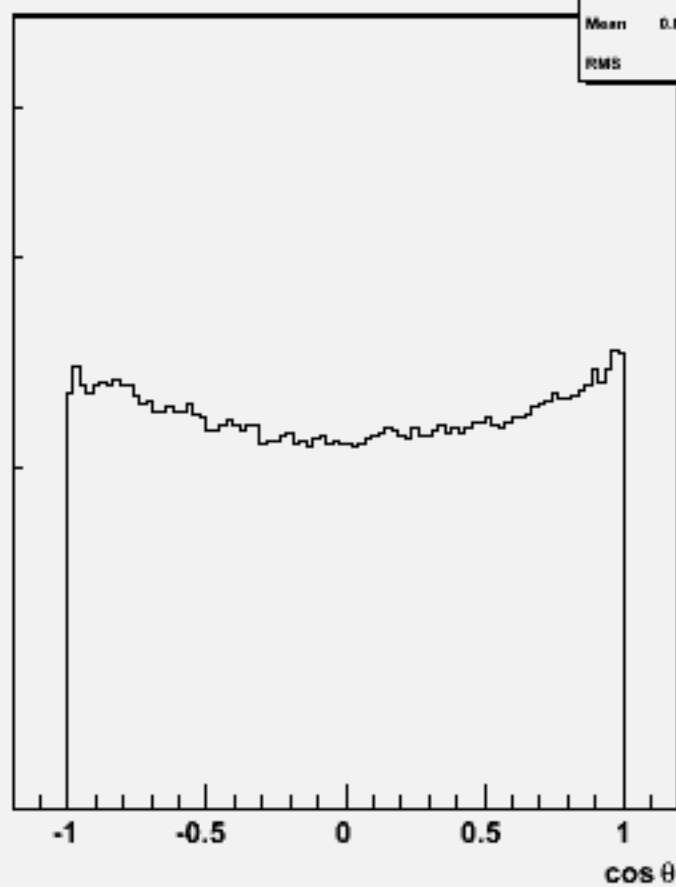
Particle cosθ : 106451 physsim-tth-6q-hbb
