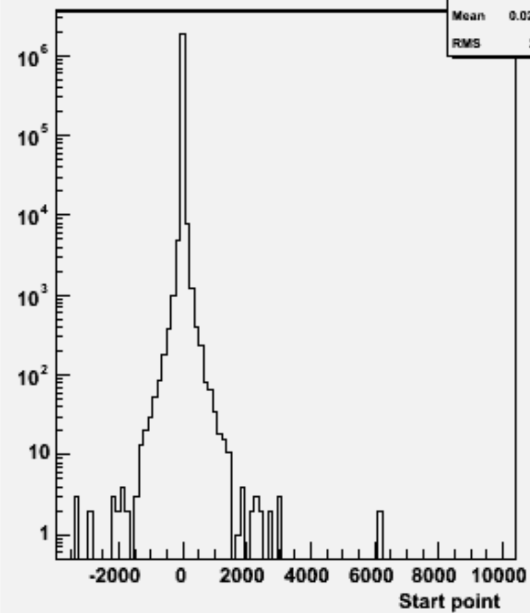
Start point Z : 106451 physsim-tth-6q-hbb
