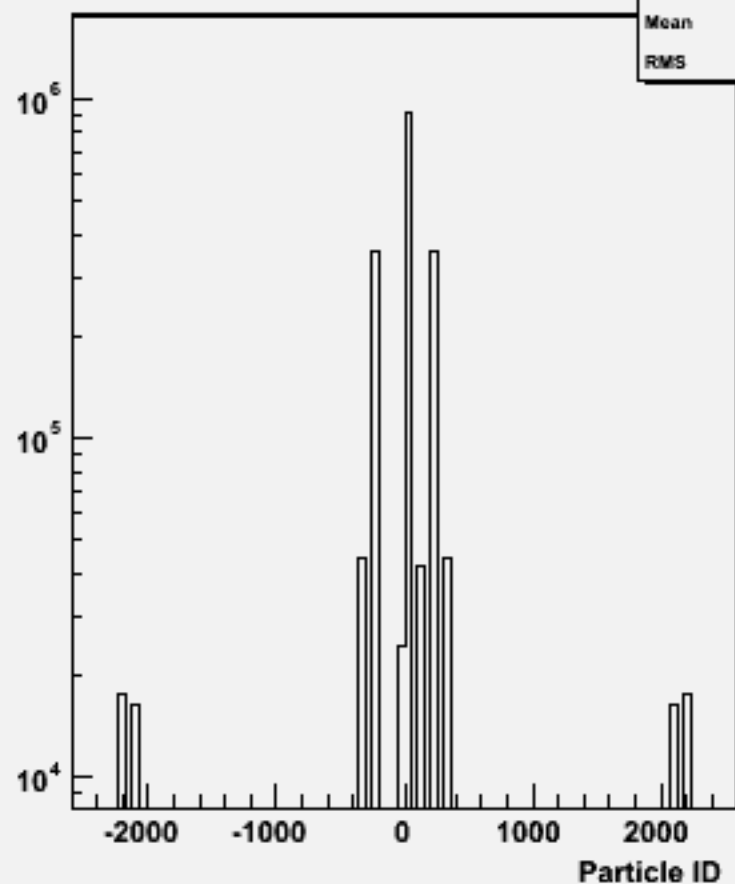
Particle ID : 106451 physsim-tth-6q-hbb
