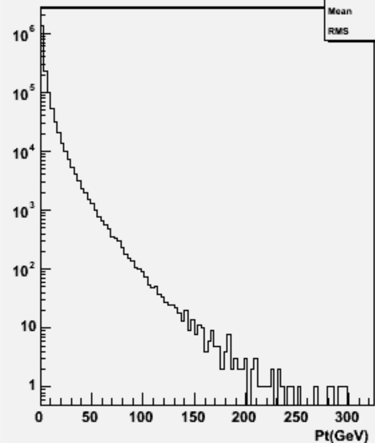
Particle Pt : 106451 physsim-tth-6q-hbb
