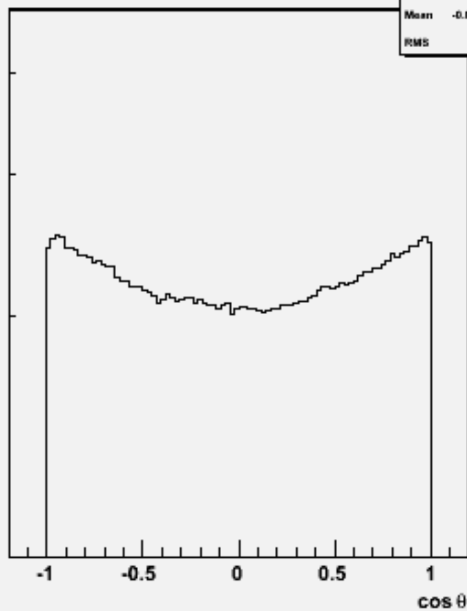
Particle cosθ : 106405 physsim-ttbb-6q-all
