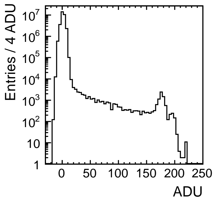
Figure 6: FPCCD response when irradiated with \text{Fe}^{55} . The two peaks in the range [150, 200] correspond with emissions of photons at energies 5.899 KeV and 6.490 keV.
